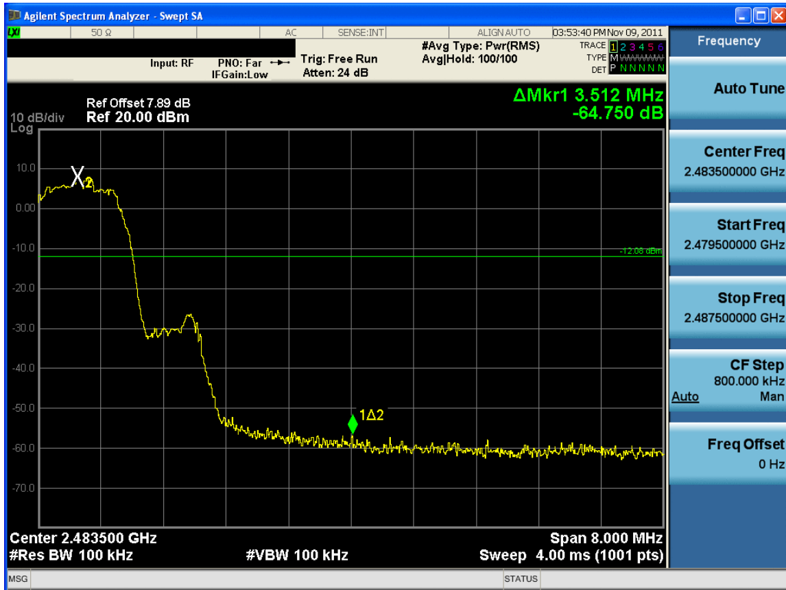
Plot 6-11. Band Edge Plot (Bluetooth, 3Mbps – Ch. 78)
