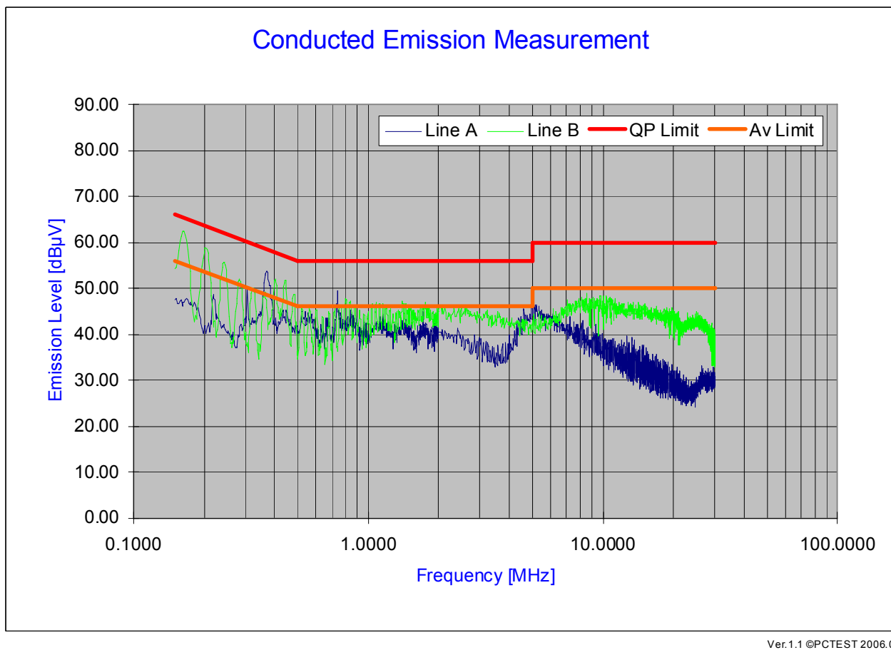
Plot 6-23. Line Conducted Plot with 802.11b
