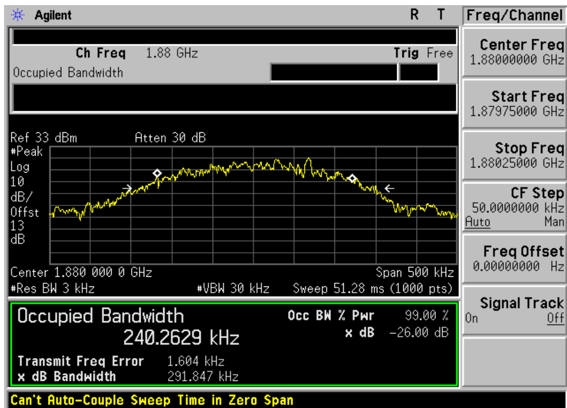
Plot 7-15. Occupied Bandwidth Plot (PCS GSM Mode – Ch.
