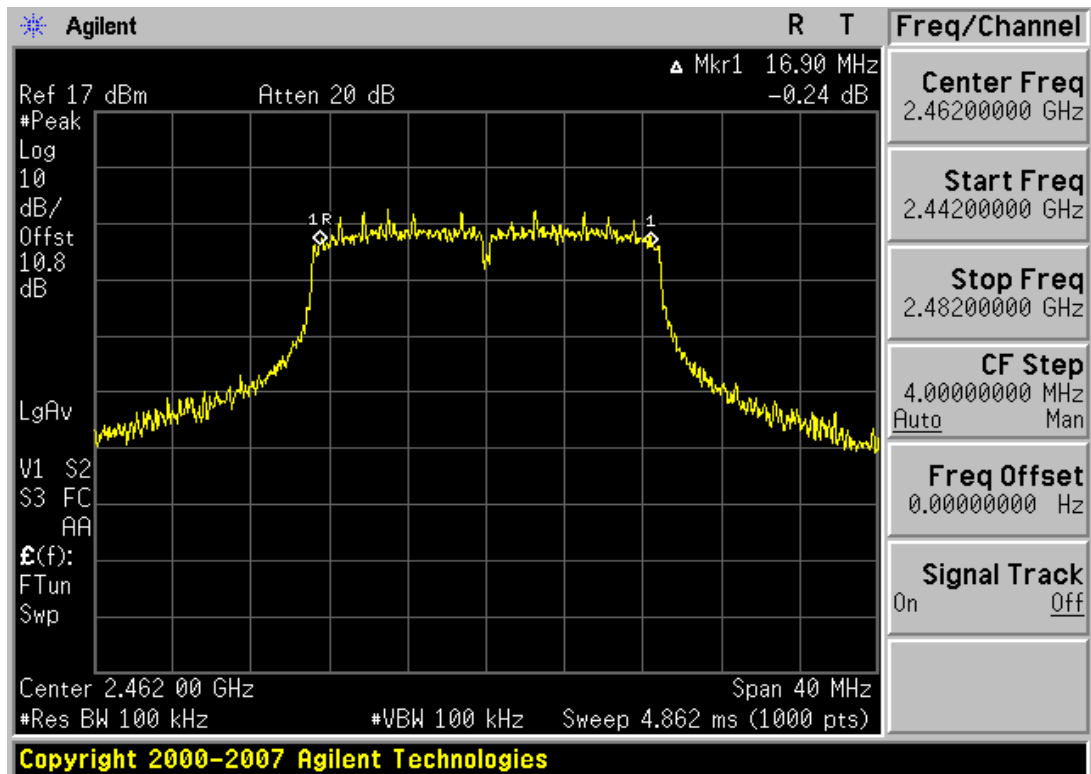
Plot 6-9. 6dB Bandwidth Plot (802.11n – Ch. 11)
