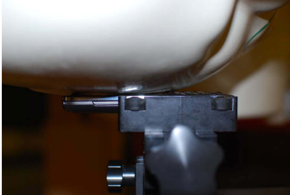
Figure 21-1 SAR Test Setup Photo 1
