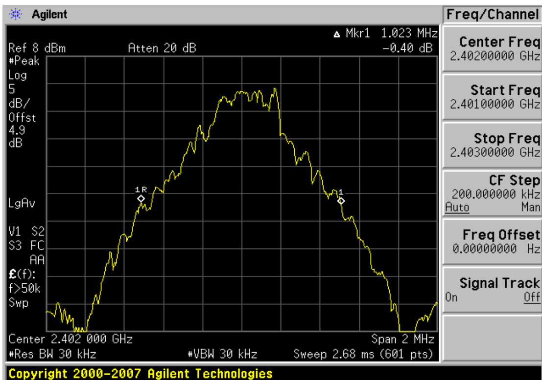
Plot 6-1. 20dB Bandwidth Plot (Bluetooth, 1Mbps – Ch. 0)
