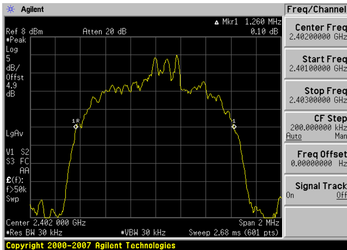
Plot 6-7. 20dB Bandwidth Plot (Bluetooth, 3Mbps – Ch. 0)
