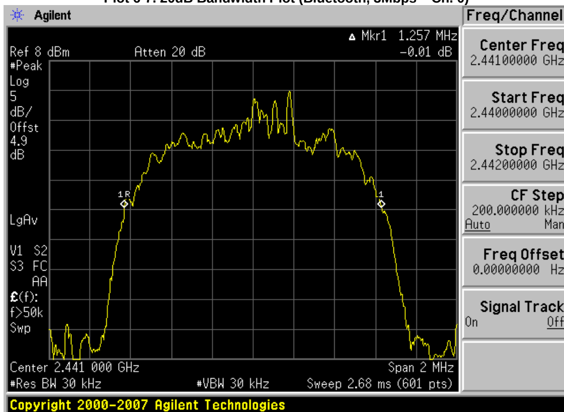
Plot 6-8. 20dB Bandwidth Plot (Bluetooth, 3Mbps – Ch. 39)
