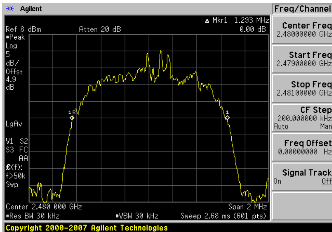
Plot 6-9. 20dB Bandwidth Plot (Bluetooth, 3Mbps – Ch. 78)
