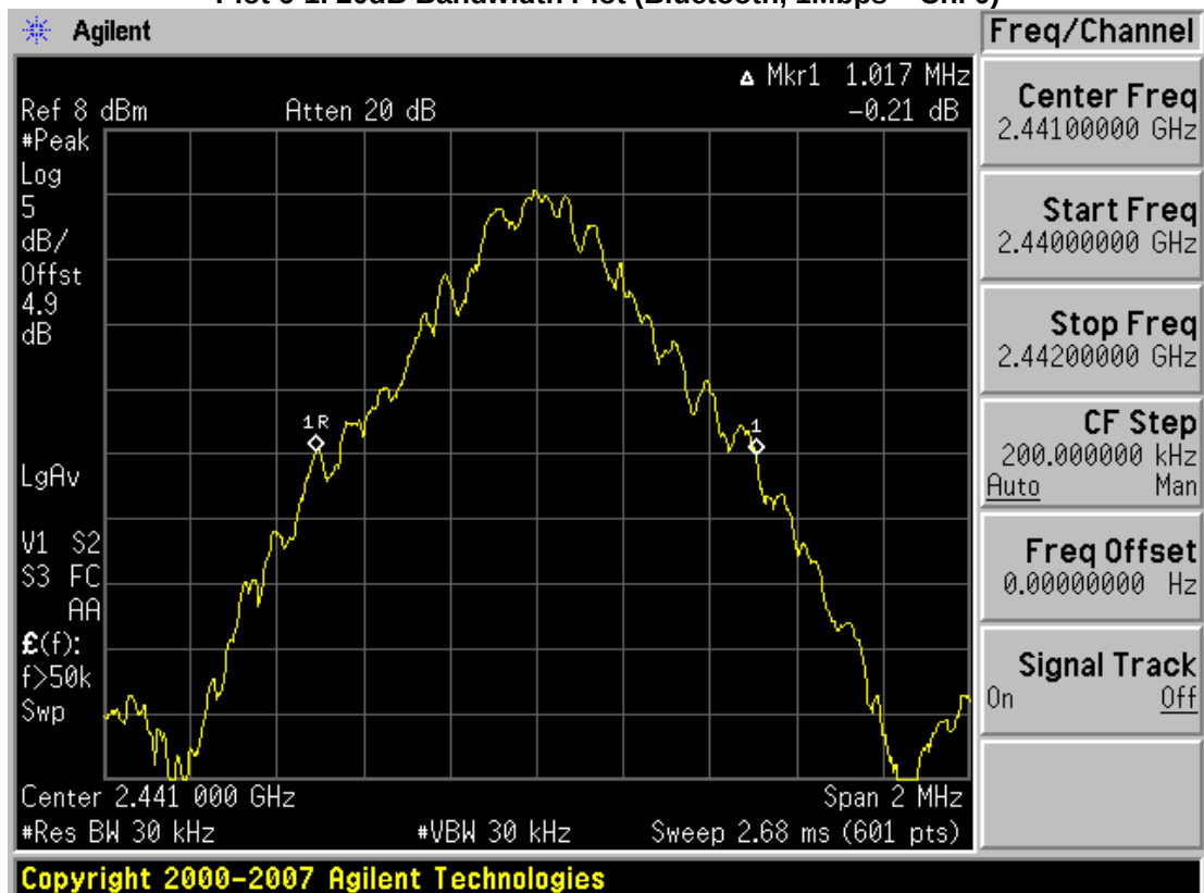
Plot 6-2. 20dB Bandwidth Plot (Bluetooth, 1Mbps – Ch. 39)
