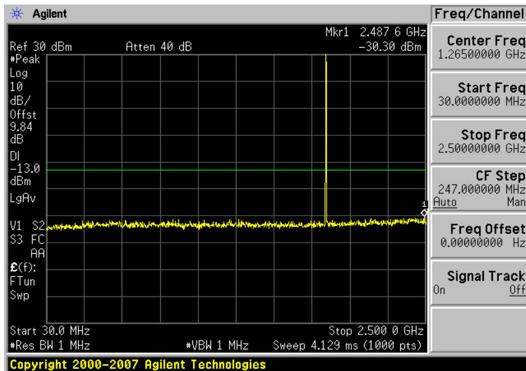
Plot 7-1. Conducted Spurious Plot (PCS GSM Mode (Main Ant.) – Ch. 512)
