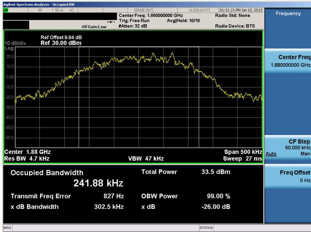
Plot 8-11. Occupied Bandwidth Plot (EDGE1900 Mode (Aux. Ant.) – Ch. 661)
