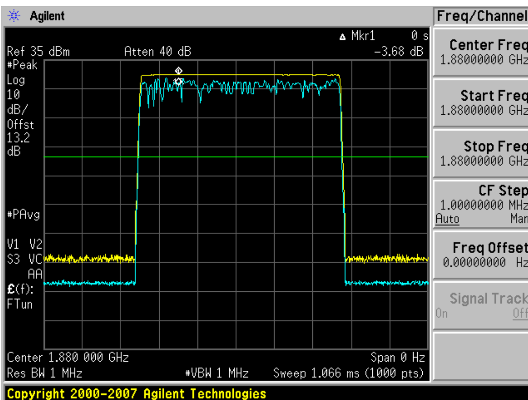
Plot 7-12. Peak-Average Ratio Plot (EDGE1900 Mode (Main Ant.) – Ch. 661)
