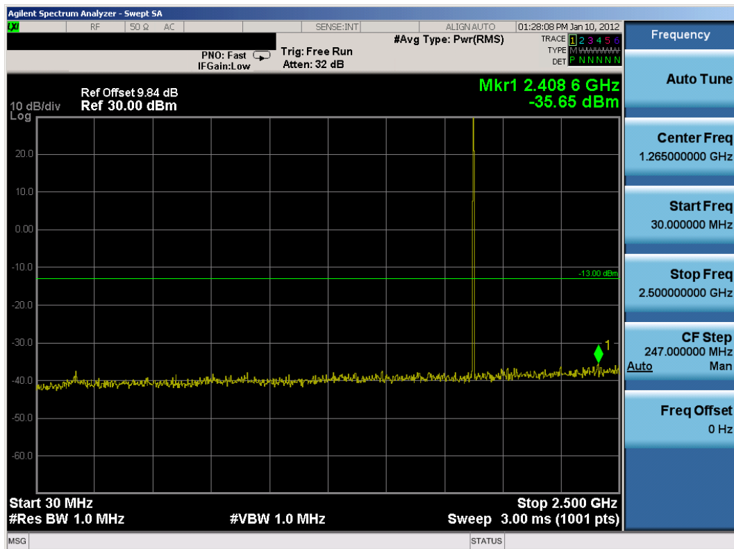
Plot 8-4. Conducted Spurious Plot (PCS GSM Mode (Aux. Ant.) – Ch. 661)
