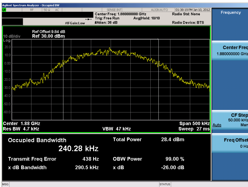
Plot 8-6. Occupied Bandwidth Plot (PCS GSM Mode (Aux. Ant.) – Ch. 661)
