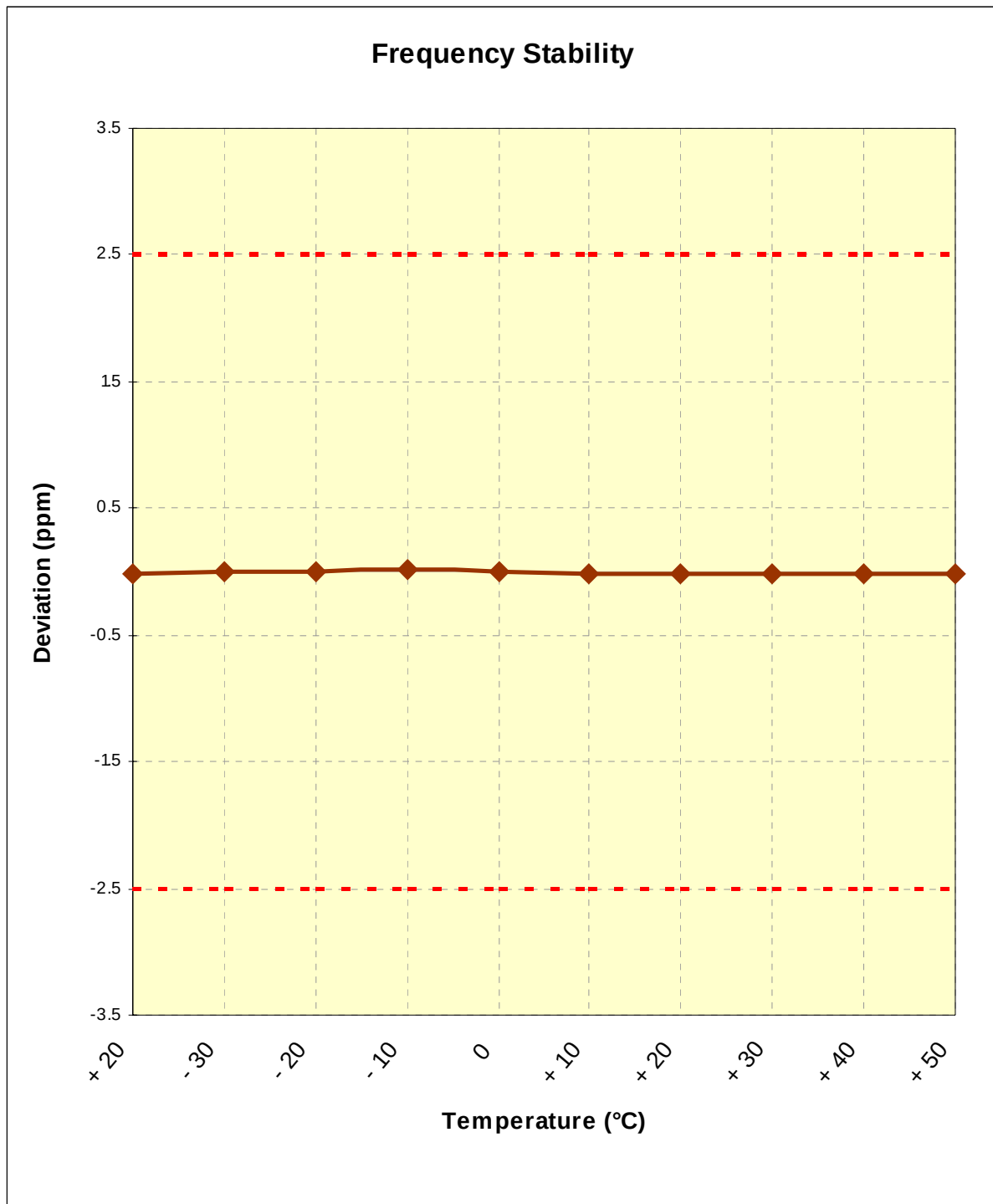
Plot 6-1. Frequency Stability Graph (PCS GSM Mode (Main Ant.) – Ch. 661)
