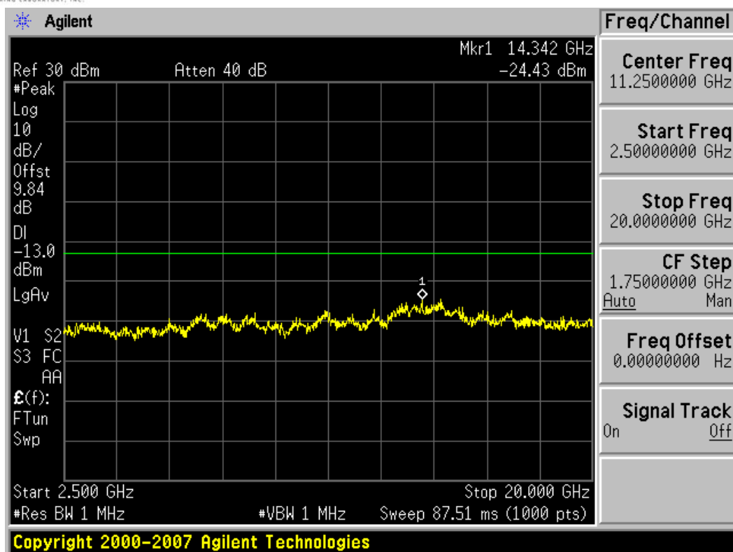
Plot 7-9. Conducted Spurious Plot (PCS GSM Mode (Main Ant.) – Ch. 810)
