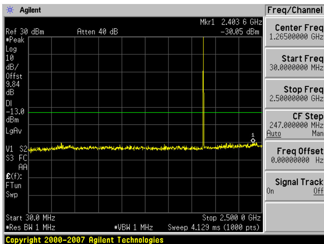
Plot 7-4. Conducted Spurious Plot (PCS GSM Mode (Main Ant.) – Ch. 661)
