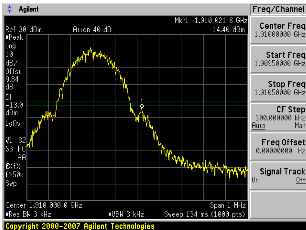
Plot 7-10. Band Edge Plot (PCS GSM Mode (Main Ant.) – Ch. 810)
