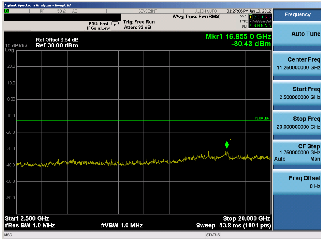
Plot 8-5. Conducted Spurious Plot (PCS GSM Mode (Aux. Ant.) – Ch. 661)
