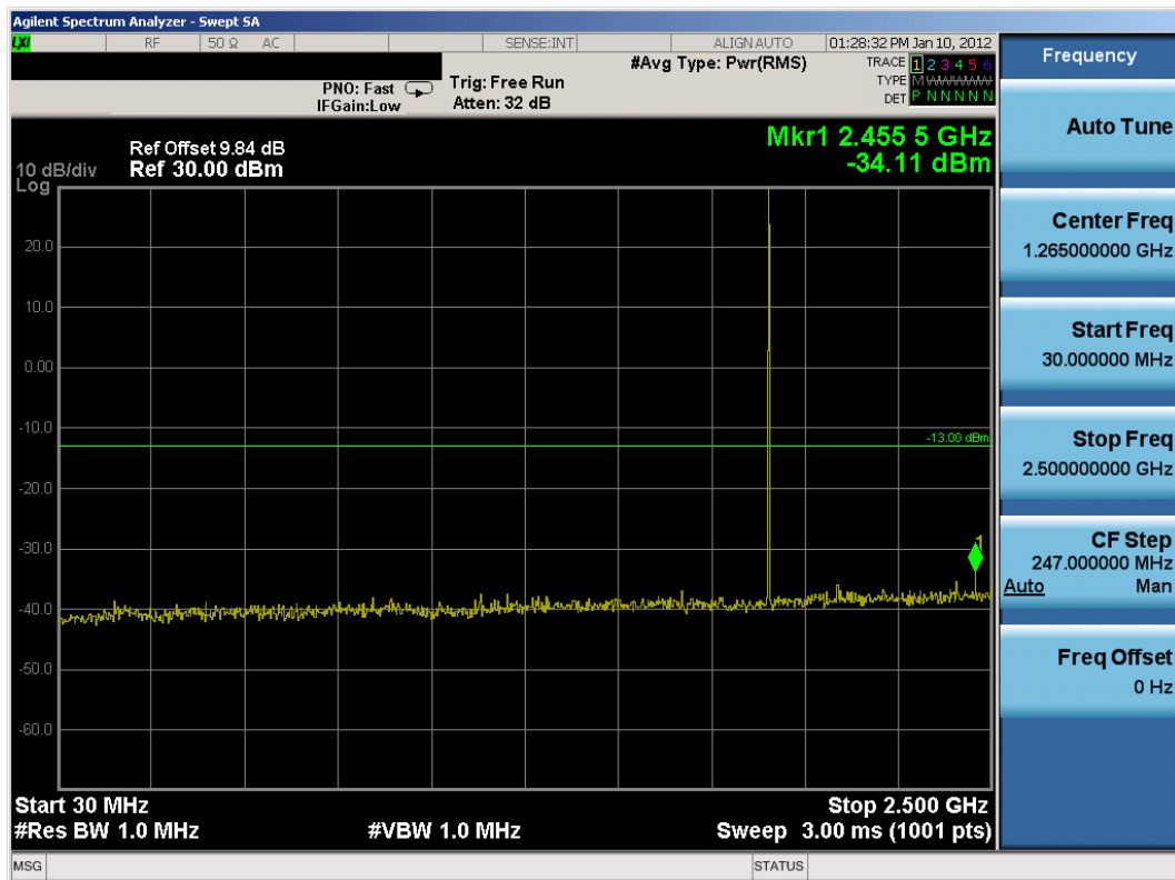
Plot 8-8. Conducted Spurious Plot (PCS GSM Mode (Aux. Ant.) - Ch. 810)
