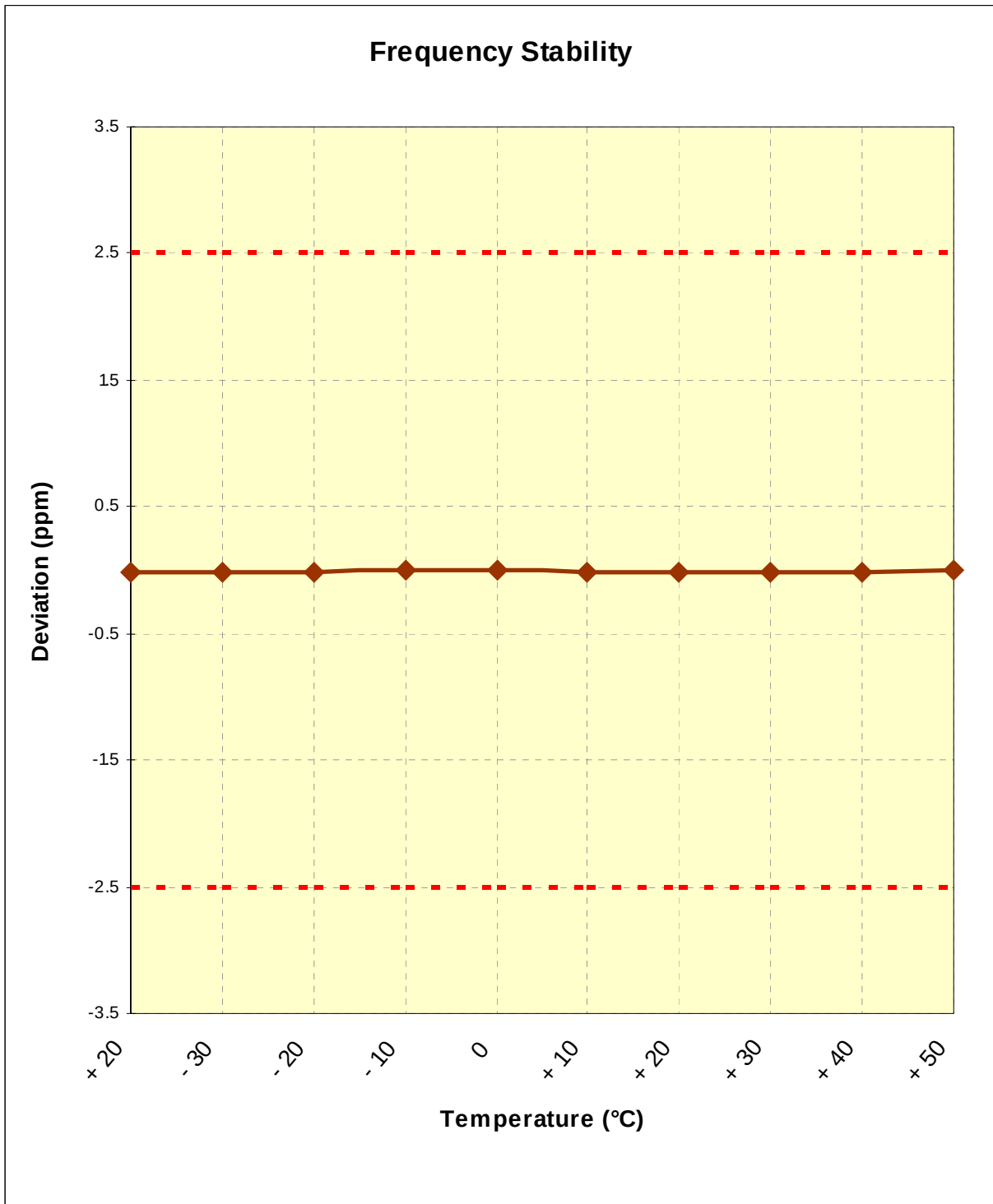
Plot 6-2. Frequency Stability Graph (PCS GSM Mode (Aux. Ant.) – Ch. 661)
