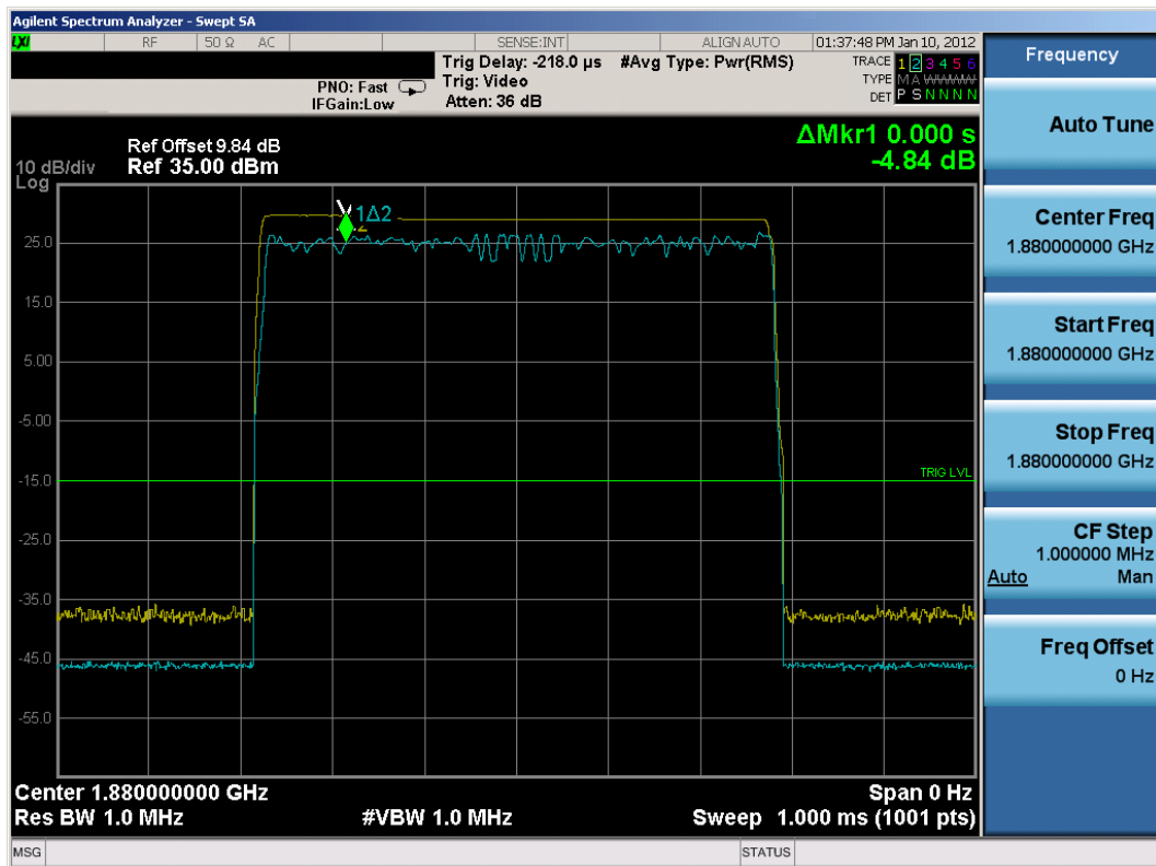
Plot 8-12. Peak-Average Ratio Plot (EDGE1900 Mode (Aux. Ant.) – Ch. 661)
