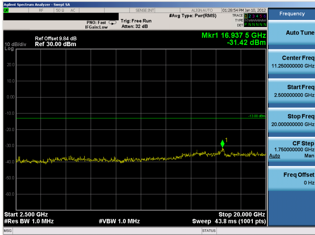
Plot 8-9. Conducted Spurious Plot (PCS GSM Mode (Aux. Ant.) – Ch. 810)
