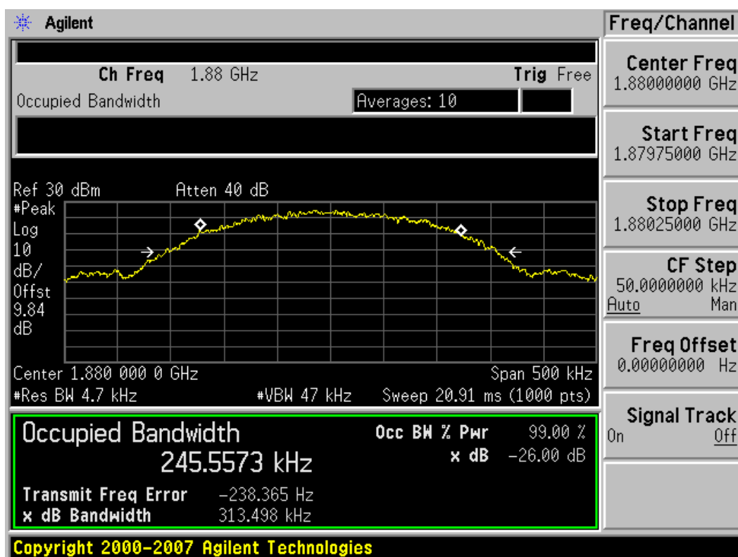
Plot 7-6. Occupied Bandwidth Plot (PCS GSM Mode (Main Ant.) – Ch. 661)
