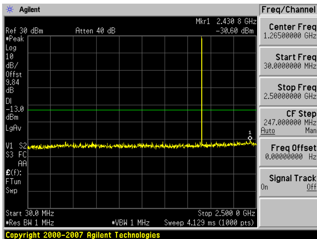
Plot 7-8. Conducted Spurious Plot (PCS GSM Mode (Main Ant.) – Ch. 810)
