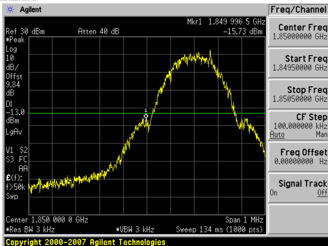
Plot 7-3. Band Edge Plot (PCS GSM Mode (Main Ant.) – Ch. 512)
