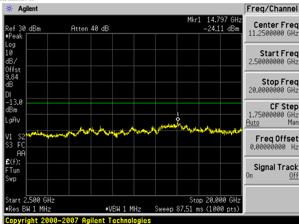
Plot 7-5. Conducted Spurious Plot (PCS GSM Mode (Main Ant.) – Ch. 661)
