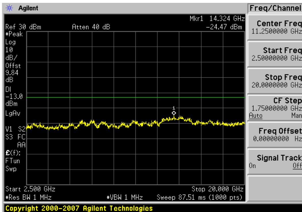
Plot 7-2. Conducted Spurious Plot (PCS GSM Mode (Main Ant.) – Ch. 512)
