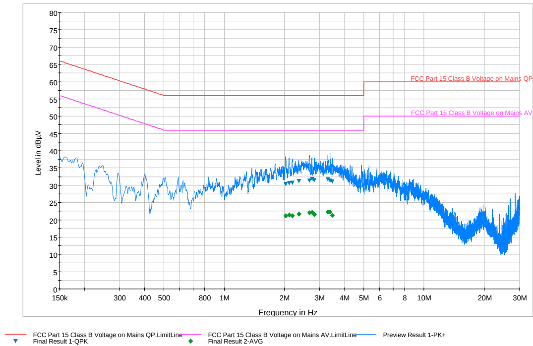
Plot 6-24. Line-Conducted Test Plot (L1)
