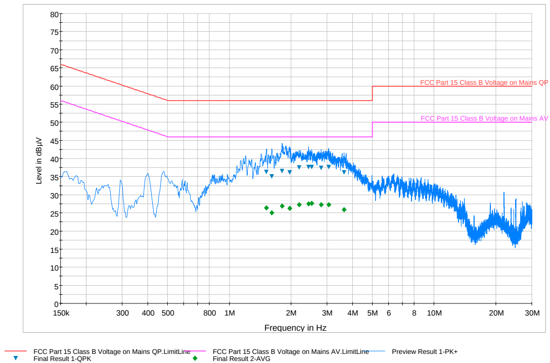
Plot 6-25. Line-Conducted Test Plot (N)
