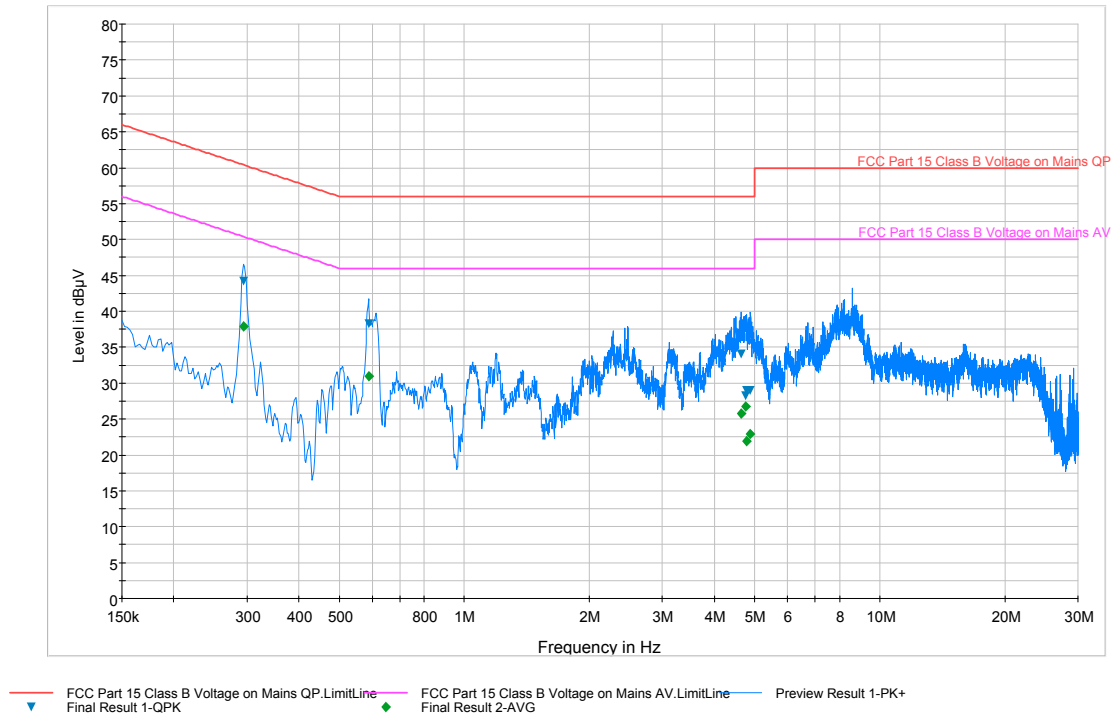
Plot 6-45. Line-Conducted Test Plot (N)
