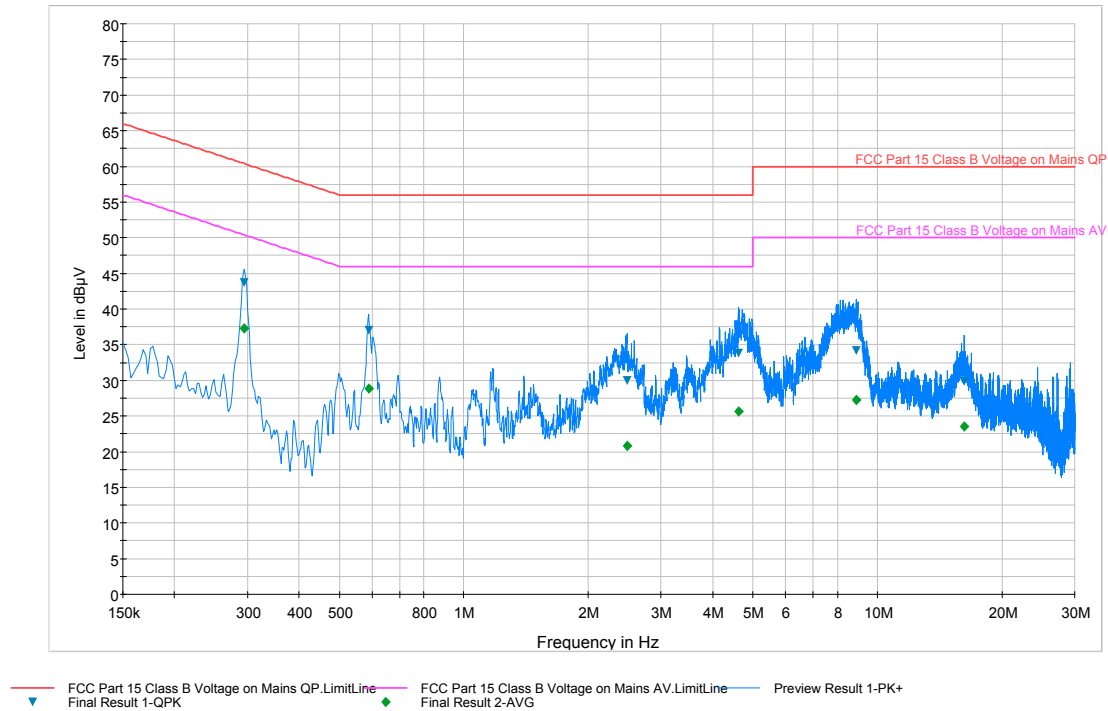
Plot 6-44. Line-Conducted Test Plot (L1)
