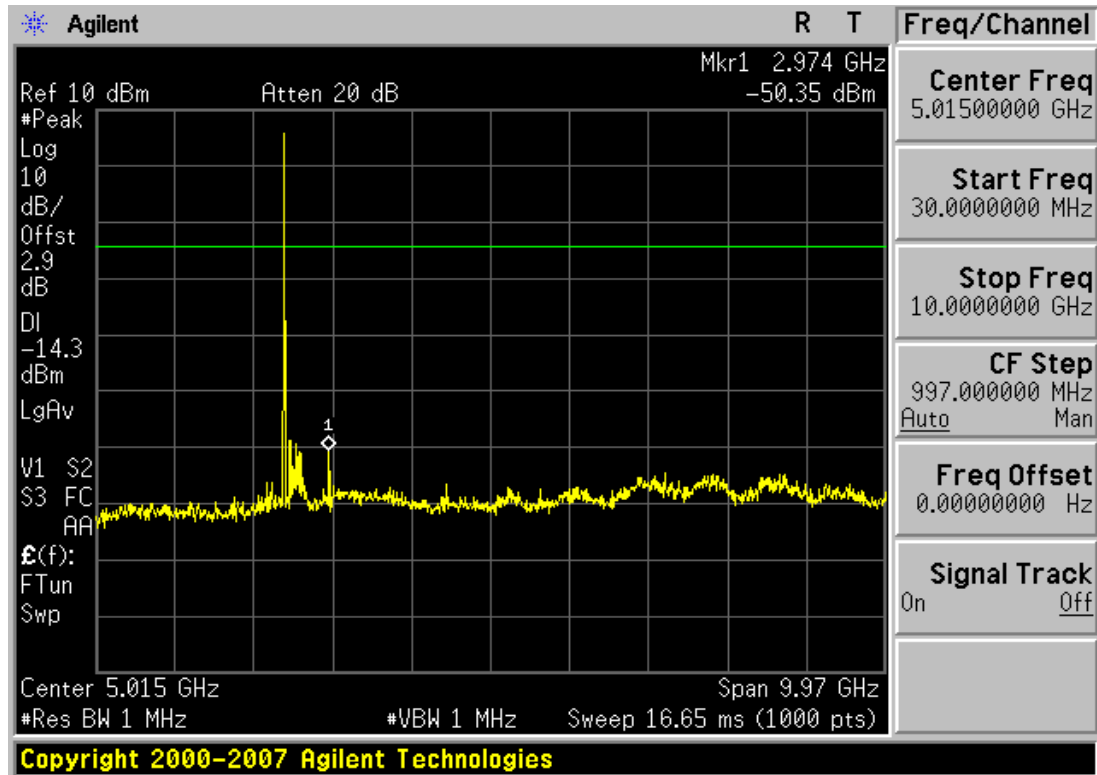
Plot 6-18. Conducted Spurious Plot (Bluetooth, 1Mbps – Ch. 0)
