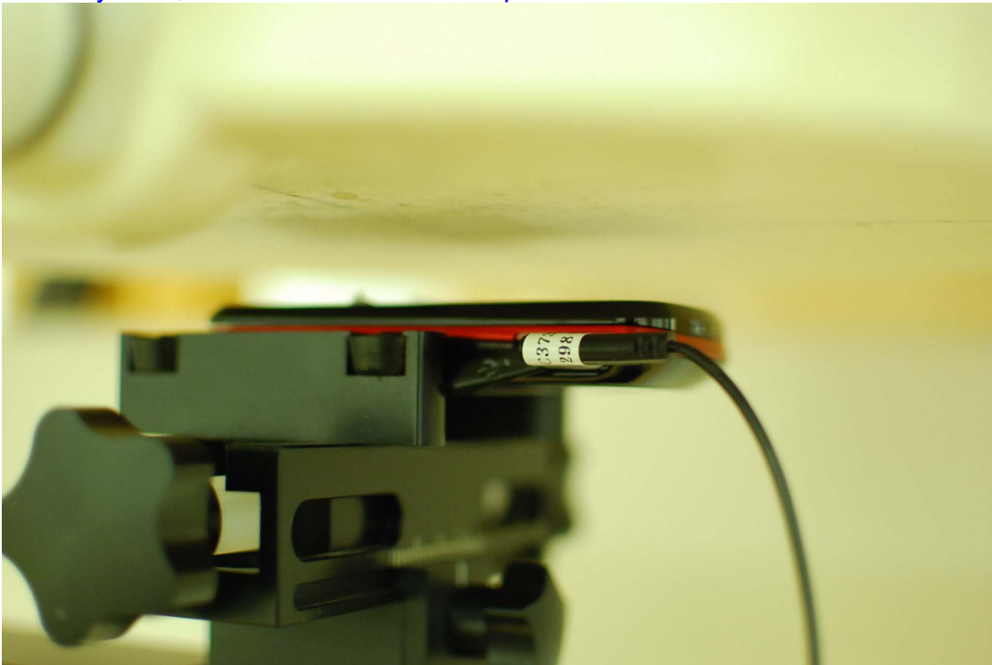
14. Body SAR, Front Side with 1.5 cm Space
