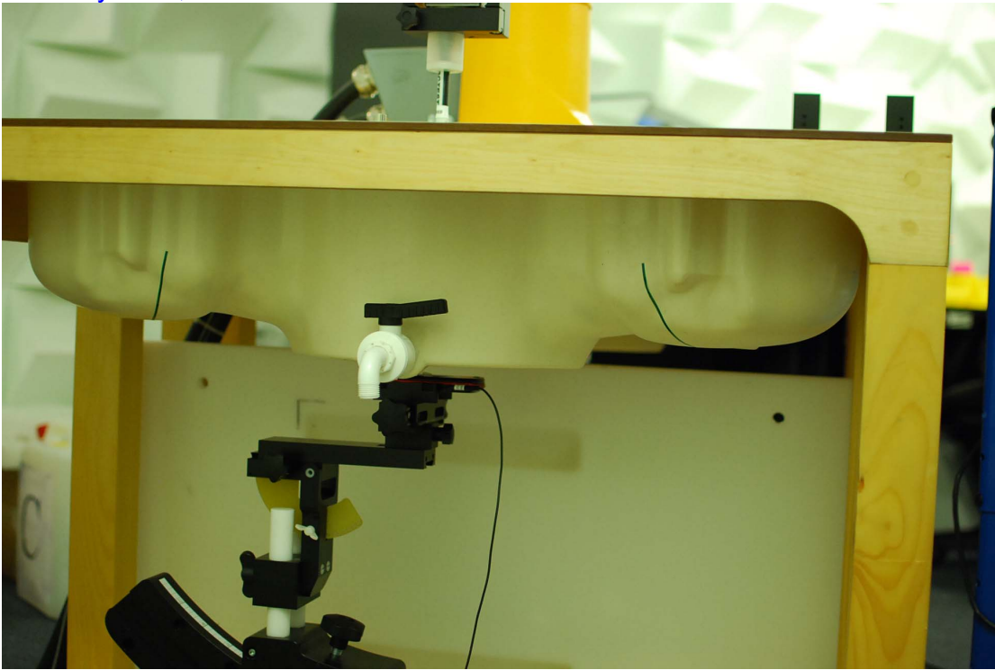
13. Body SAR, Front Side
