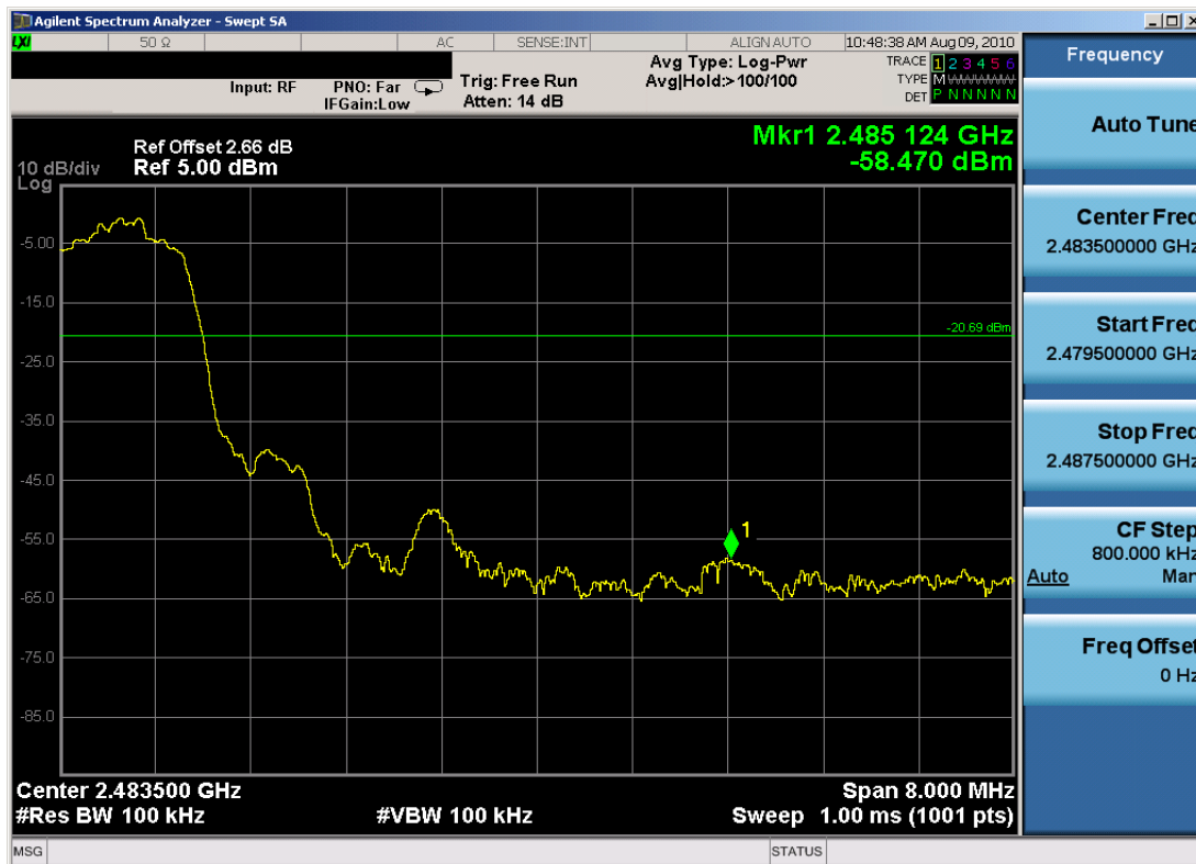
Plot 6-7. Band Edge Plot (Bluetooth (EDR) - Ch. 78)
