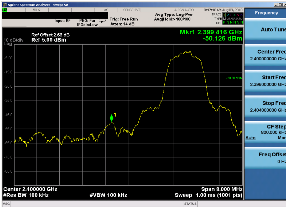
Plot 6-6. Band Edge Plot (Bluetooth (EDR) - Ch. 0)
