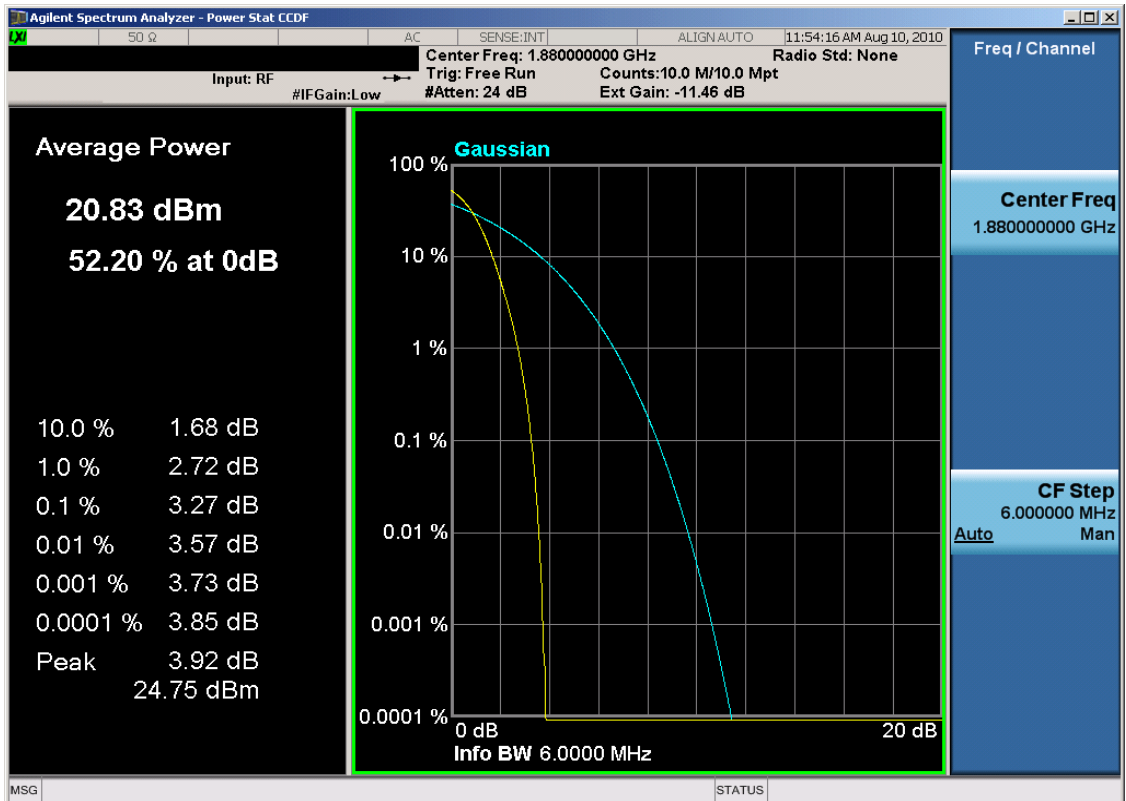
Plot 7-38. Peak-Average Ratio Plot (PCS WCDMA Mode – Ch. 9400)
