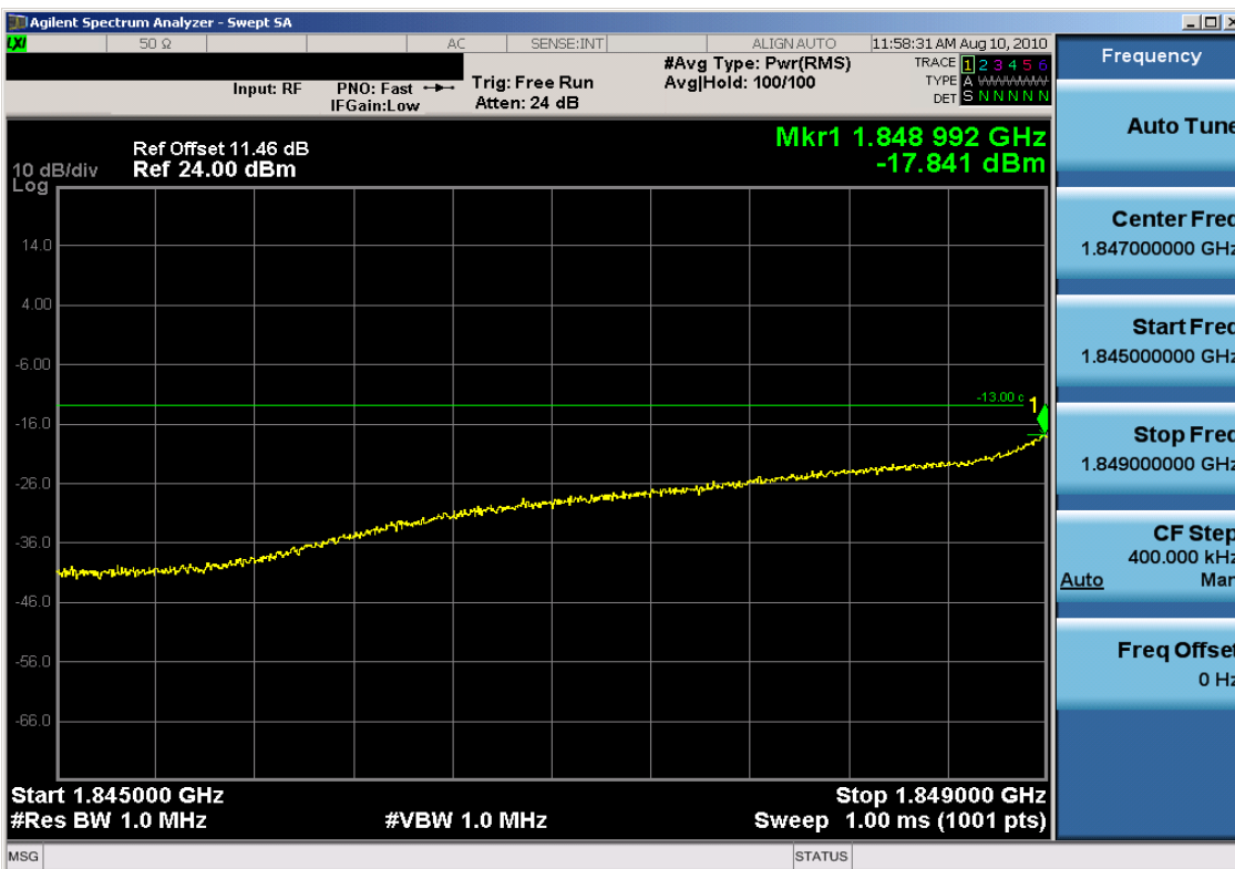
Plot 7-34. 4MHz Span Plot (PCS WCDMA Mode – Ch. 9262)
