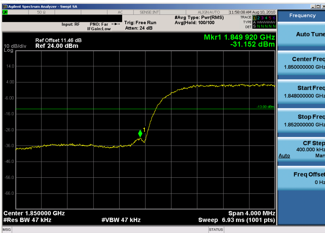
Plot 7-33. Band Edge Plot (PCS WCDMA Mode – Ch. 9262)
