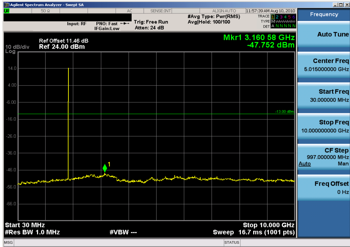
Plot 7-31. Conducted Spurious Plot (PCS WCDMA Mode – Ch. 9262)
