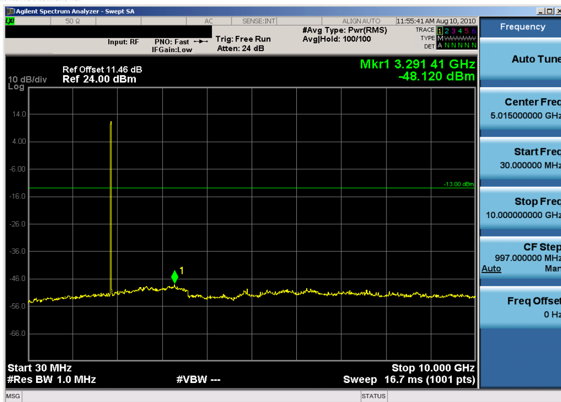
Plot 7-35. Conducted Spurious Plot (PCS WCDMA Mode – Ch. 9400)
