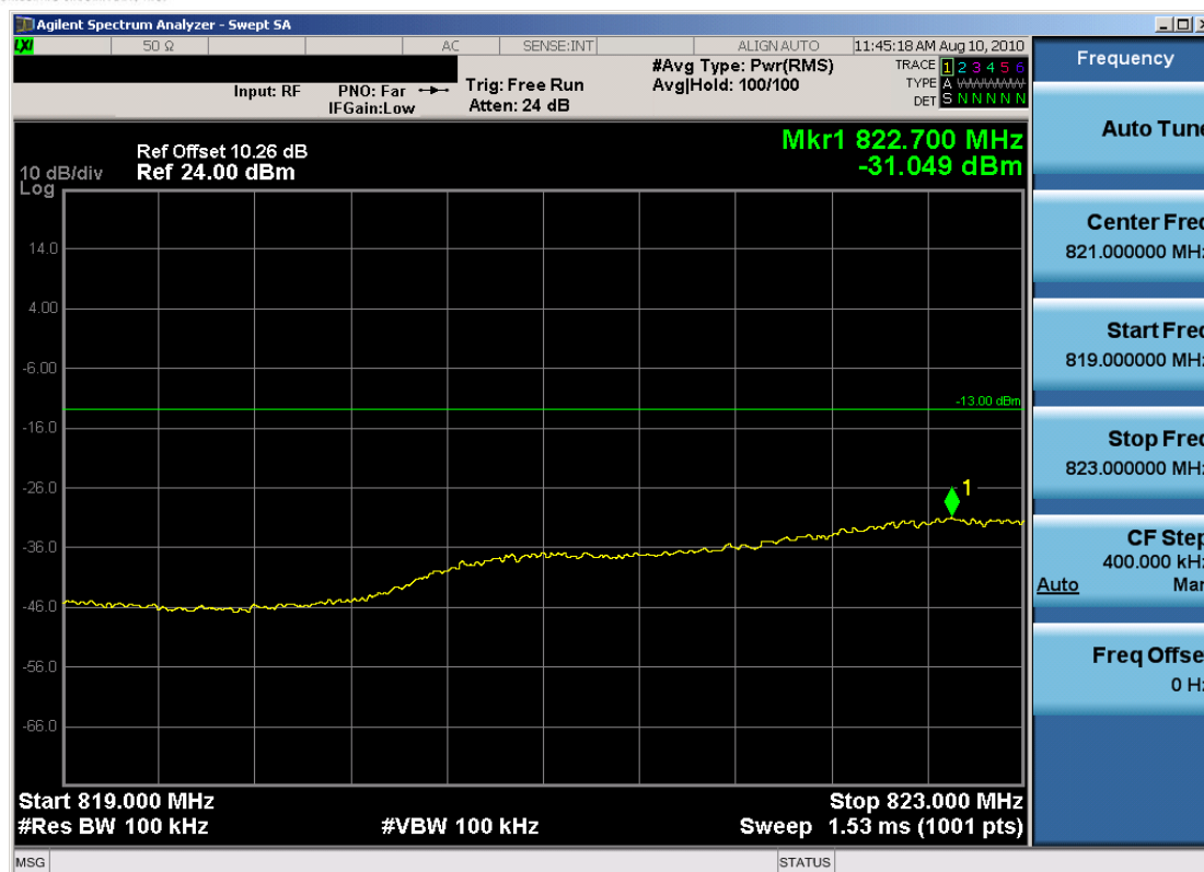
Plot 7-23. 4MHz Span Plot (Cellular WCDMA Mode – Ch. 4132)
