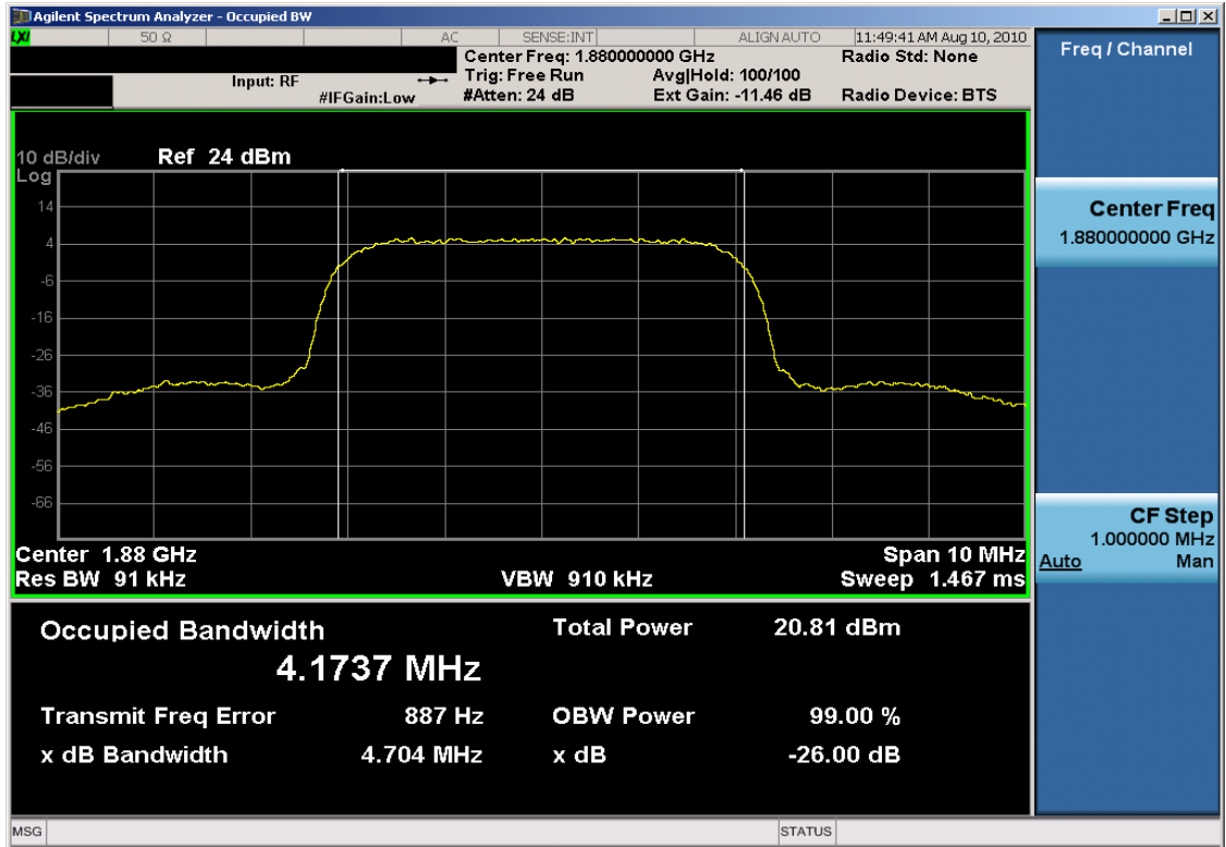
Plot 7-37. Occupied Bandwidth Plot (PCS WCDMA Mode – Ch. 9400)
