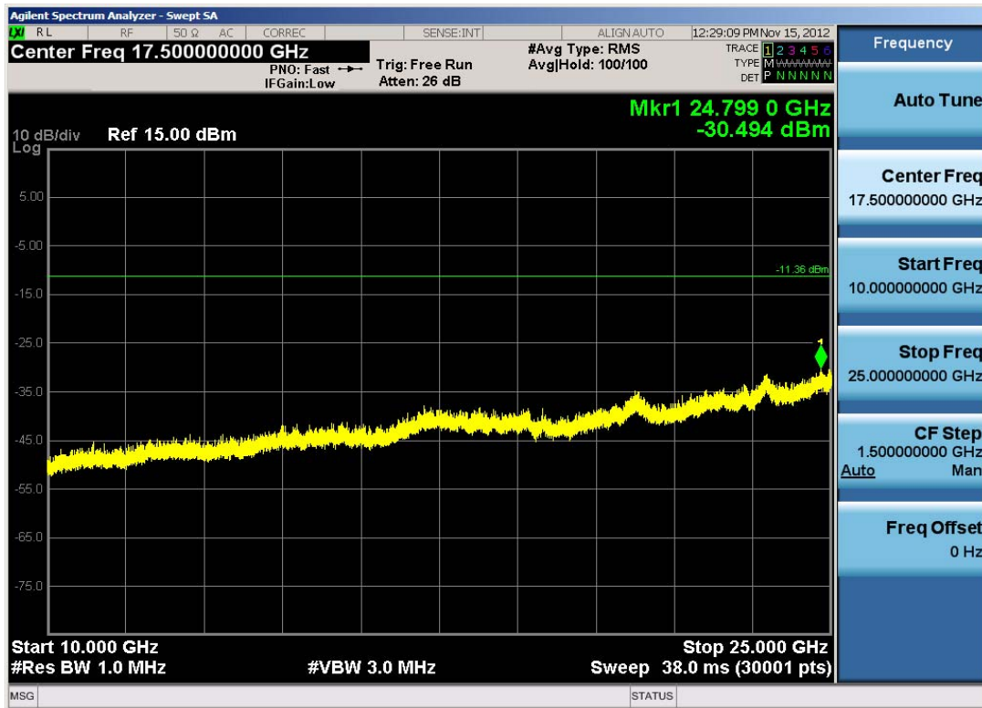
Plot 6-39. Conducted Spurious Plot (Bluetooth, 1Mbps – Ch. 39)
