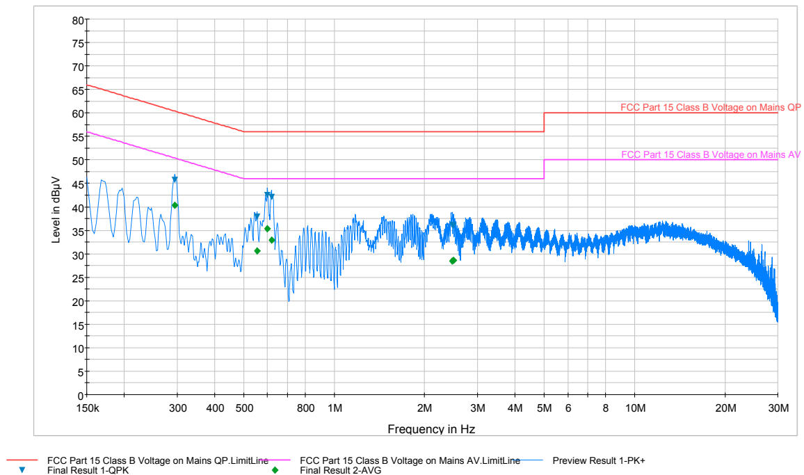
Plot 6-43. Line-Conducted Test Plot (N)
