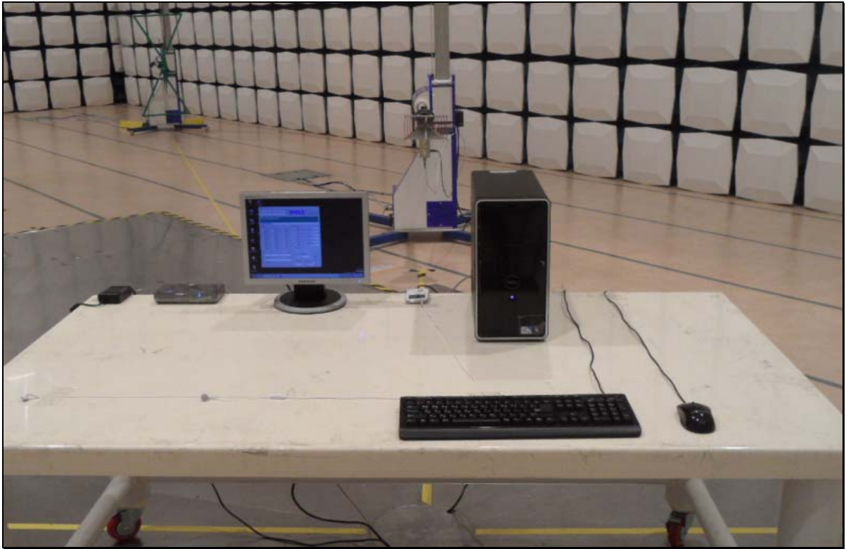
[ Radiated Disturbance for Above 1 GHz – Front ]
