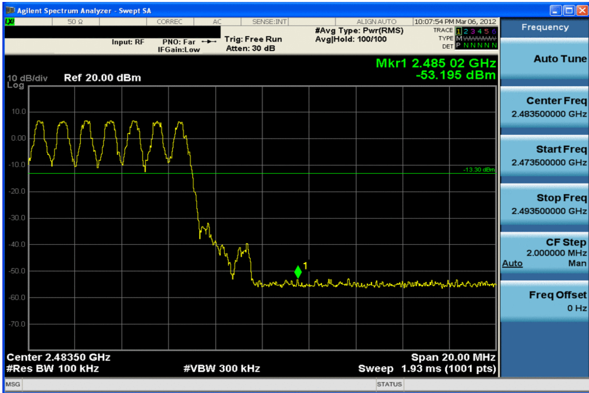
Plot 6-13. Band Edge Plot (Bluetooth with Hopping Enabled, 1Mbps – Ch. 78)
