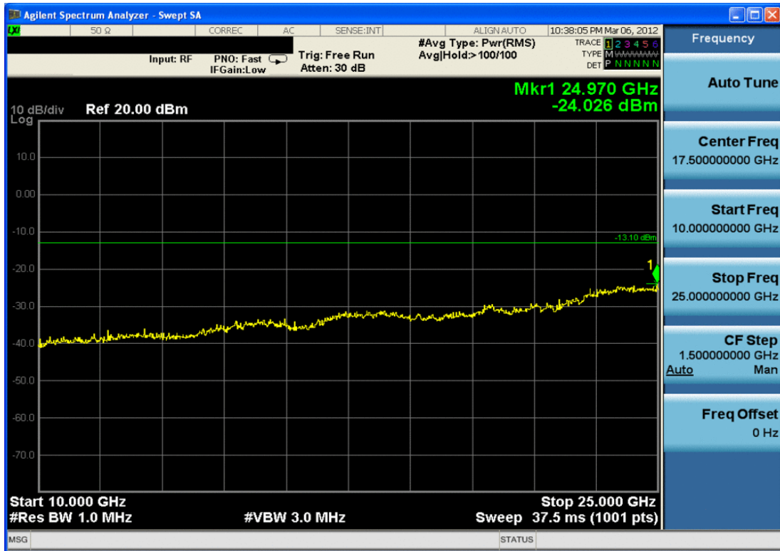
Plot 6-19. Conducted Spurious Plot (Bluetooth, 1Mbps – Ch. 0)
