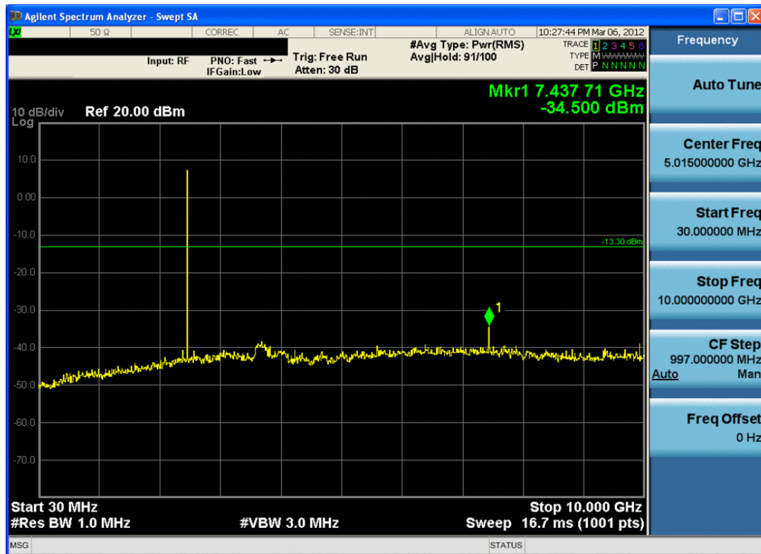
Plot 6-22. Conducted Spurious Plot (Bluetooth, 1Mbps – Ch. 78)
