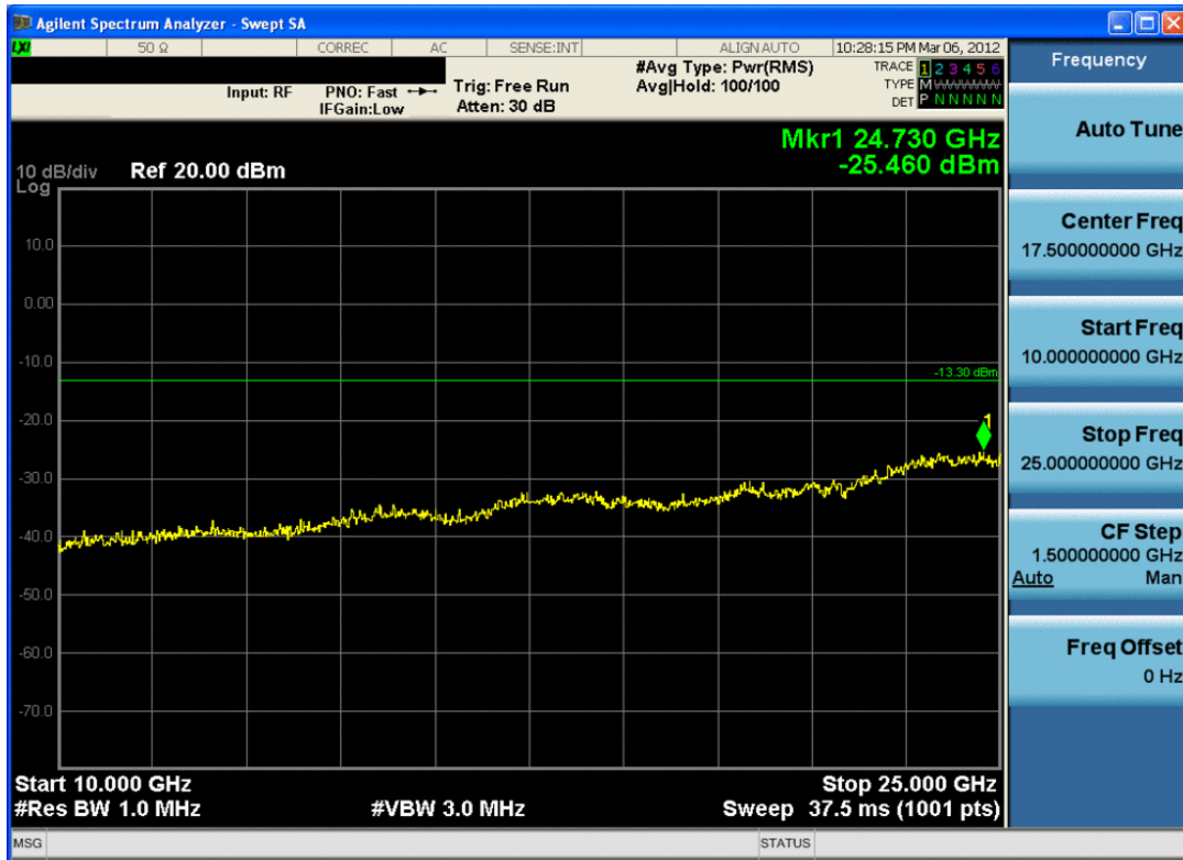
Plot 6-23. Conducted Spurious Plot (Bluetooth, 1Mbps – Ch. 78)
