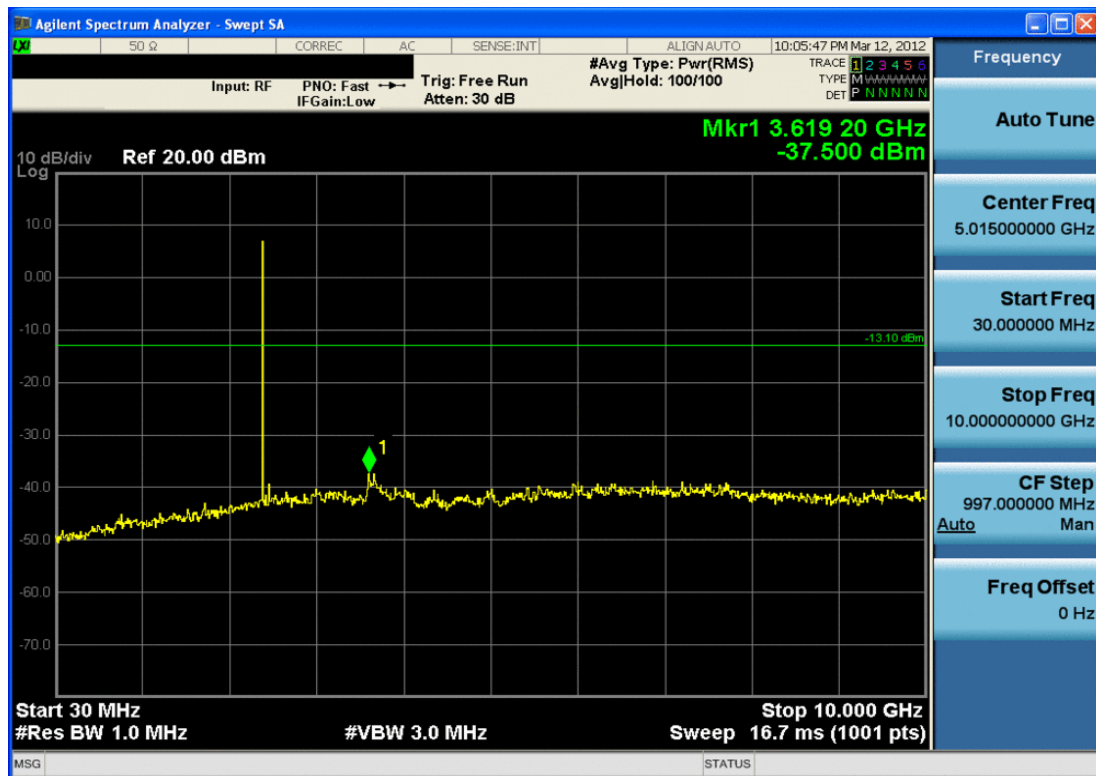
Plot 6-18. Conducted Spurious Plot (Bluetooth, 1Mbps – Ch. 0)
