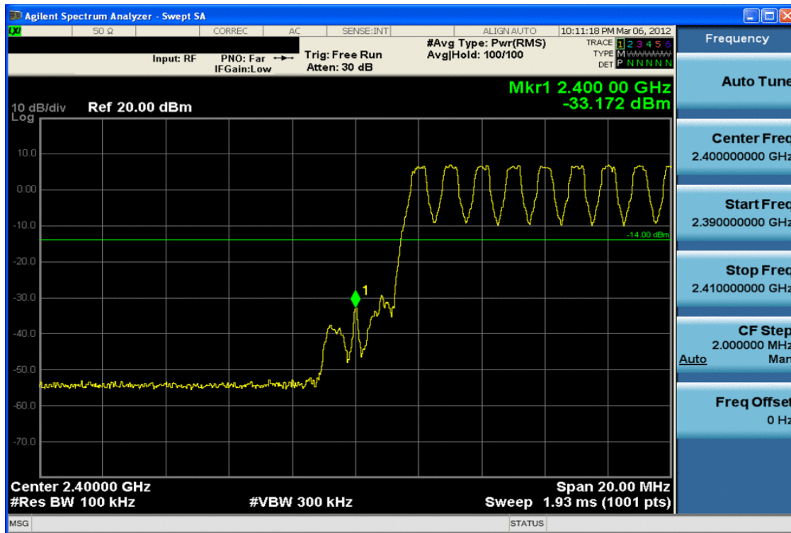
Plot 6-12. Band Edge Plot (Bluetooth with Hopping Enabled, 1Mbps – Ch. 0)
