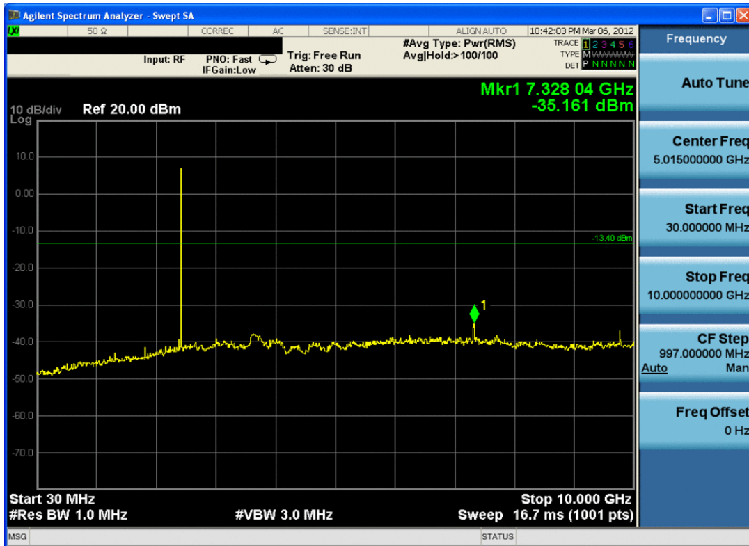
Plot 6-20. Conducted Spurious Plot (Bluetooth, 1Mbps – Ch. 39)
