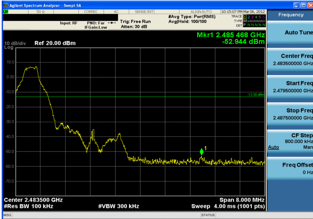
Plot 6-11. Band Edge Plot (Bluetooth with Hopping Disabled, 1Mbps – Ch. 78)
