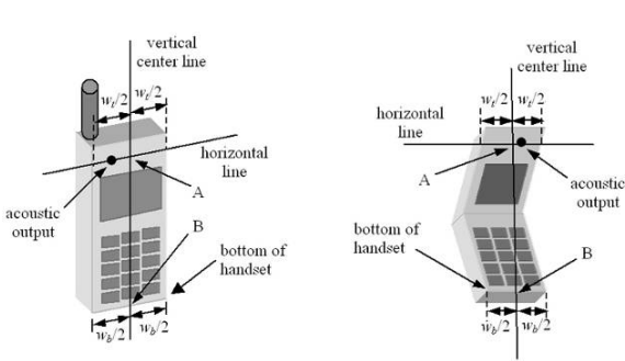
Figure 5.4 Handset vertical and horizontal reference lines
