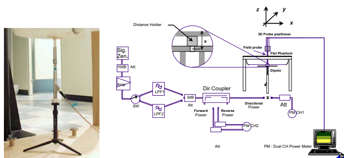
Figure 7.1 Dipole Validation Test Setup
