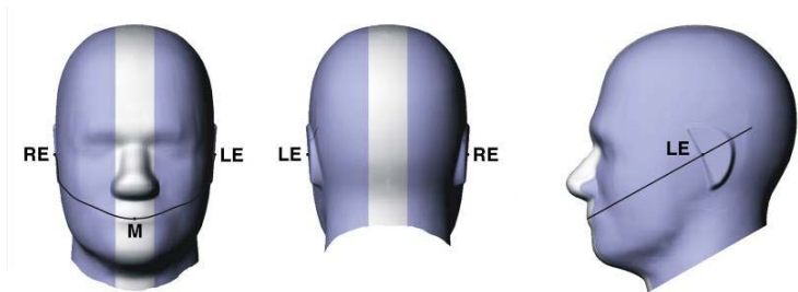
Figure 5.1 Front, back and side view of SAM
