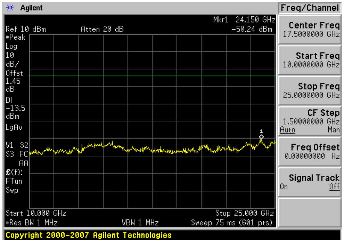
Plot 6-19. Conducted Spurious Plot (Bluetooth, 1Mbps - Ch. 0)
