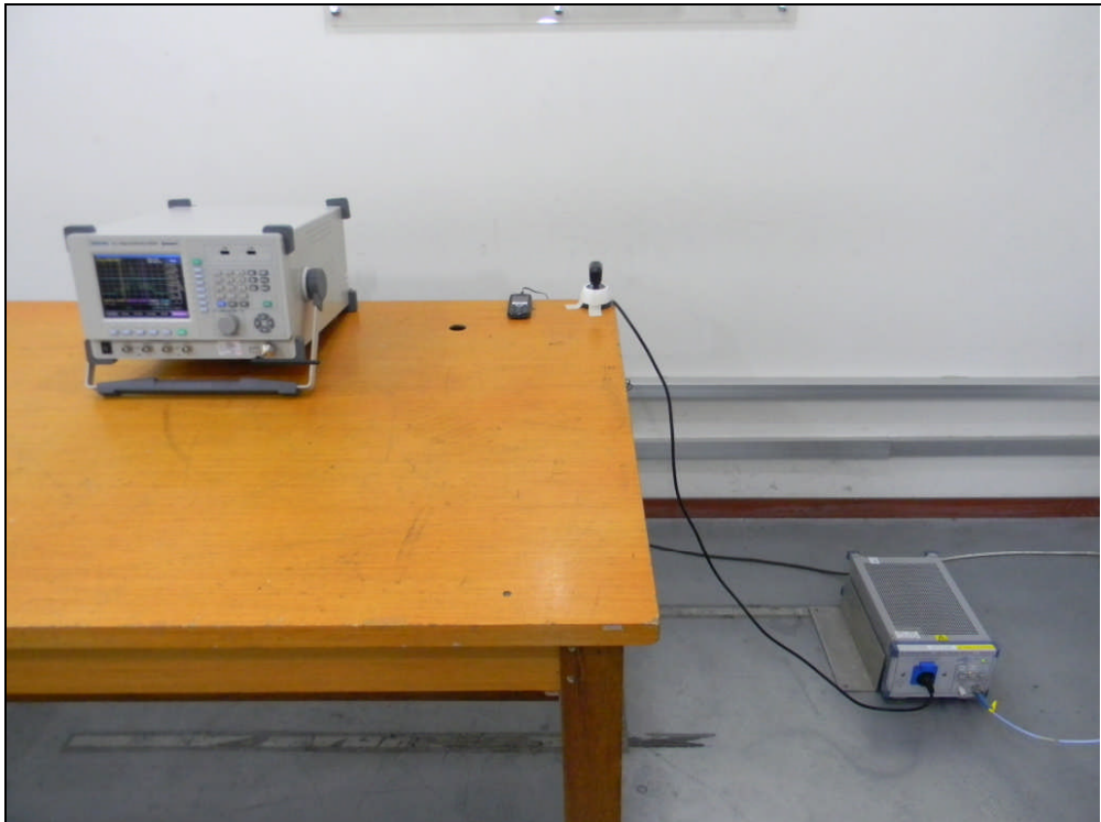
Photos of AC Power line conducted emission test.
