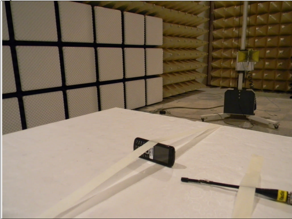
Photo of Spurious Emission Test
