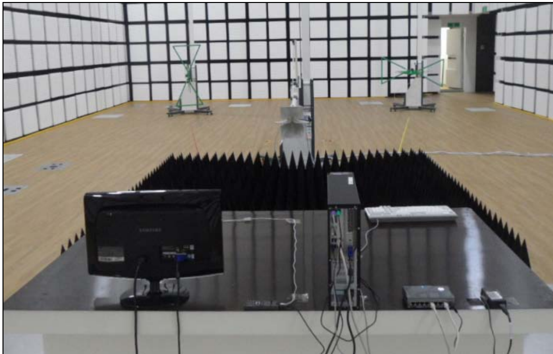
[ Radiated Disturbance for Above 1 GHz – Rear ]
