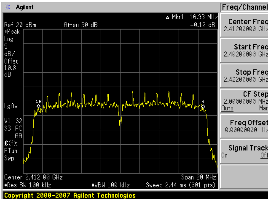
Plot 6-7. 6dB Bandwidth 19.5/21.7Mbps Data Rate Plot (802.11n – Ch. 1)
