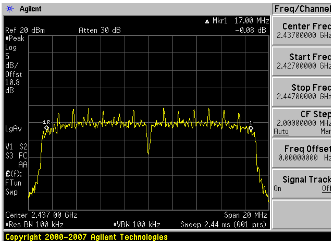
Plot 6-8. 6dB Bandwidth 19.5/21.7Mbps Data Rate Plot (802.11n – Ch. 6)
