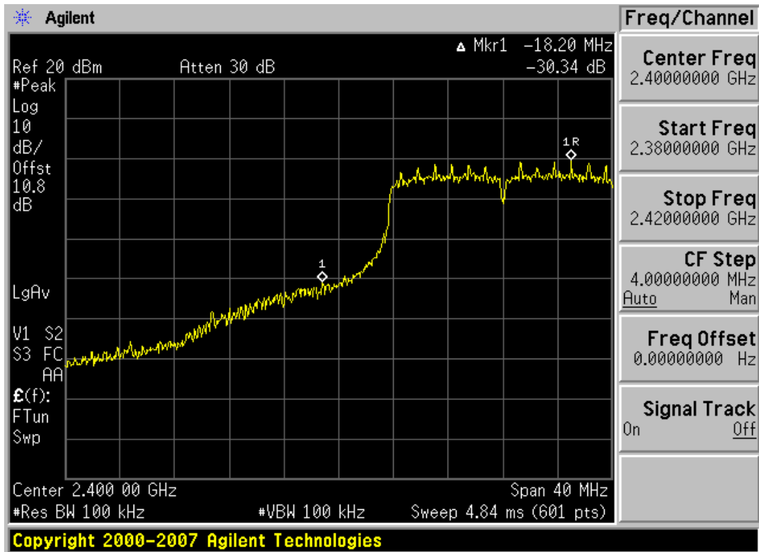
Plot 6-21. Band Edge 1Mbps Data Rate Plot (802.11g – Ch. 1)
