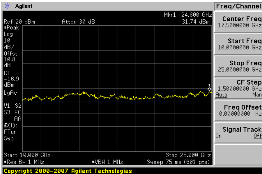
Plot 6-26. Conducted Spurious 1Mbps Data Rate Plot (802.11b – Ch. 1)
