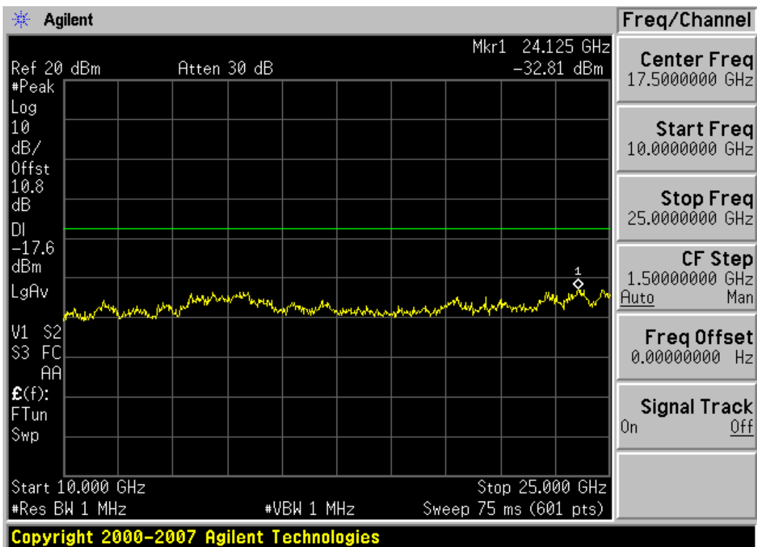
Plot 6-30. Conducted Spurious 1Mbps Data Rate Plot (802.11b – Ch. 11)
