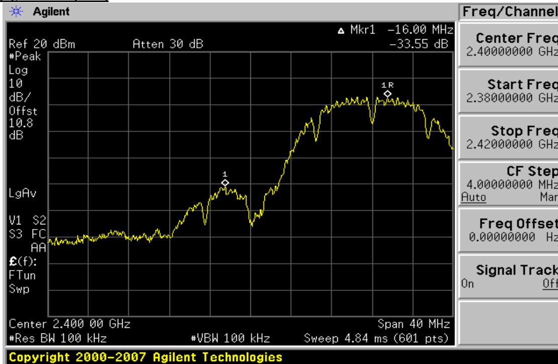
Plot 6-19. Band Edge 1Mbps Data Rate Plot (802.11b - Ch. 1)
