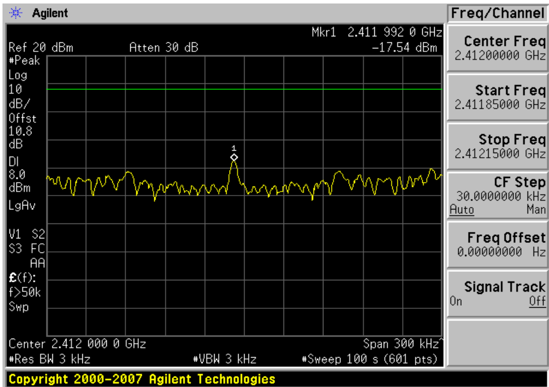
Plot 6-10. Power Spectral Density 1Mbps Data Rate Plot (802.11b – Ch. 1)
