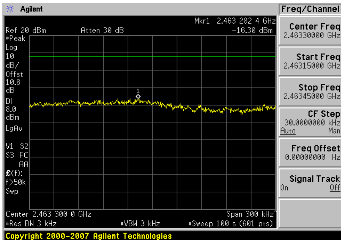
Plot 6-15. Power Spectral Density 36Mbps Data Rate Plot (802.11g – Ch. 11)
