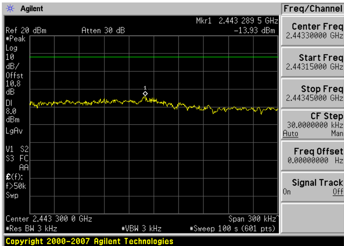
Plot 6-14. Power Spectral Density 36Mbps Data Rate Plot (802.11g – Ch. 6)
