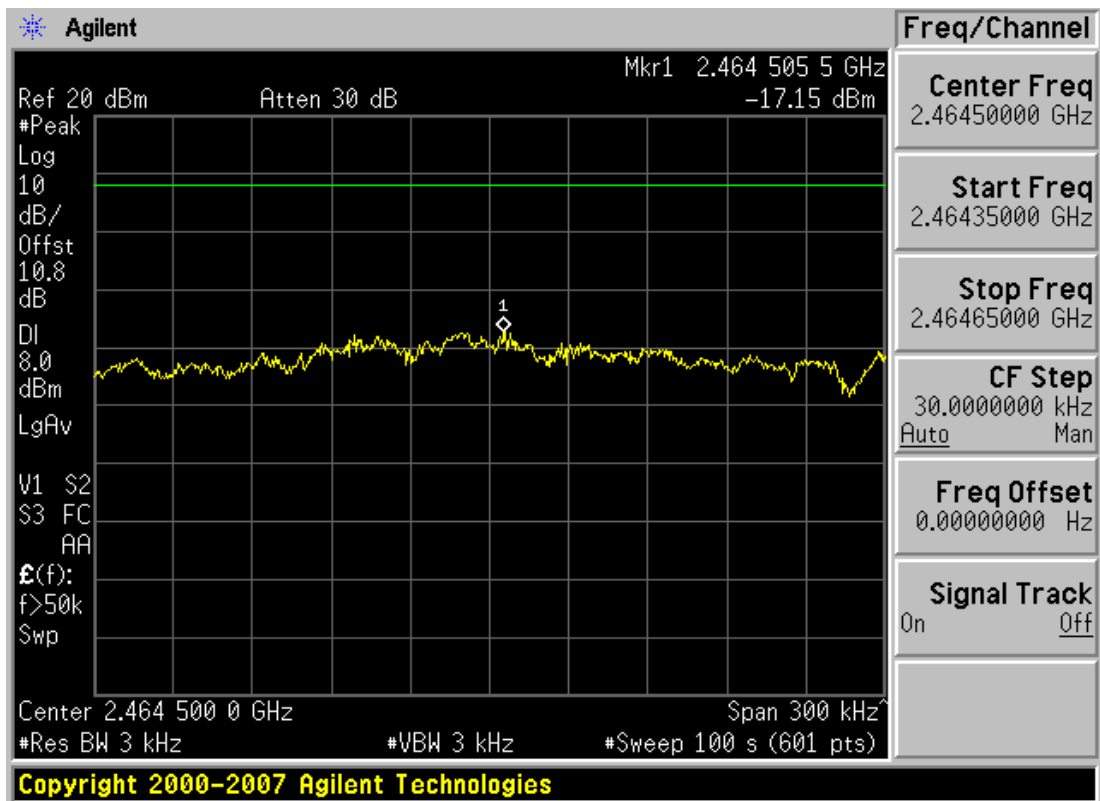
Plot 6-18. Power Spectral Density 19.5/21.7Mbps (802.11n – Ch. 11)
