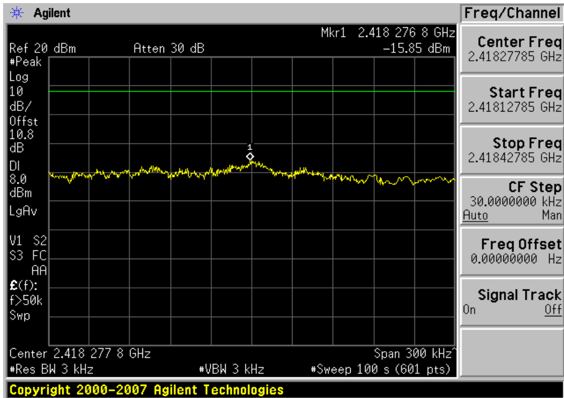
Plot 6-16. Power Spectral Density 19.5/21.7Mbps (802.11n – Ch. 1)
