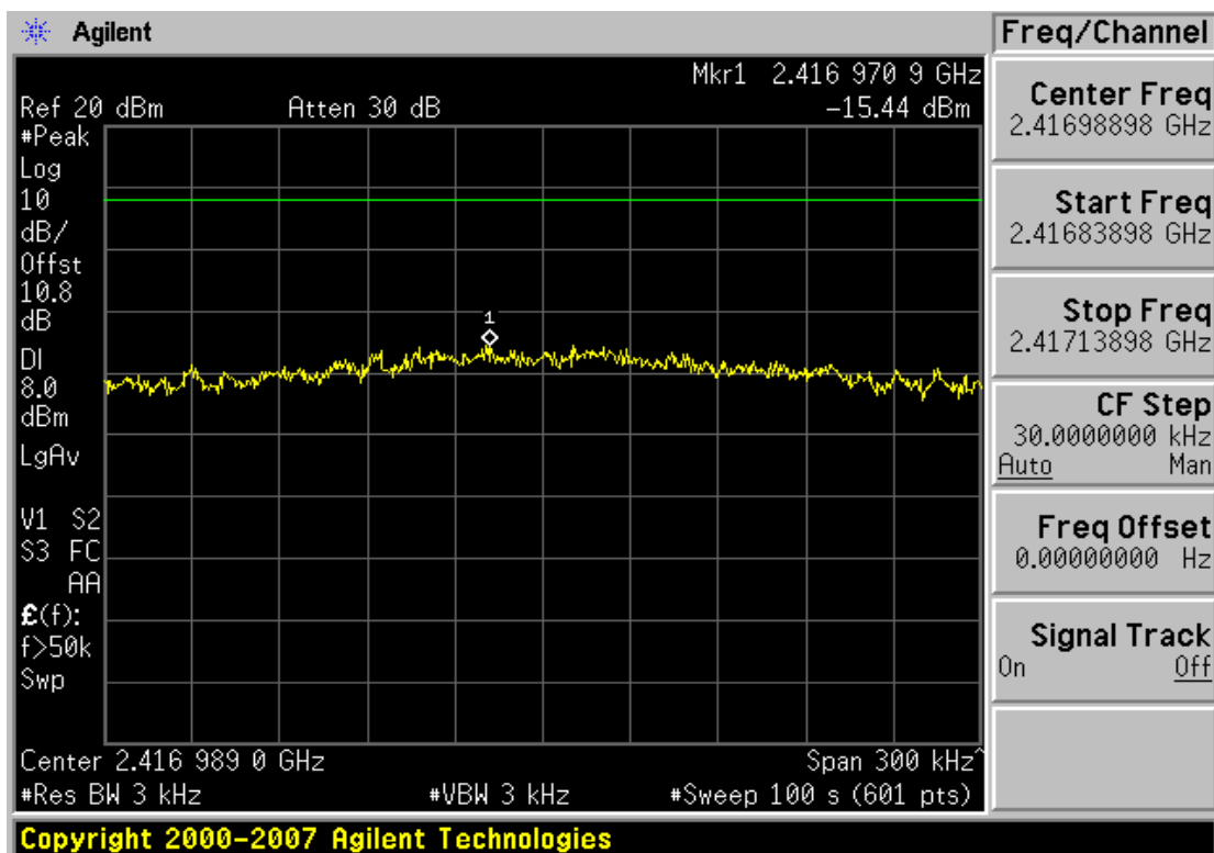
Plot 6-13. Power Spectral Density 36Mbps Data Rate Plot (802.11g – Ch. 1)
