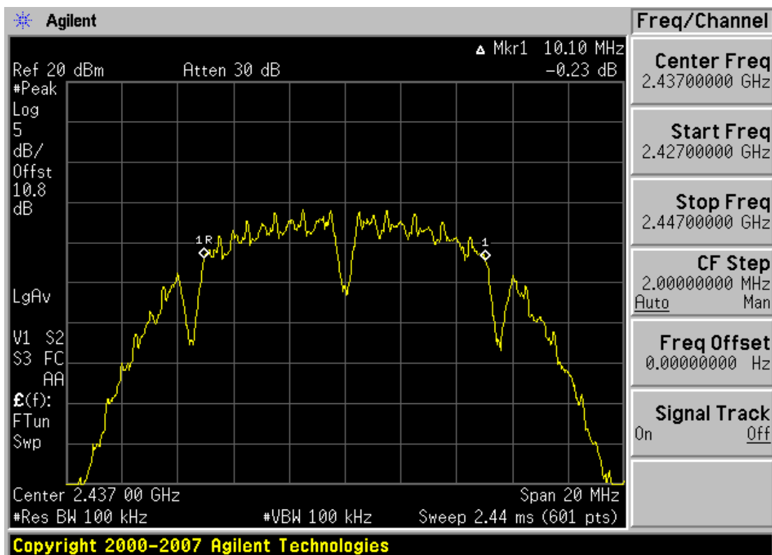
Plot 6-2. 6dB Bandwidth 1Mbps Data Rate Plot (802.11b – Ch. 6)
