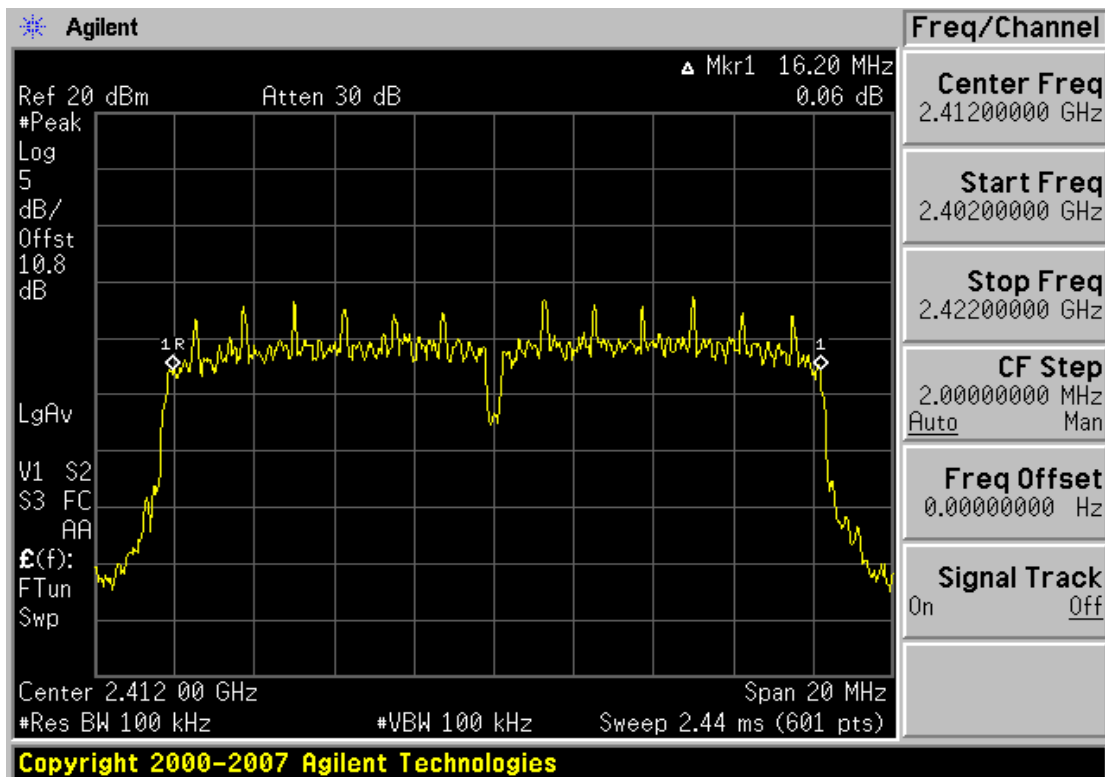
Plot 6-4. 6dB Bandwidth 36Mbps Data Rate Plot (802.11g – Ch. 1)
