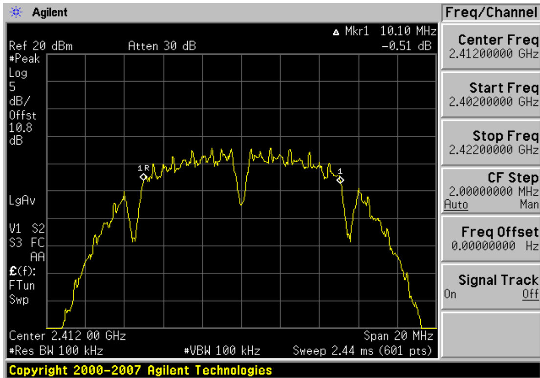
Plot 6-1. 6dB Bandwidth 1Mbps Data Rate Plot (802.11b – Ch. 1)
