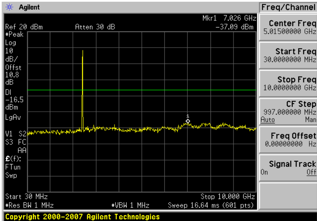
Plot 6-27. Conducted Spurious 1Mbps Data Rate Plot (802.11b – Ch. 6)
