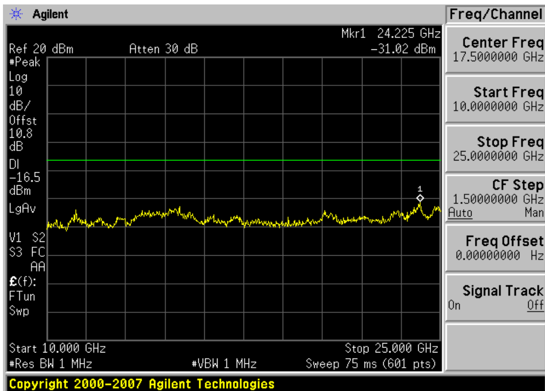
Plot 6-28. Conducted Spurious 1Mbps Data Rate Plot (802.11b – Ch. 6)
