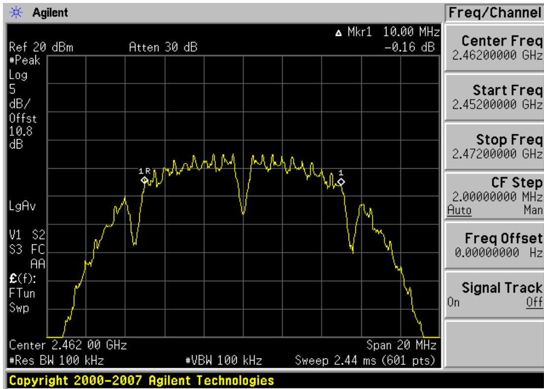
Plot 6-3. 6dB Bandwidth 1Mbps Data Rate Plot (802.11b – Ch. 11)
