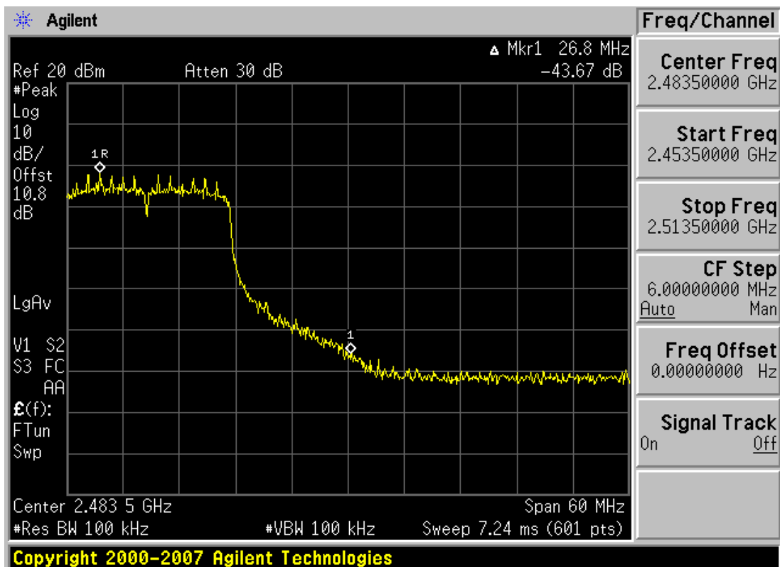
Plot 6-24. Band Edge 19.5/21.7Mbps (802.11n – Ch. 11)
