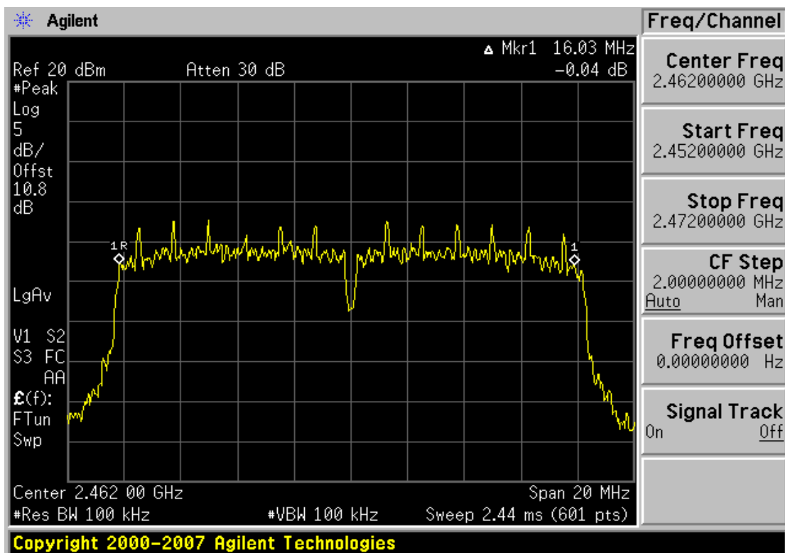
Plot 6-6. 6dB Bandwidth 36Mbps Data Rate Plot (802.11g - Ch. 11)
