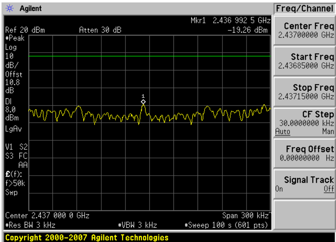
Plot 6-11. Power Spectral Density 1Mbps Data Rate Plot (802.11b – Ch. 6)
