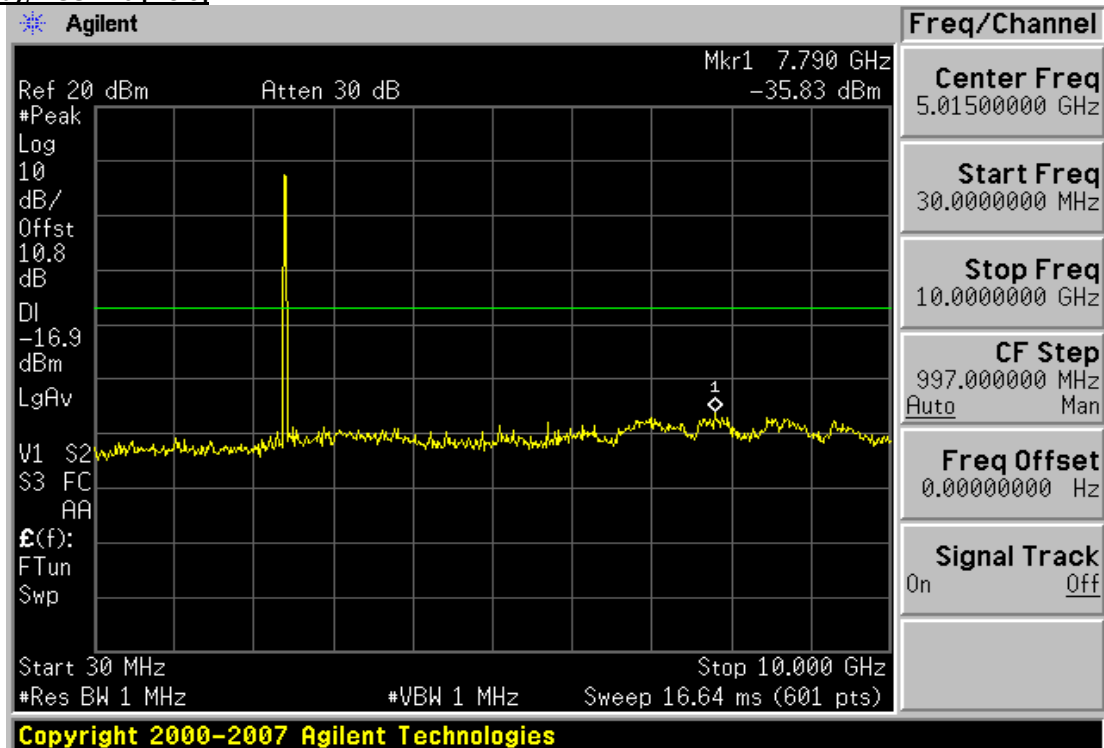
Plot 6-25. Conducted Spurious 1Mbps Data Rate Plot (802.11b – Ch. 1)
