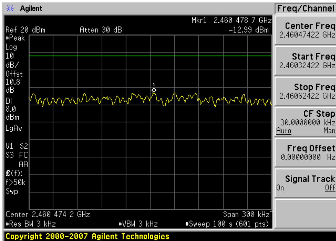
Plot 6-12. Power Spectral Density 1Mbps Data Rate Plot (802.11b – Ch. 11)
