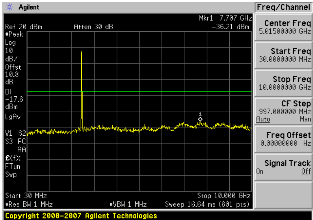
Plot 6-29. Conducted Spurious 1Mbps Data Rate Plot (802.11b – Ch. 11)
