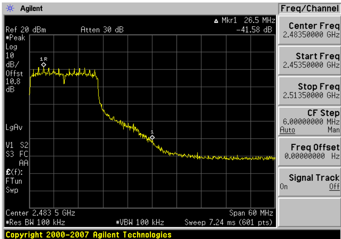
Plot 6-22. Band Edge 1Mbps Data Rate Plot (802.11g – Ch. 11)
