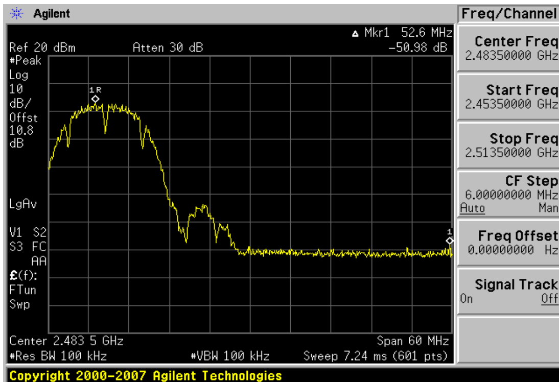
Plot 6-20. Band Edge 1Mbps Data Rate Plot (802.11b - Ch. 11)
