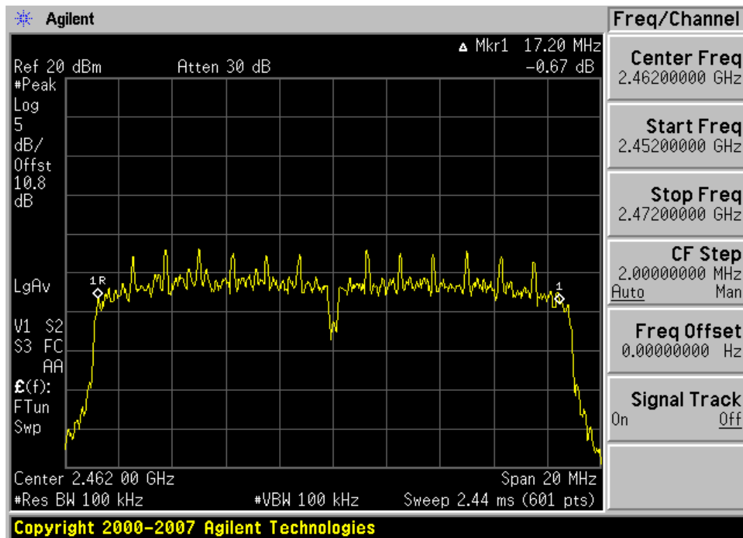
Plot 6-9. 6dB Bandwidth 19.5/21.7Mbps Data Rate Plot (802.11n – Ch. 11)
