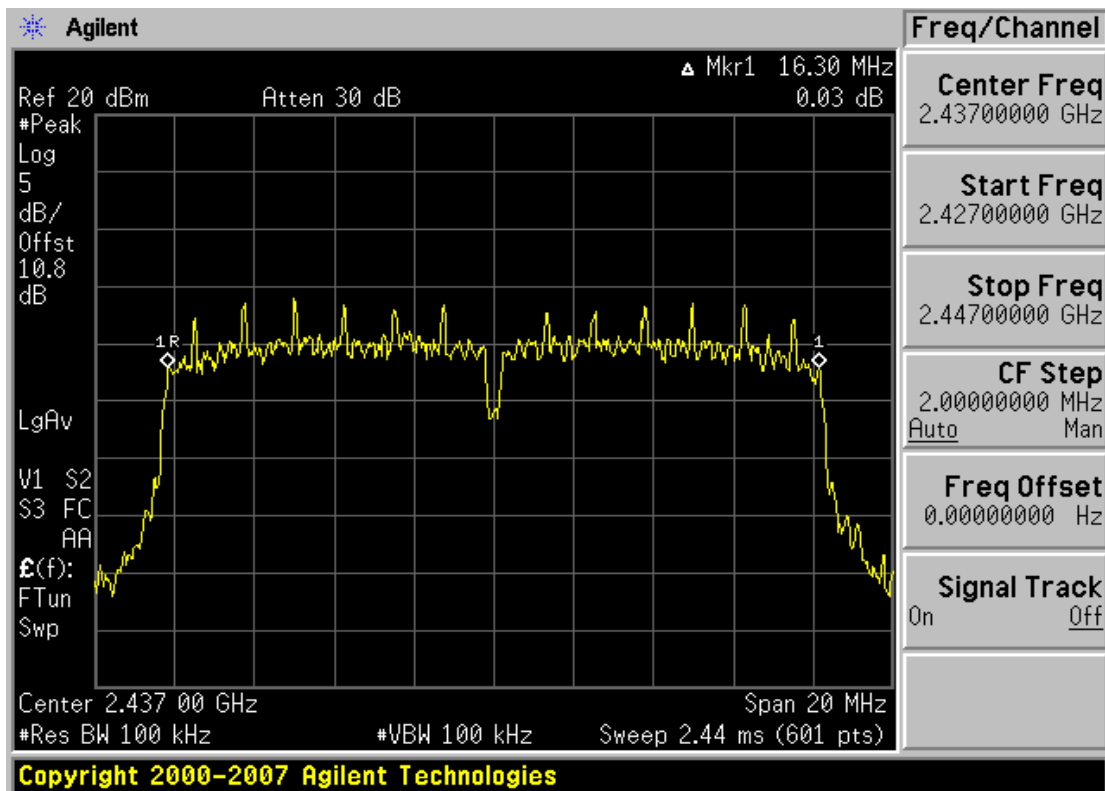
Plot 6-5. 6dB Bandwidth 36Mbps Data Rate Plot (802.11g - Ch. 6)
