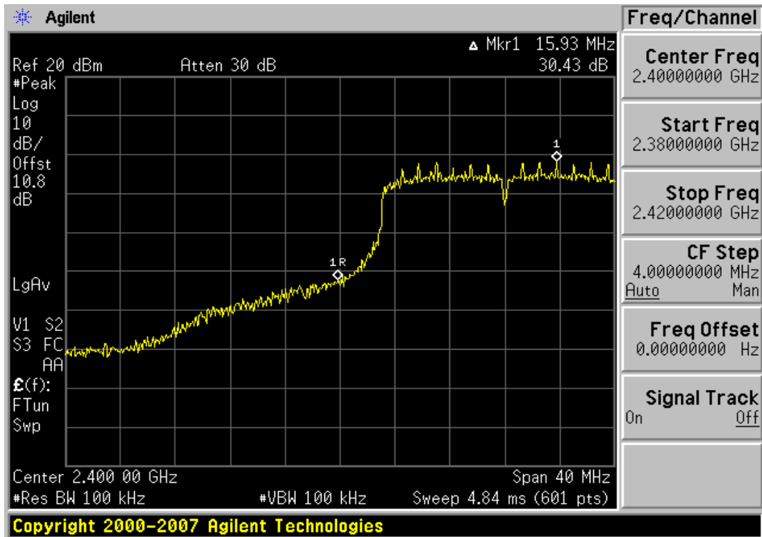
Plot 6-23. Band Edge 19.5/21.7Mbps (802.11n – Ch. 1)
