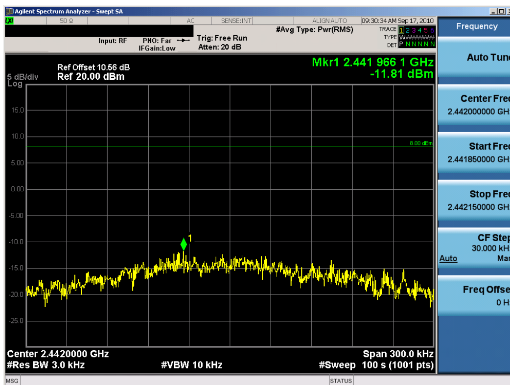
Plot 6-5. Power Spectral Density Plot (802.11g – Ch. 6)
