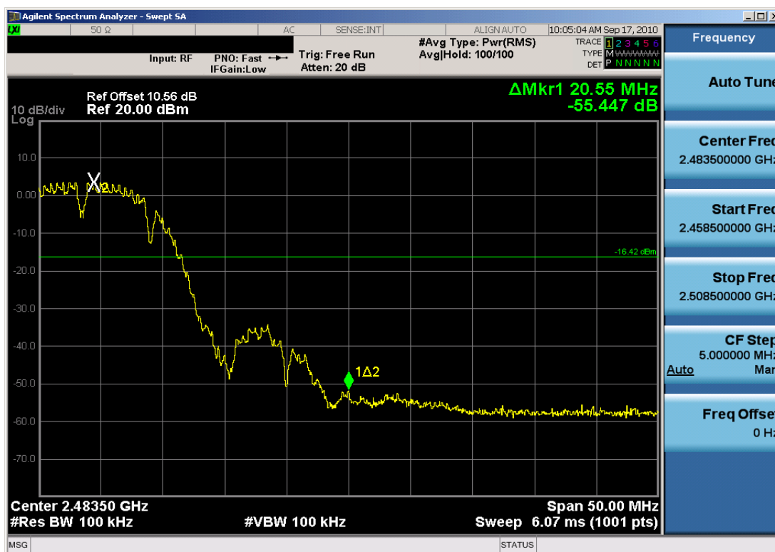
Plot 6-8. Band Edge Plot (802.11b – Ch. 11)
