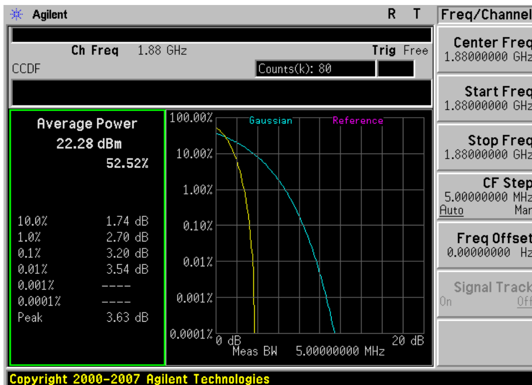
Plot 7-38. Peak-Average Ratio Plot (PCS WCDMA Mode – Ch. 9400)
