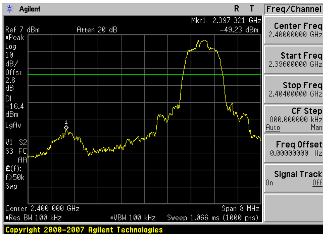
Plot 6-6. Band Edge Plot (Bluetooth (EDR) – Ch. 0)
