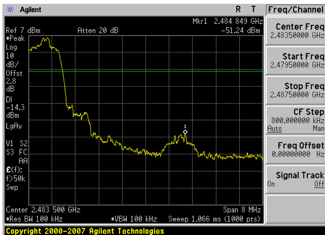
Plot 6-7. Band Edge Plot (Bluetooth (EDR) – Ch. 78)
