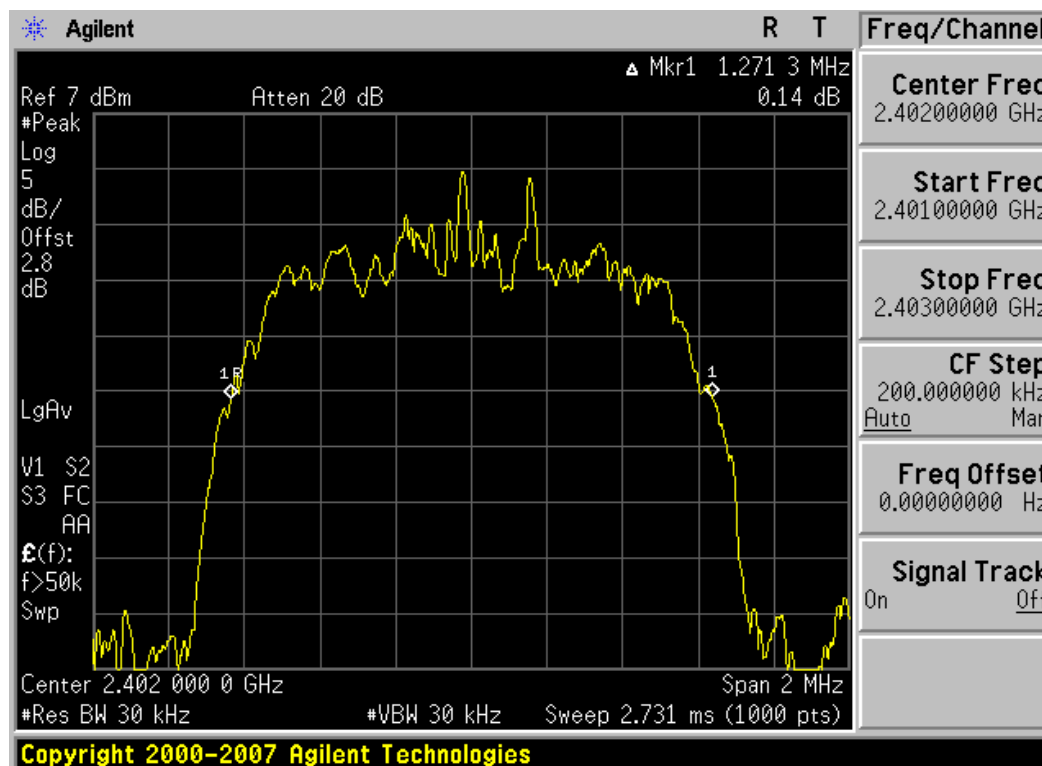
Plot 6-1. 20dB Bandwidth Plot (Bluetooth (EDR) – Ch. 0)
