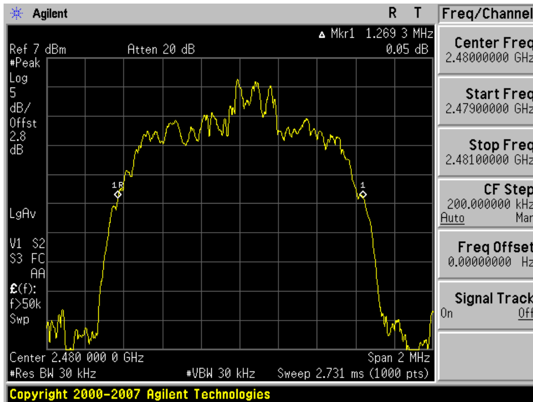
Plot 6-3. 20dB Bandwidth Plot (Bluetooth (EDR) – Ch. 78)
