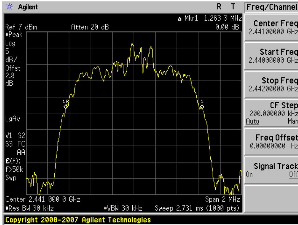
Plot 6-2. 20dB Bandwidth Plot (Bluetooth (EDR) – Ch. 39)
