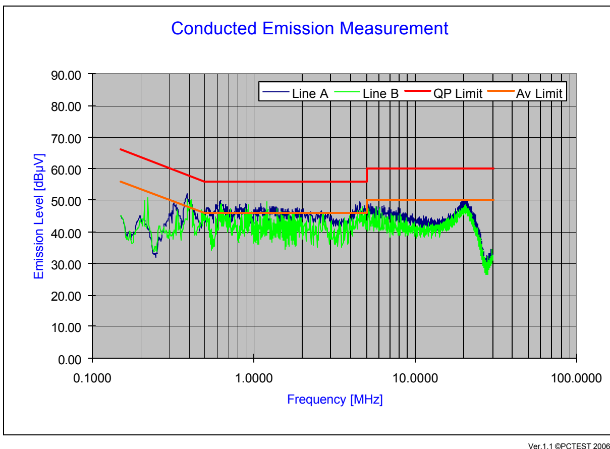
Plot 6-18. Line Conducted Plot with Bluetooth
