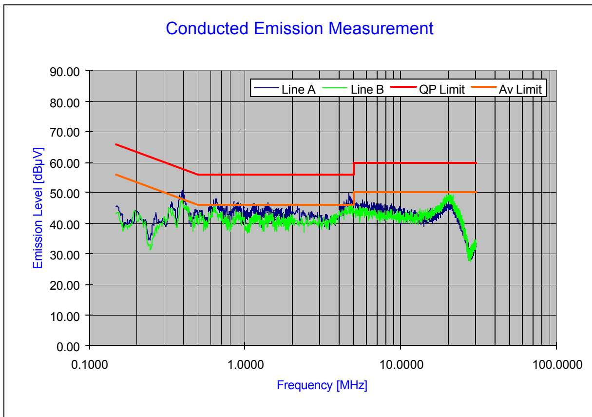
lot 6-18. Line Conducted Plot with Bluetooth
