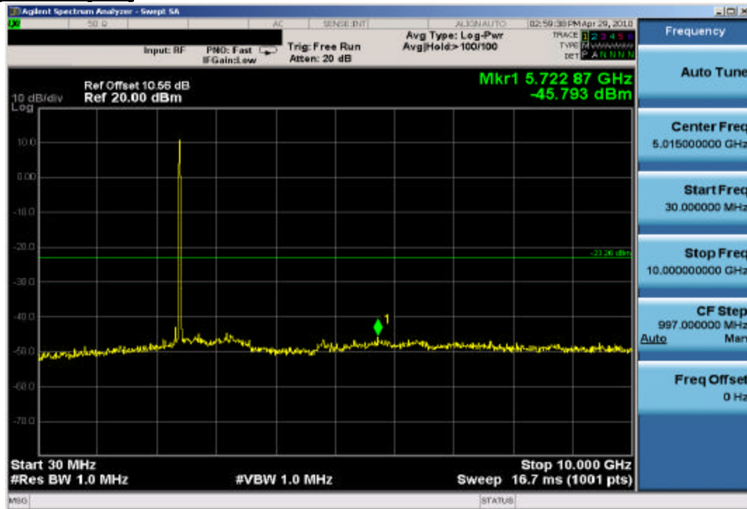
Plot 6-25. Conducted Spurious Plot (802.11b – Ch. 1)
