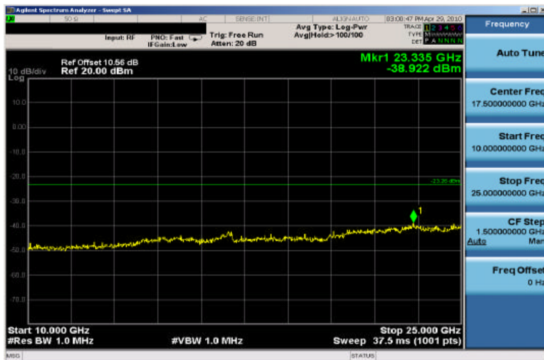
Plot 6-26. Conducted Spurious Plot (802.11b – Ch. 1)
