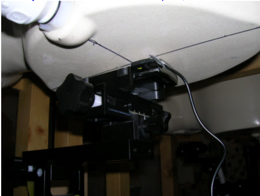
12. Body SAR, Back Side with 15mm Space, Slide In
