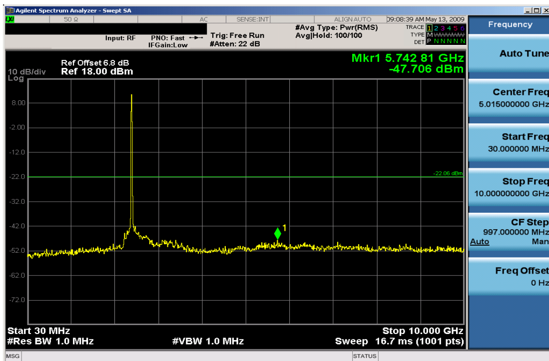
Plot 6-17. Conducted Spurious Plot (802.11b – Ch. 1)
