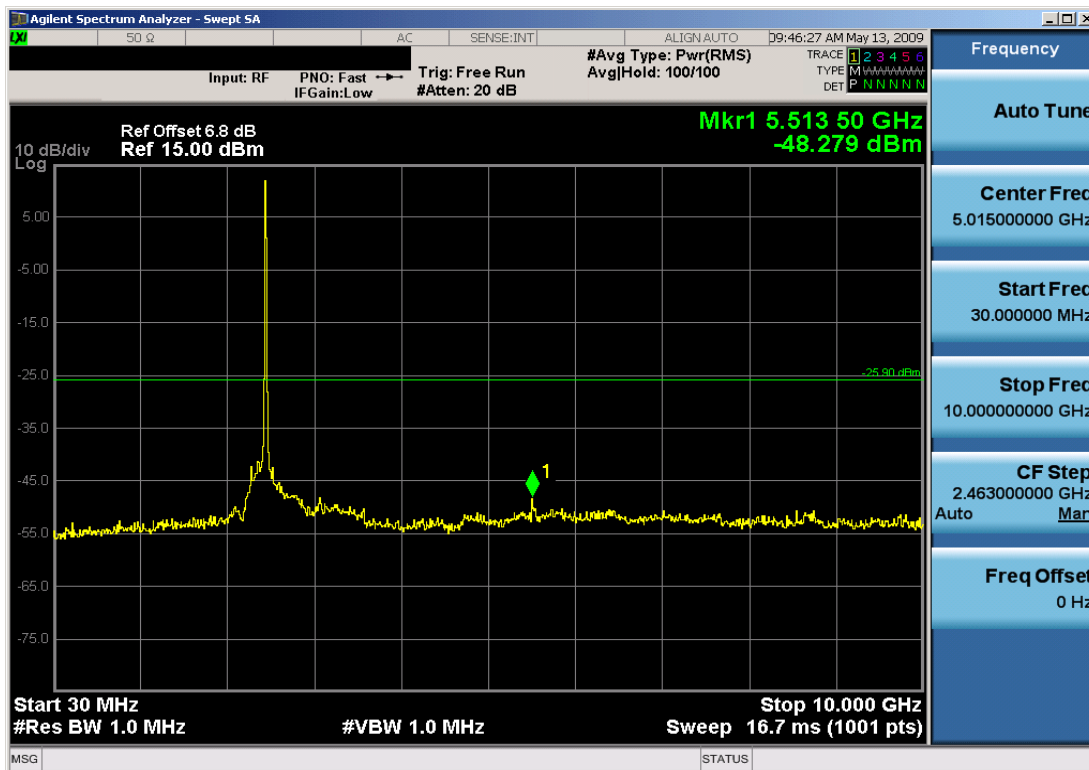
Plot 6-21. Conducted Spurious Plot (802.11b – Ch. 11)
