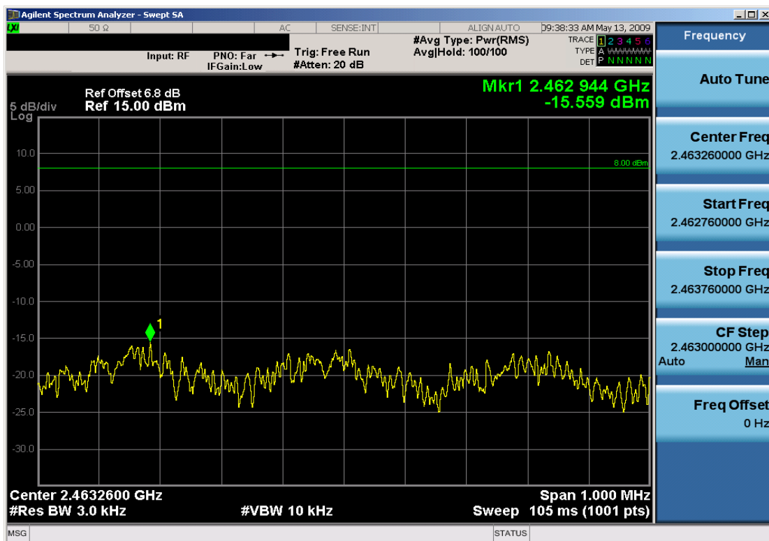
Plot 6-12. Power Spectral Density Plot (802.11g – Ch. 11)
