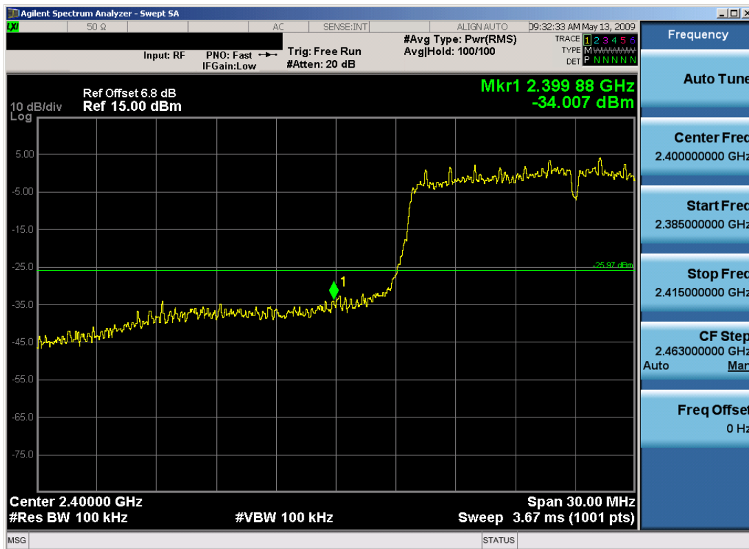
Plot 6-15. Band Edge Plot (802.11g – Ch. 1)
