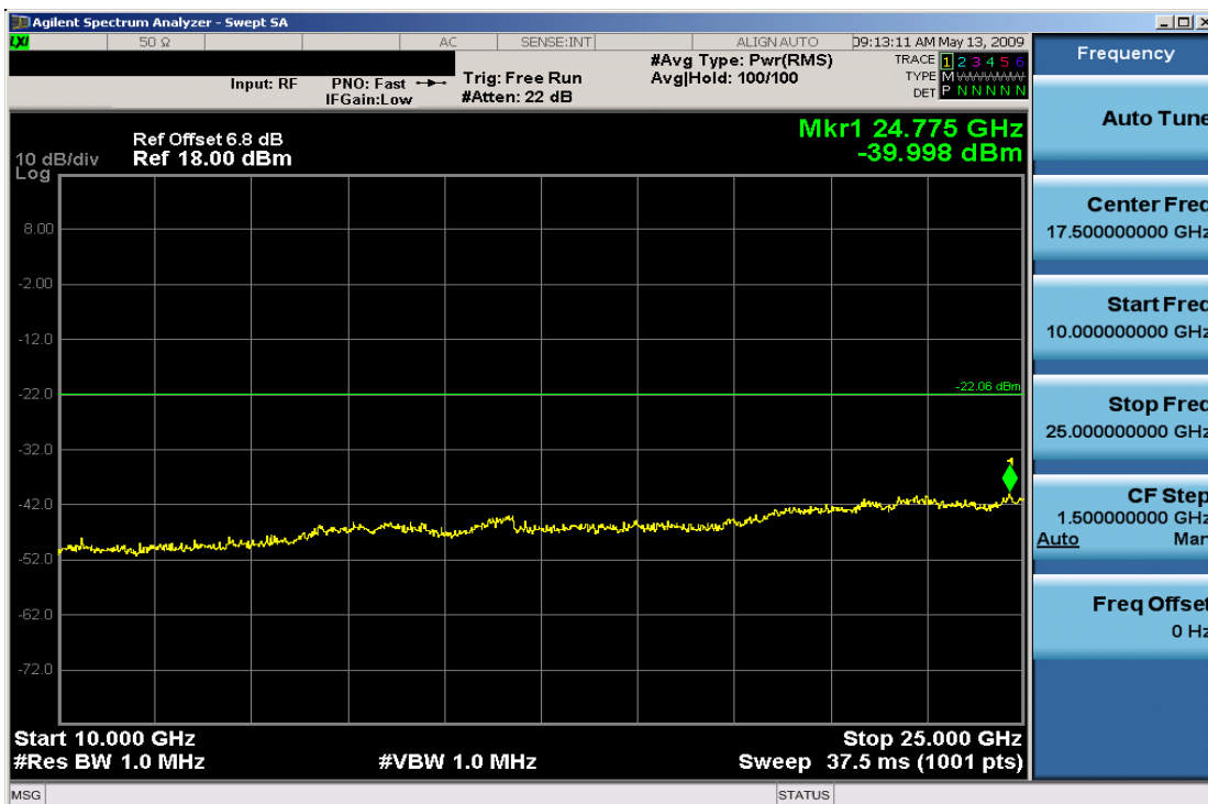
Plot 6-18. Conducted Spurious Plot (802.11b – Ch. 1)
