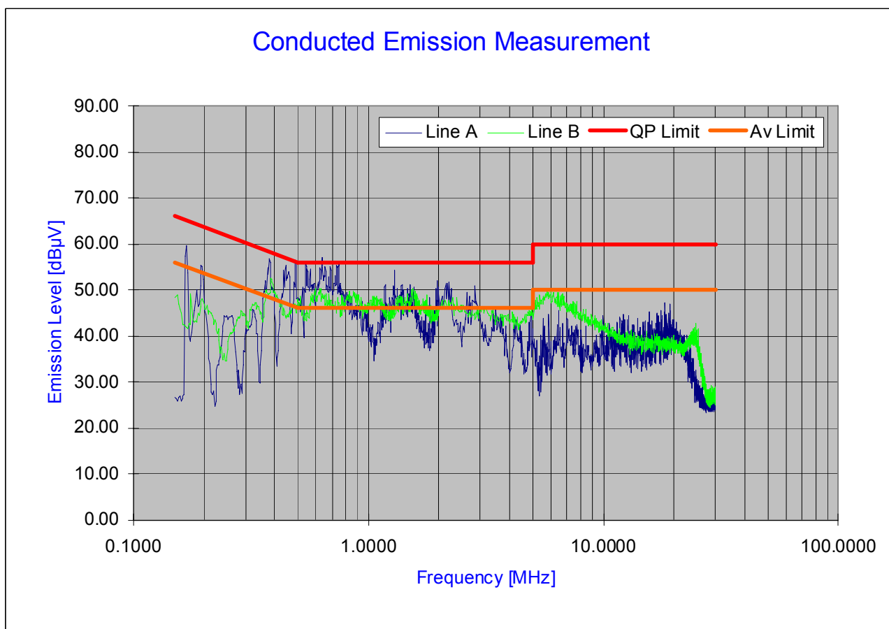
Plot 6-23. Line Conducted Plot with 802.11b
