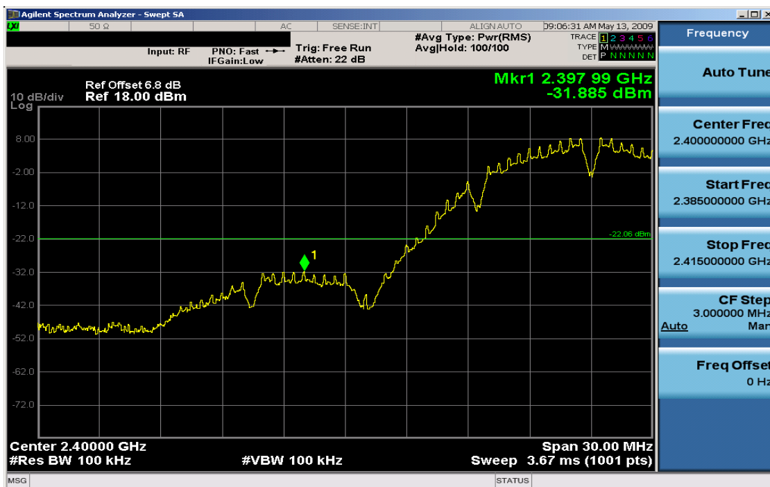
Plot 6-13. Band Edge Plot (802.11b – Ch. 1)
