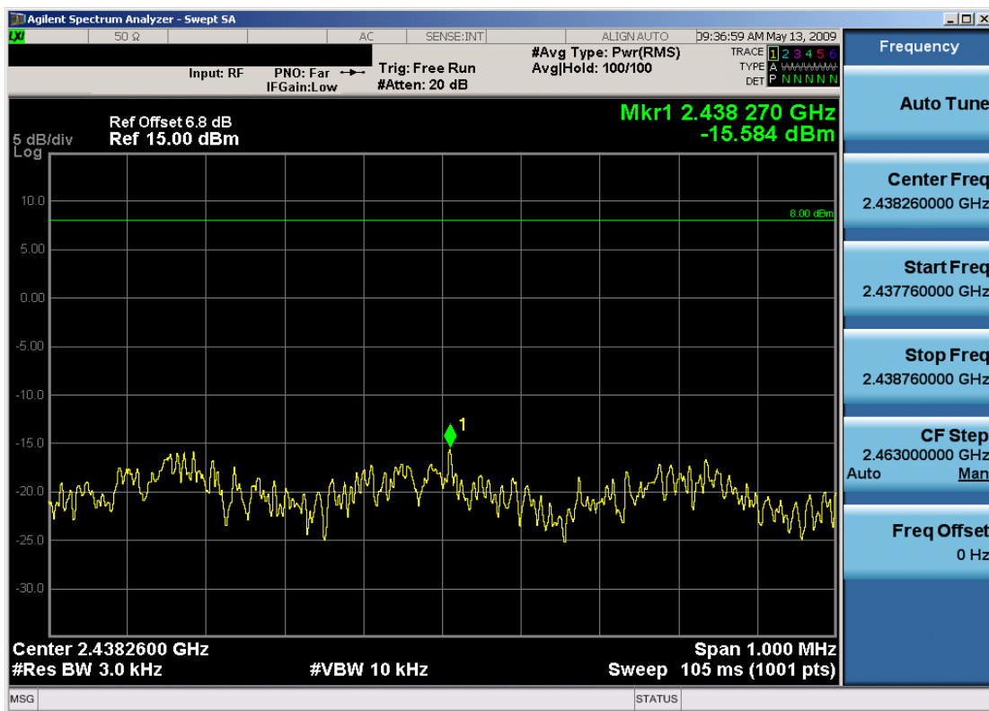
Plot 6-11. Power Spectral Density Plot (802.11g – Ch. 6)
