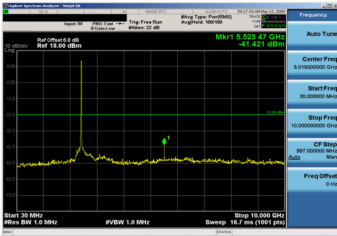
Plot 6-19. Conducted Spurious Plot (802.11b – Ch. 6)
