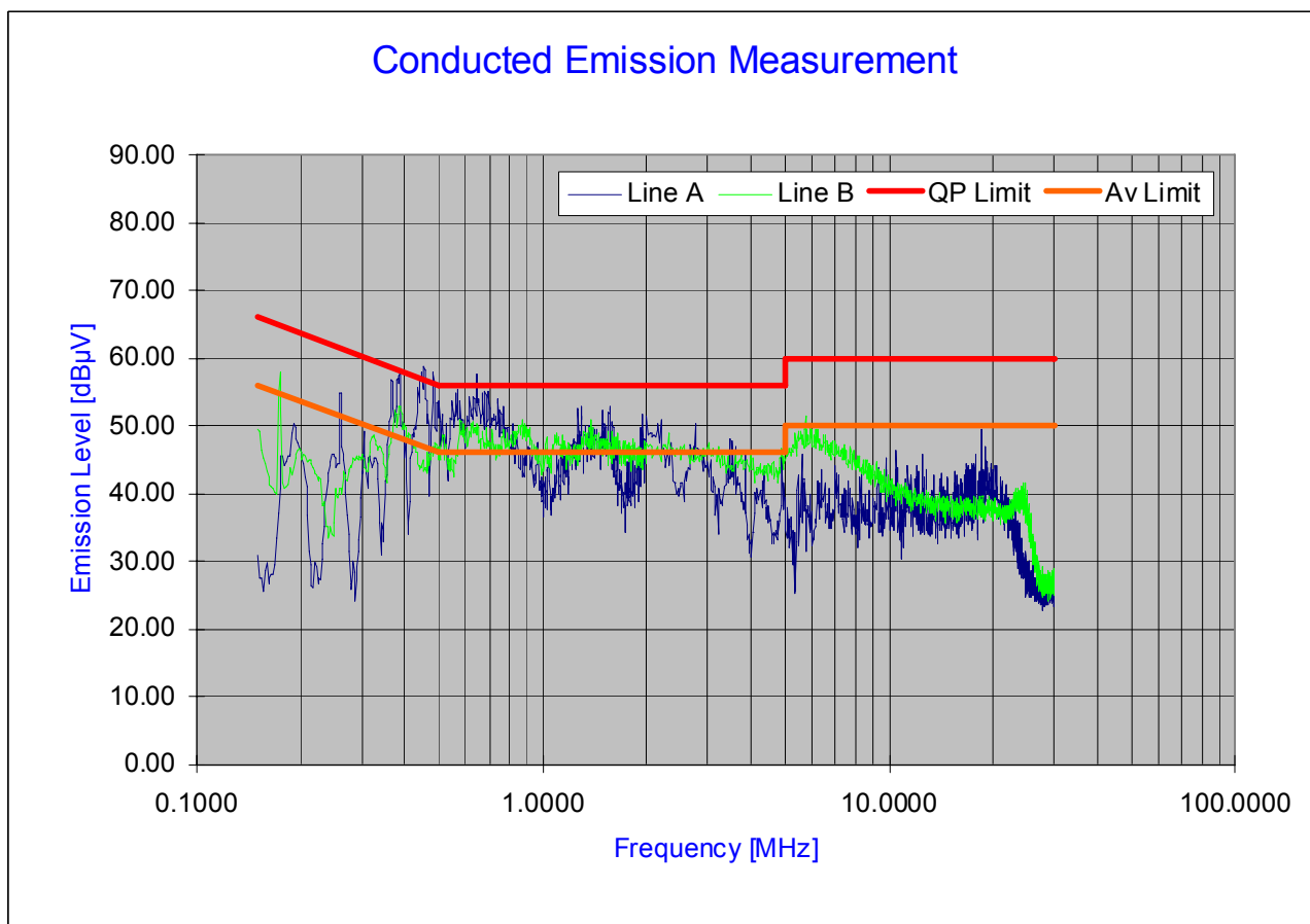
Plot 6-24. Line Conducted Plot with 802.11g
