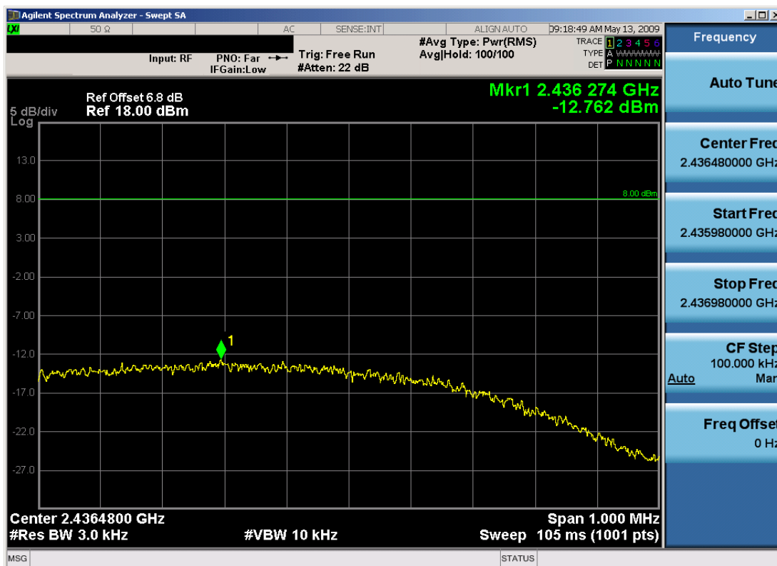
Plot 6-8. Power Spectral Density Plot (802.11b – Ch. 6)
