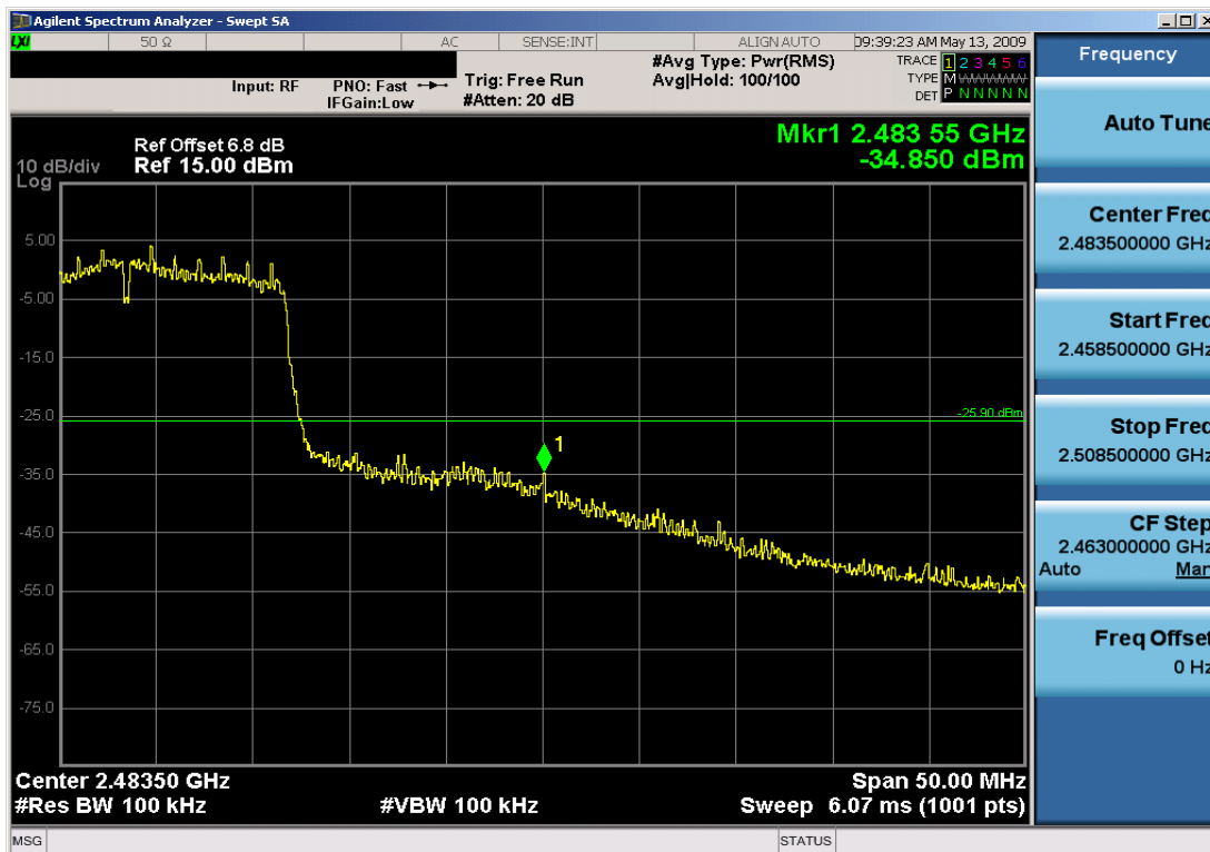
Plot 6-16. Band Edge Plot (802.11g – Ch. 11)
