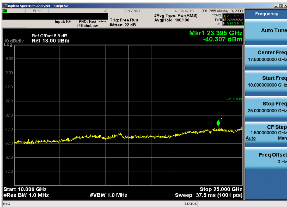
Plot 6-20. Conducted Spurious Plot (802.11b – Ch. 6)
