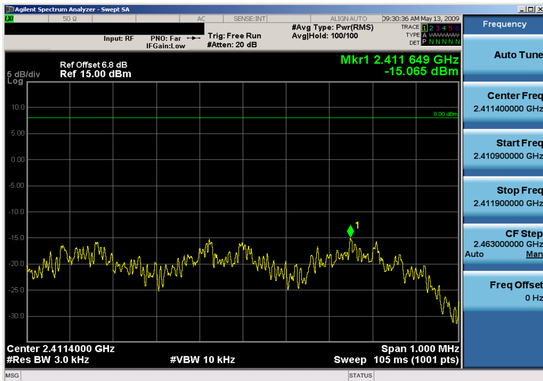
Plot 6-10. Power Spectral Density Plot (802.11g – Ch. 1)
