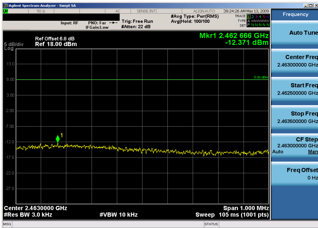
Plot 6-9. Power Spectral Density Plot (802.11b – Ch. 11)
