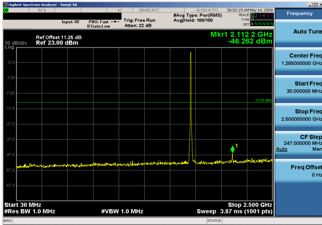
Plot 7-1. Conducted Spurious Plot (AWS WCDMA Mode – Ch. 1312)
