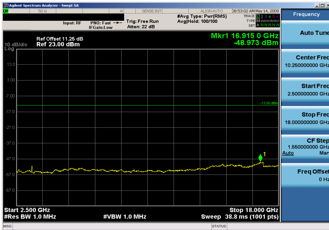
Plot 7-2. Conducted Spurious Plot (AWS WCDMA Mode – Ch. 1312)
