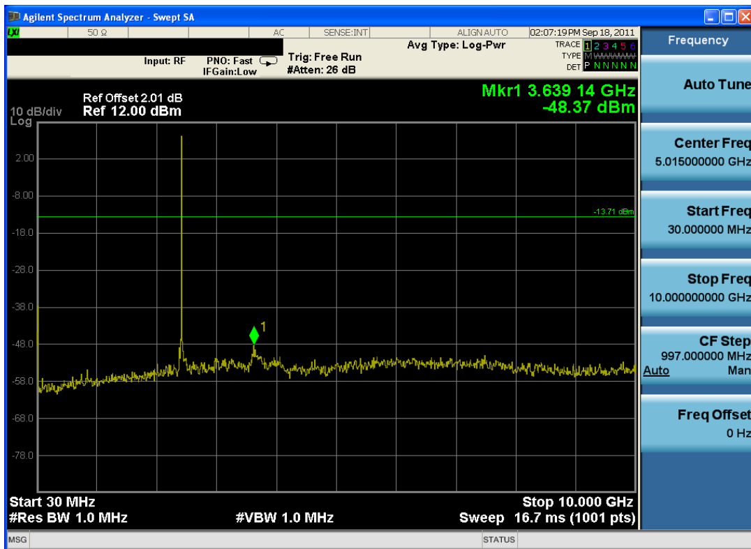
Plot 6-18. Conducted Spurious Plot (Bluetooth, 2Mbps – Ch. 39)
