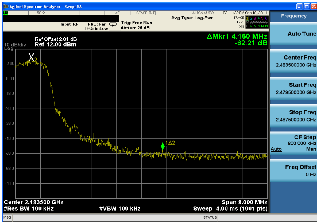
Plot 6-11. Band Edge Plot (Bluetooth, 2Mbps – Ch. 78)
