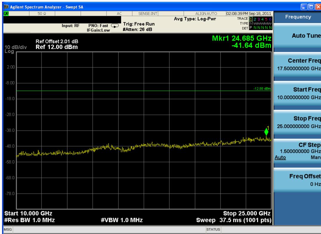
Plot 6-21. Conducted Spurious Plot (Bluetooth, 2Mbps – Ch. 78)
