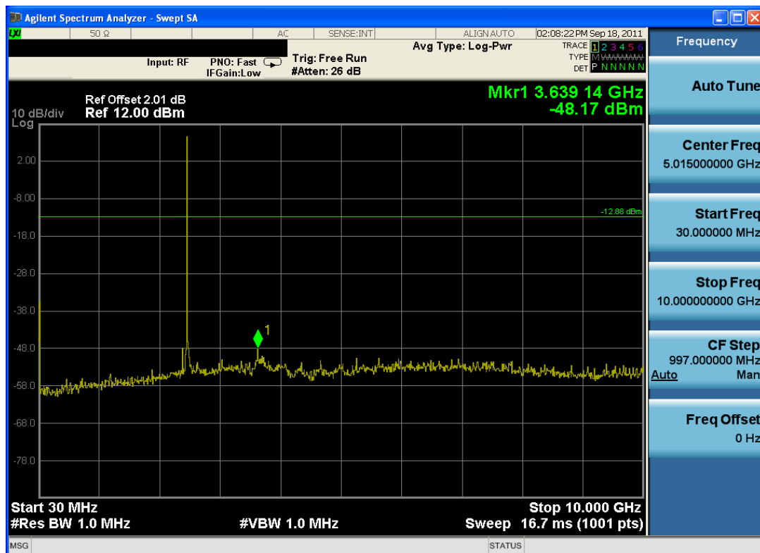
Plot 6-20. Conducted Spurious Plot (Bluetooth, 2Mbps – Ch. 78)
