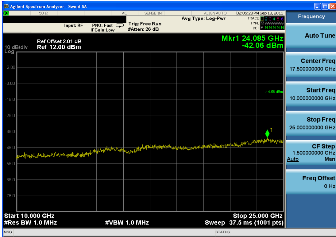
Plot 6-17. Conducted Spurious Plot (Bluetooth, 2Mbps – Ch. 0)
