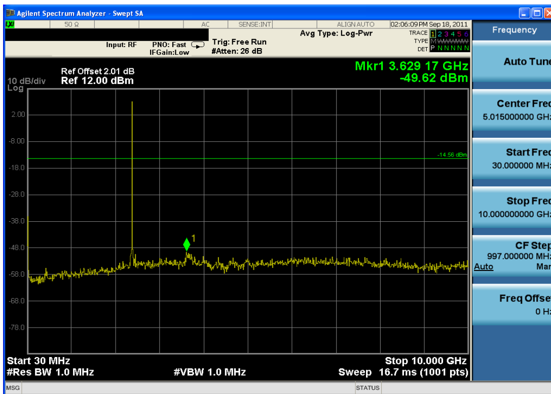
Plot 6-16. Conducted Spurious Plot (Bluetooth, 2Mbps – Ch. 0)
