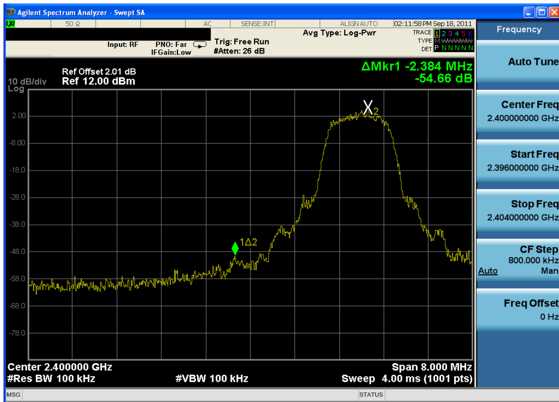
Plot 6-10. Band Edge Plot (Bluetooth, 2Mbps – Ch. 0)
