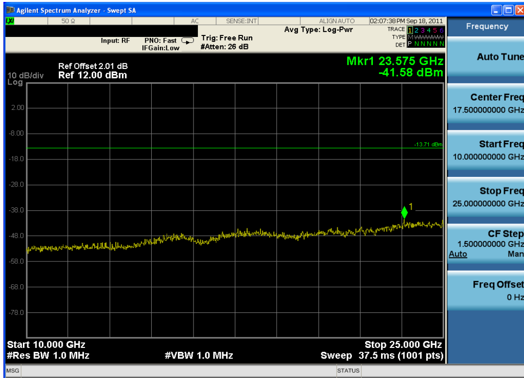
Plot 6-19. Conducted Spurious Plot (Bluetooth, 2Mbps – Ch. 39)
