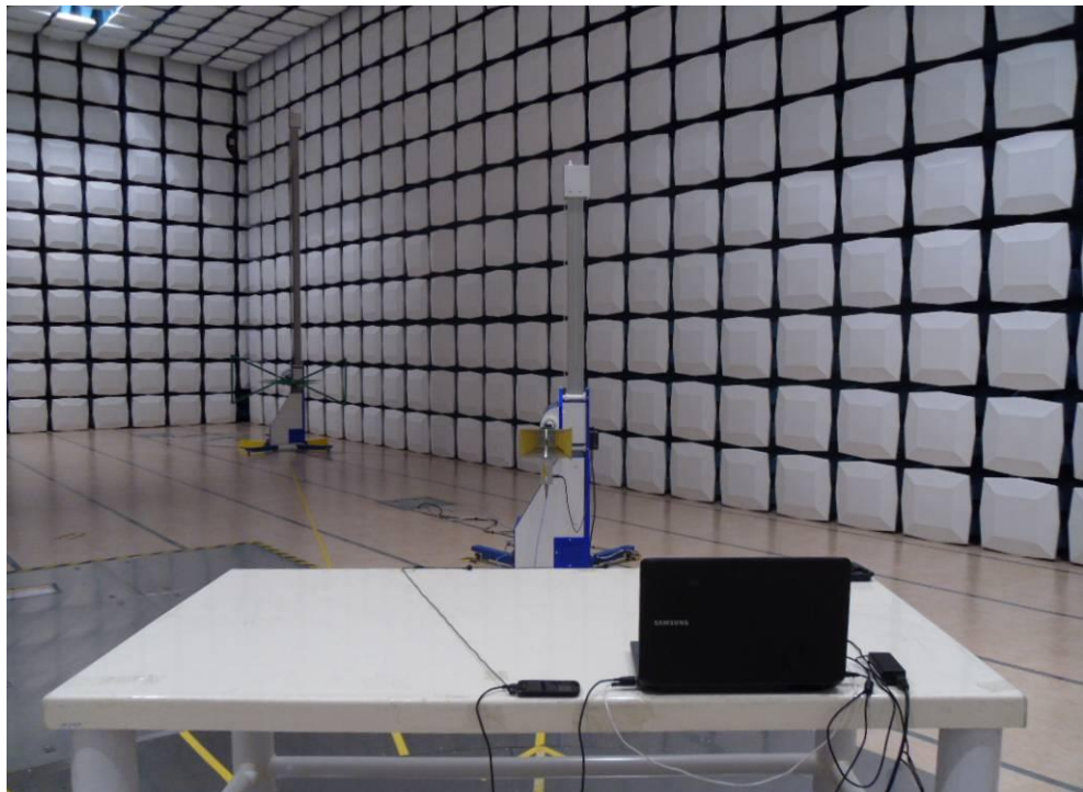
[ Radiated Disturbance for Above 1 GHz – Rear ]
