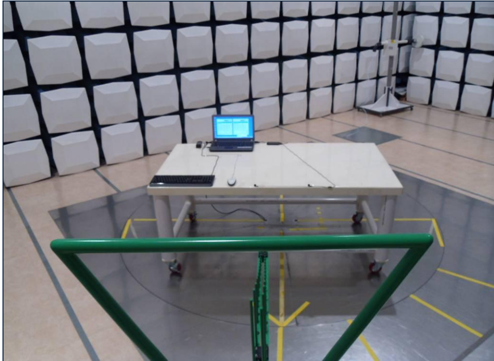
[ Radiated Disturbance for Below 1 GHz – Front ]
