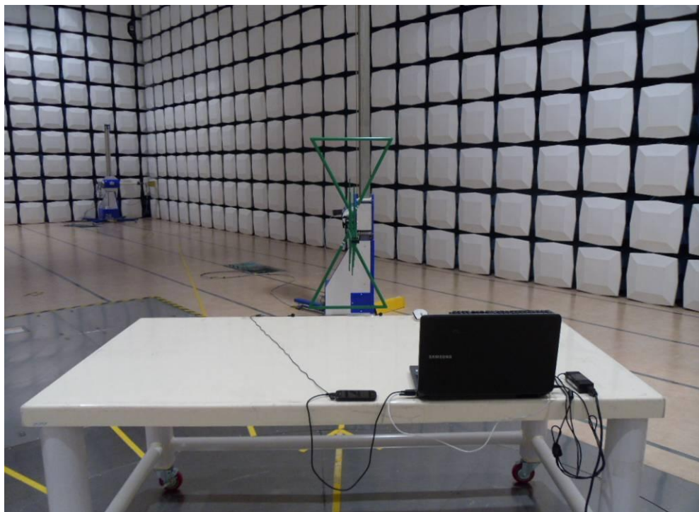
[ Radiated Disturbance for Below 1 GHz – Rear ]
