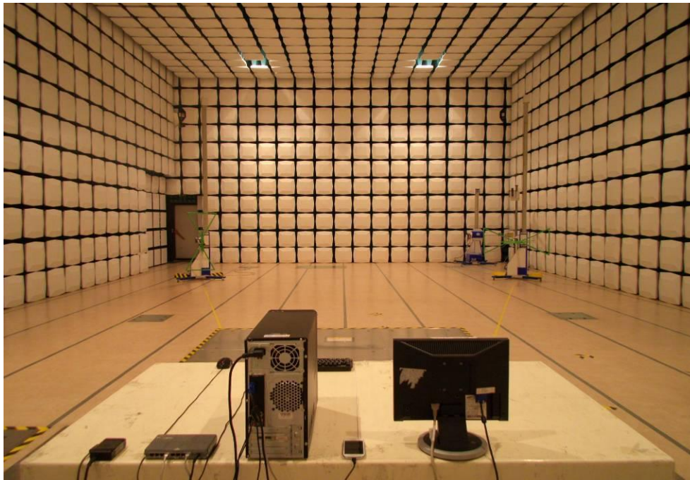
[ Radiated Disturbance for Below 1 GHz – Rear ]
