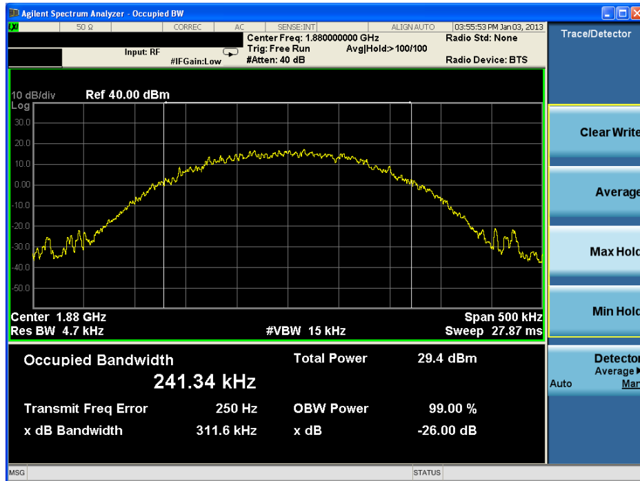
Plot 7-21. Occupied Bandwidth Plot (EDGE1900 Mode – Ch. 661)
