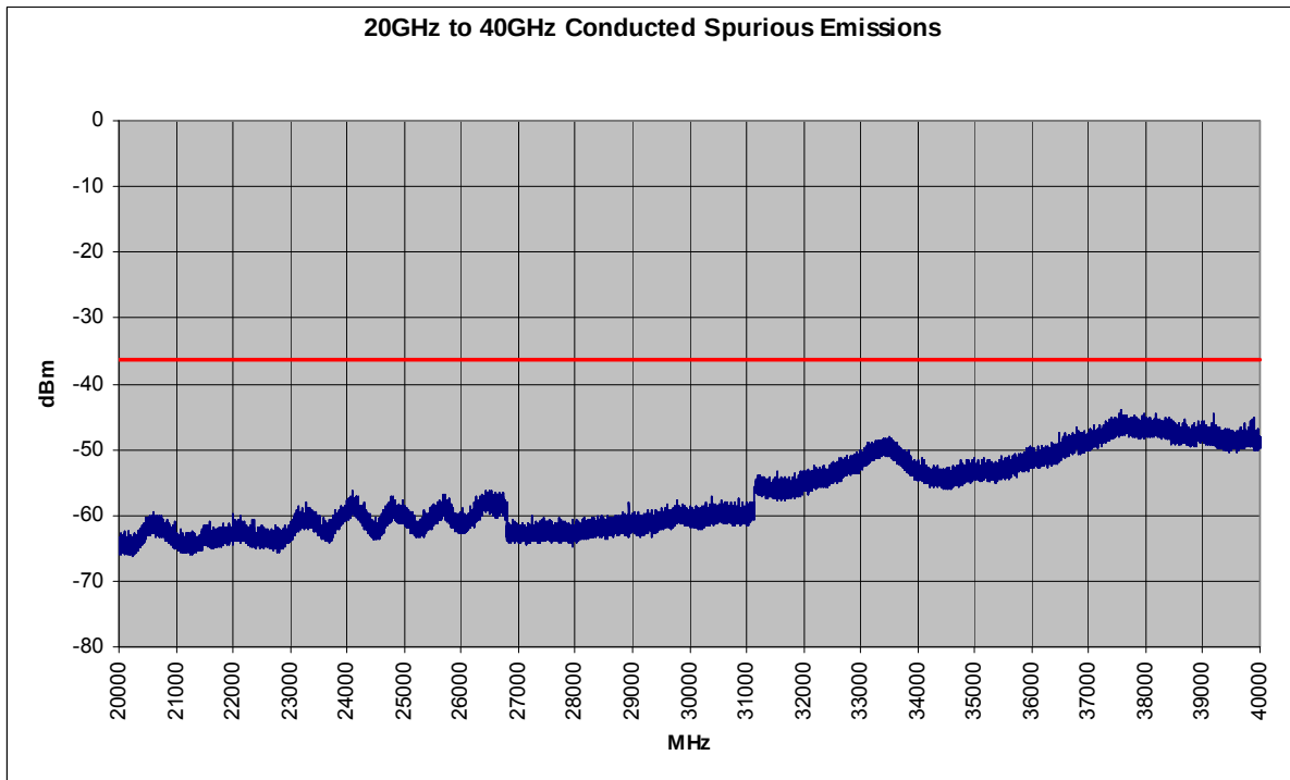
Plot 6-58. Conducted Spurious Plot (802.11a – Ch. 165)
