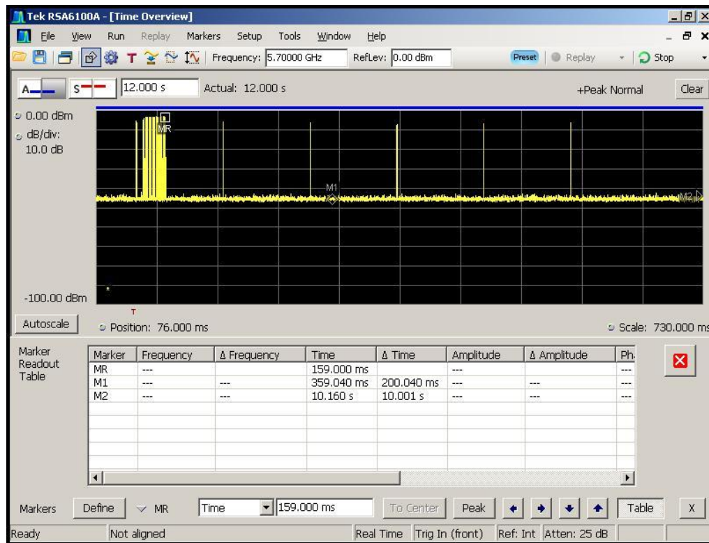
Figure 6-5. Channel Move Time Zoomed in (< 0.73sec)
