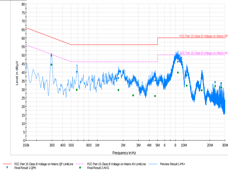
Plot 6-44. Line-Conducted Test Plot (L1)
