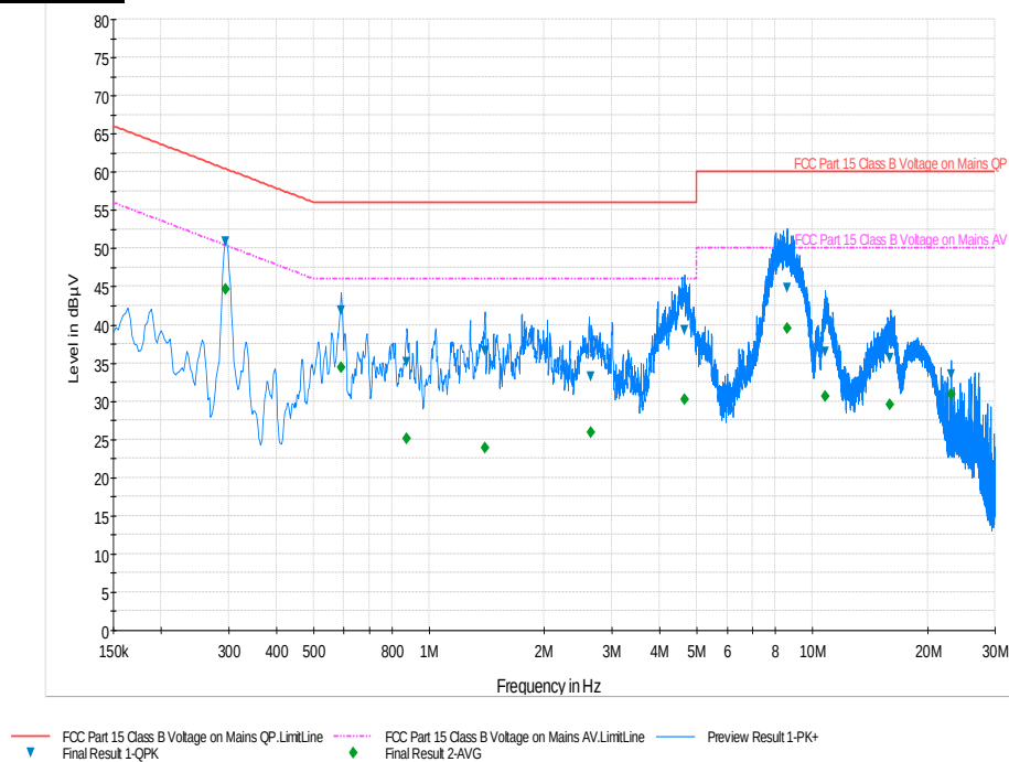
Plot 6-45. Line-Conducted Test Plot (N)
