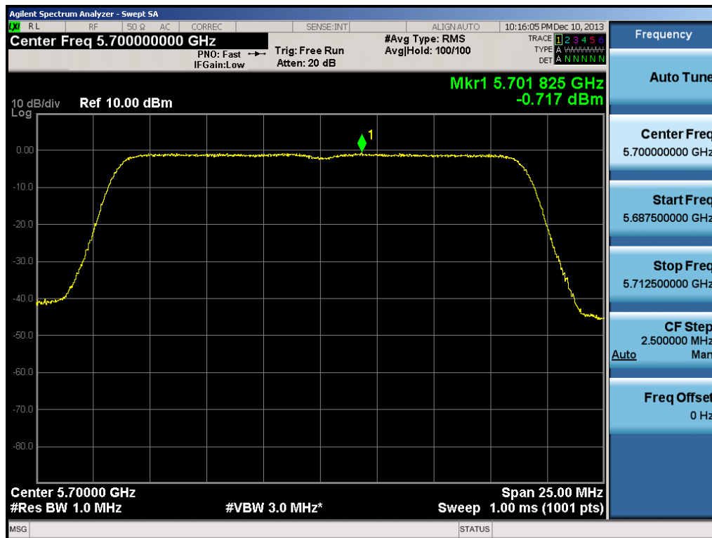
Plot 6-48. Peak Power Spectral Density Plot (20MHz BW 802.11n (UNII Band 2C) – Ch. 140)
