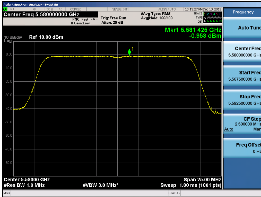
Plot 6-47. Peak Power Spectral Density Plot (20MHz BW 802.11n (UNII Band 2C) – Ch. 116)
