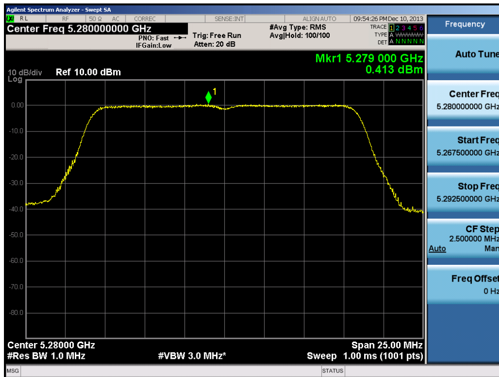
Plot 6-36. Peak Power Spectral Density Plot (802.11a (UNII Band 2A) – Ch. 56)
