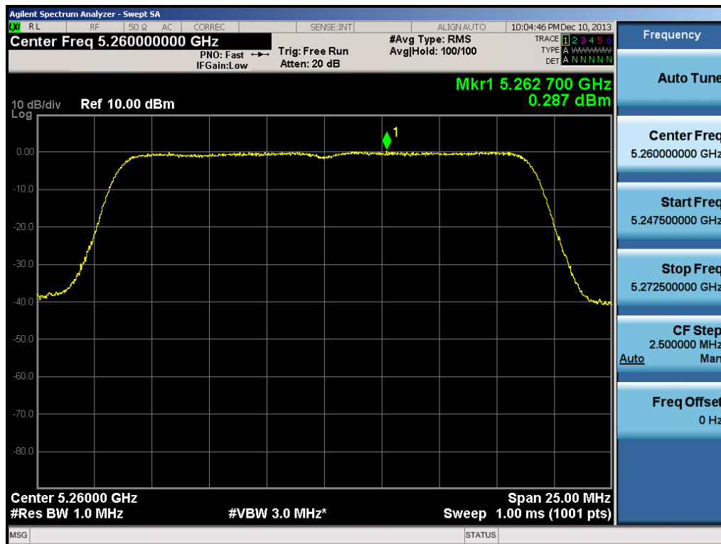
Plot 6-38. Peak Power Spectral Density Plot (20MHz BW 802.11n (UNII Band 2A) – Ch. 52)
