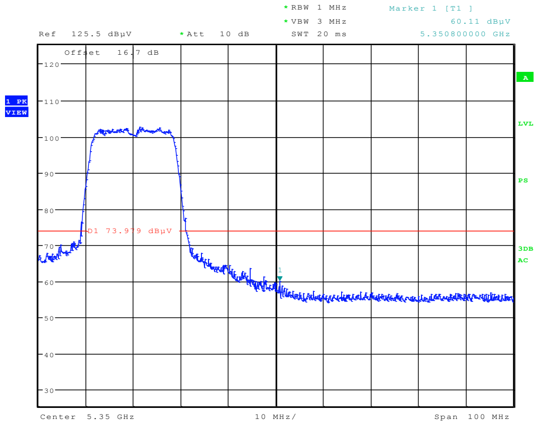
Plot 6-58. Radiated Restricted Upper Band Edge Plot (Peak – UNII Band 2A)
