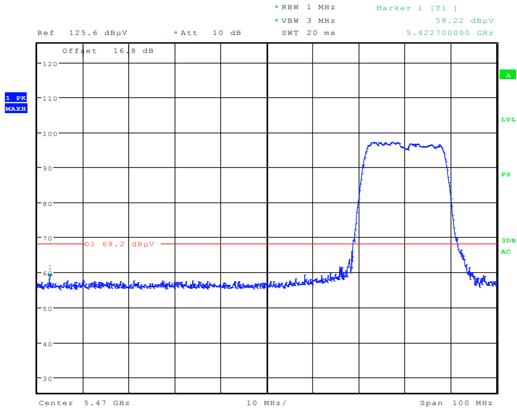
Plot 6-60. Radiated Restricted Lower Band Edge Plot (Peak – UNII Band 2C)
