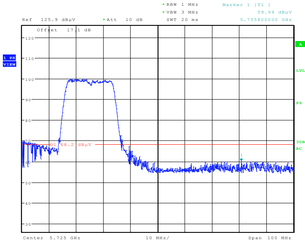
Plot 6-61. Radiated Upper Band Edge Plot (Peak – UNII Band 2C)
