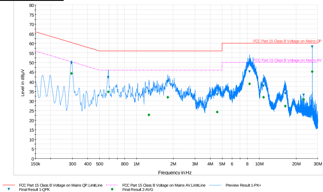
Plot 6-73. Line Conducted Plot with 802.11a UNII Band 2C (L1)
