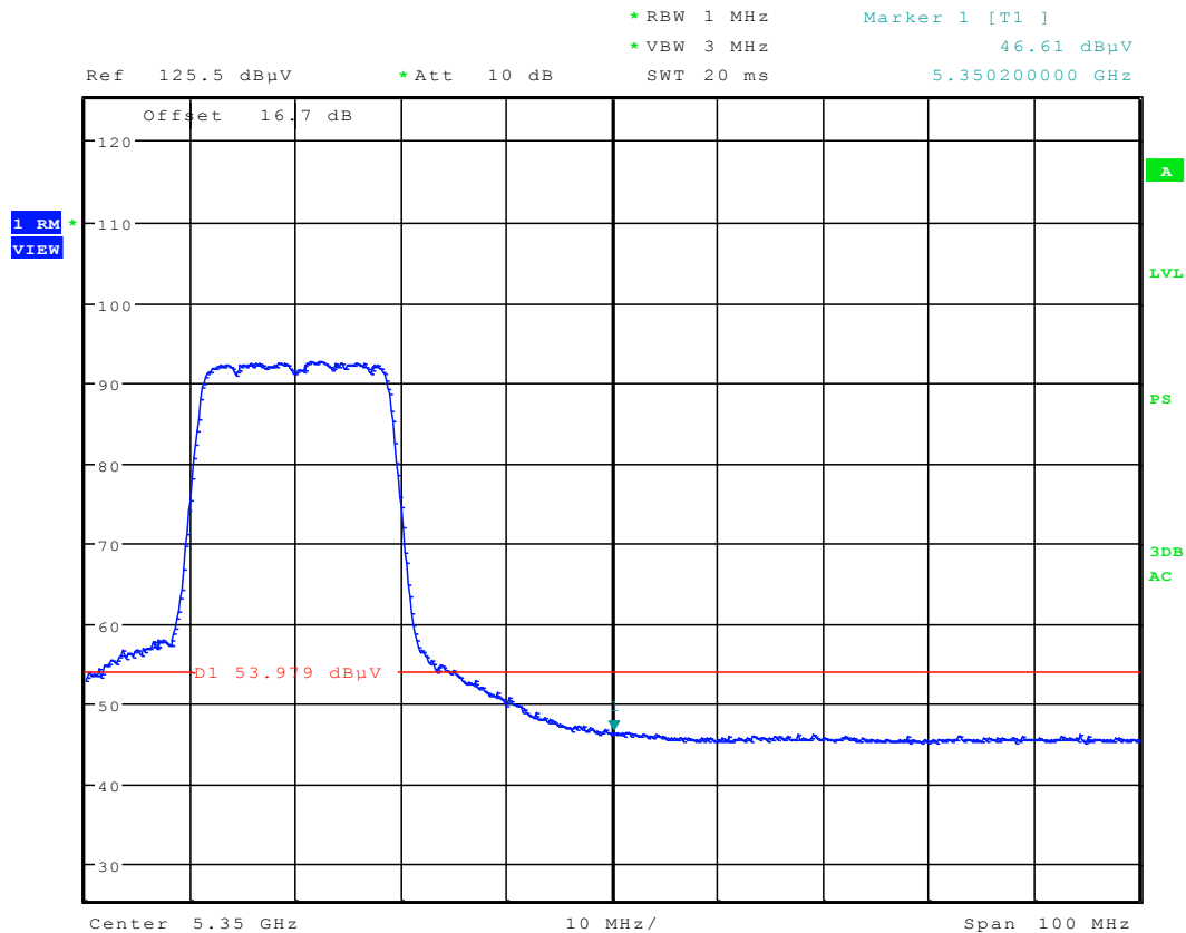
Plot 6-57. Radiated Restricted Upper Band Edge Plot (Average – UNII Band 2A)
