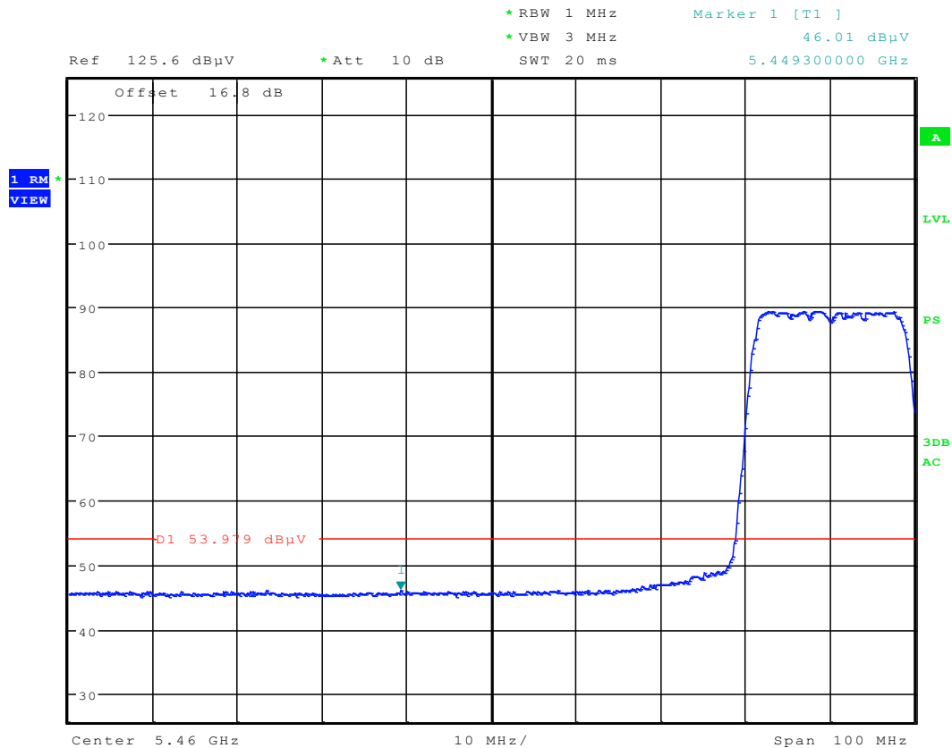
Plot 6-59. Radiated Restricted Lower Band Edge Plot (Average – UNII Band 2C)
