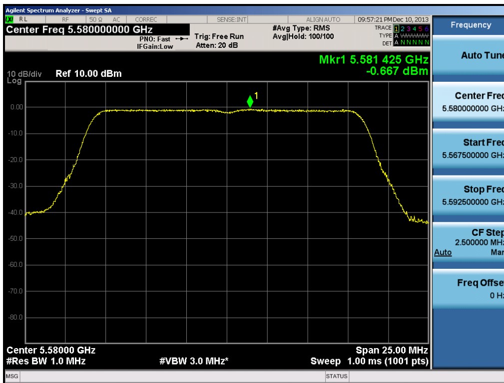
Plot 6-44. Peak Power Spectral Density Plot (802.11a (UNII Band 2C) – Ch. 116)
