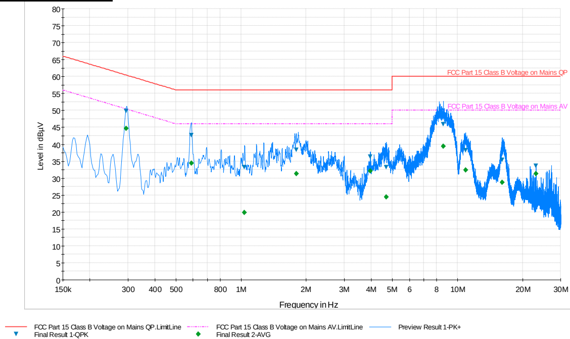
Plot 6-74. Line Conducted Plot with 802.11a UNII Band 2C (N)
