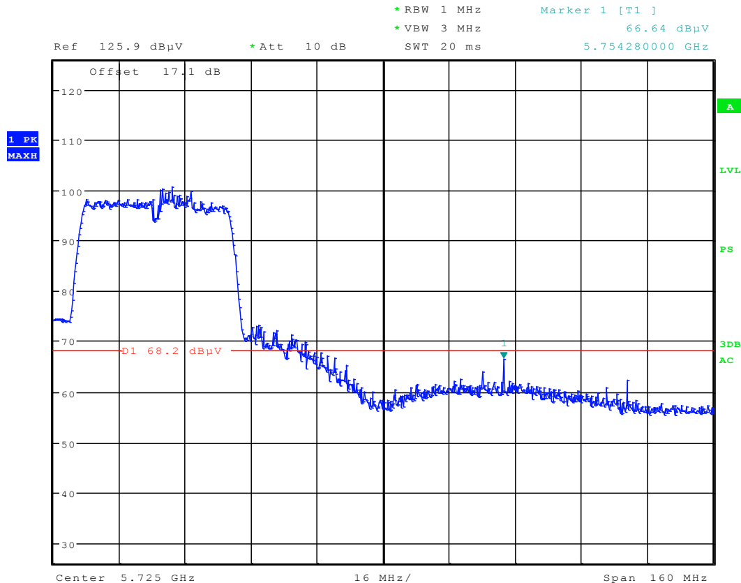
Plot 6-68. Radiated Upper Band Edge Plot (Peak – UNII Band 2C)
