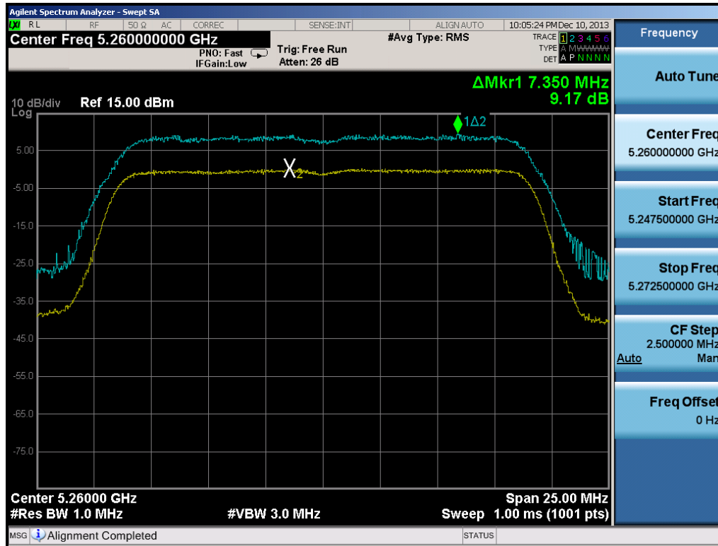
Plot 6-53. Peak Excursion Ratio Plot (20MHz BW 802.11n)
