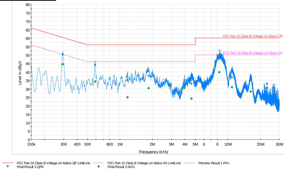
Plot 6-71. Line Conducted Plot with 802.11a UNII Band 2A (L1)
