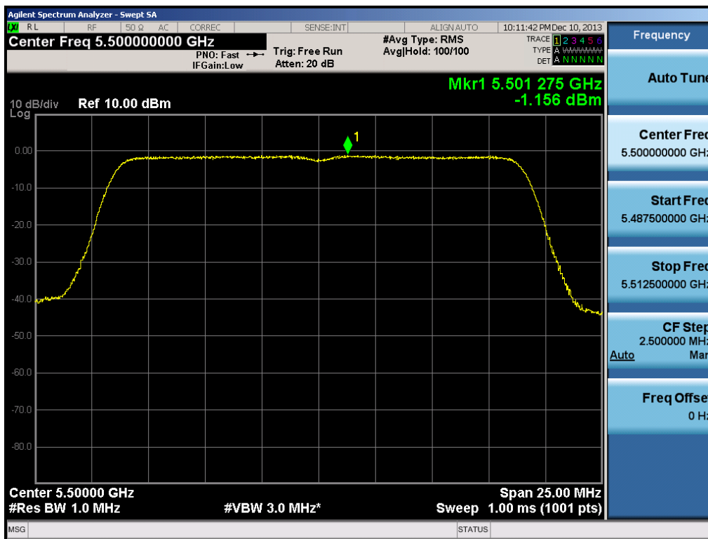
Plot 6-46. Peak Power Spectral Density Plot (20MHz BW 802.11n (UNII Band 2C) – Ch. 100)
