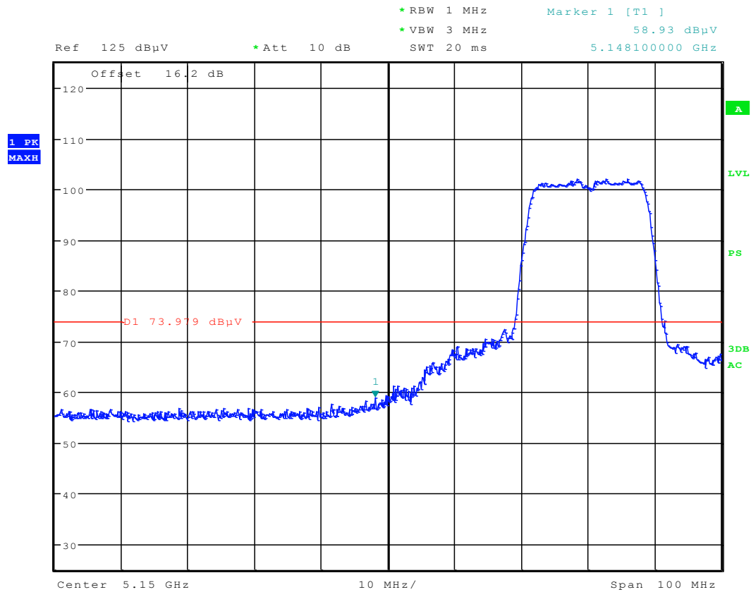
Plot 6-56. Radiated Restricted Lower Band Edge Plot (Peak – UNII Band 1)
