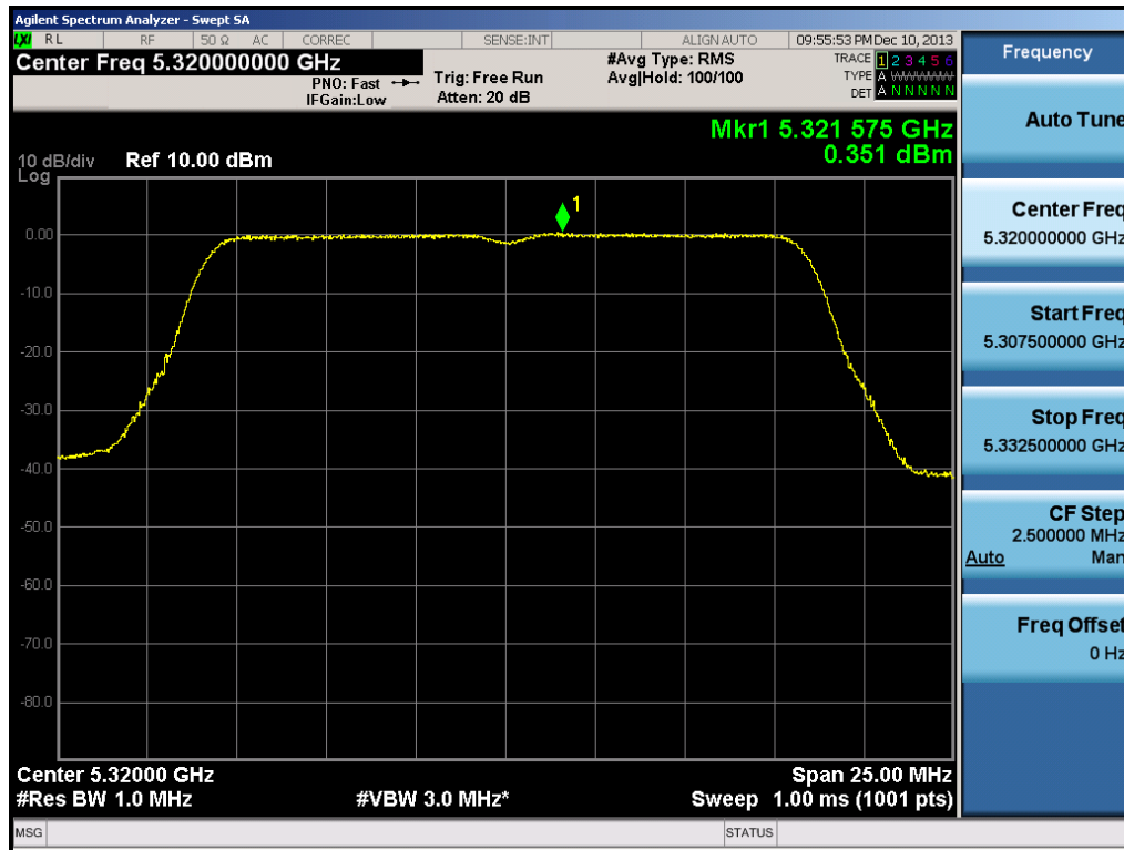
Plot 6-37. Peak Power Spectral Density Plot (802.11a (UNII Band 2A) – Ch. 64)
