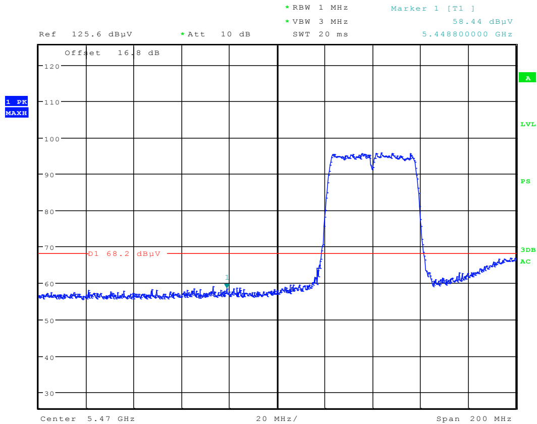
Plot 6-67. Radiated Restricted Lower Band Edge Plot (Peak – UNII Band 2C)
