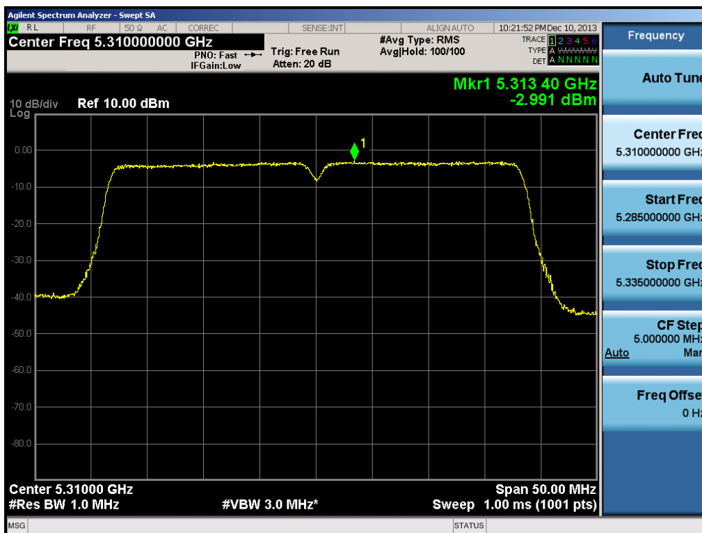
Plot 6-42. Peak Power Spectral Density Plot (40MHz BW 802.11n (UNII Band 2A) – Ch. 62)
