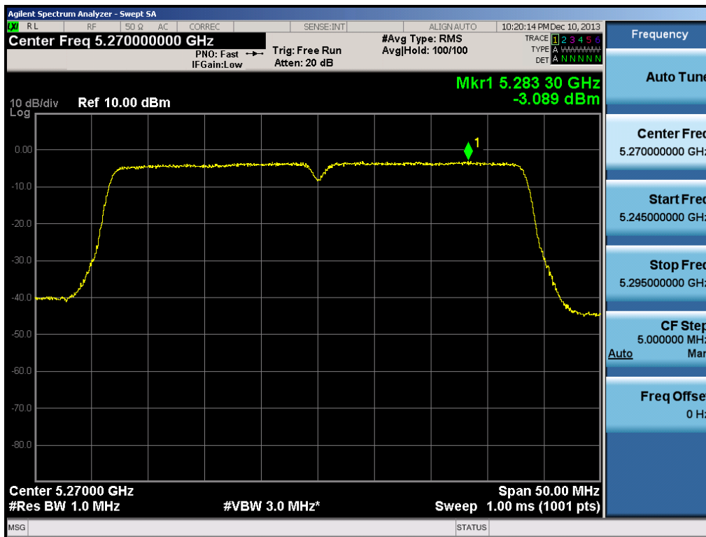
Plot 6-41. Peak Power Spectral Density Plot (40MHz BW 802.11n (UNII Band 2A) – Ch. 54)
