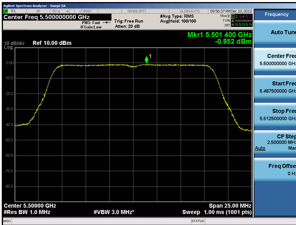
Plot 6-43. Peak Power Spectral Density Plot (802.11a (UNII Band 2C) – Ch. 100)
