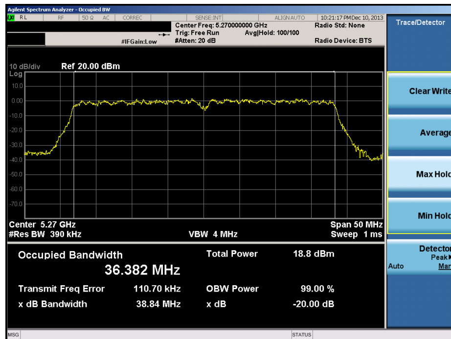
Plot 6-26. 20dB Bandwidth Plot (40MHz BW 802.11n (UNII Band 2A) – Ch. 54)
