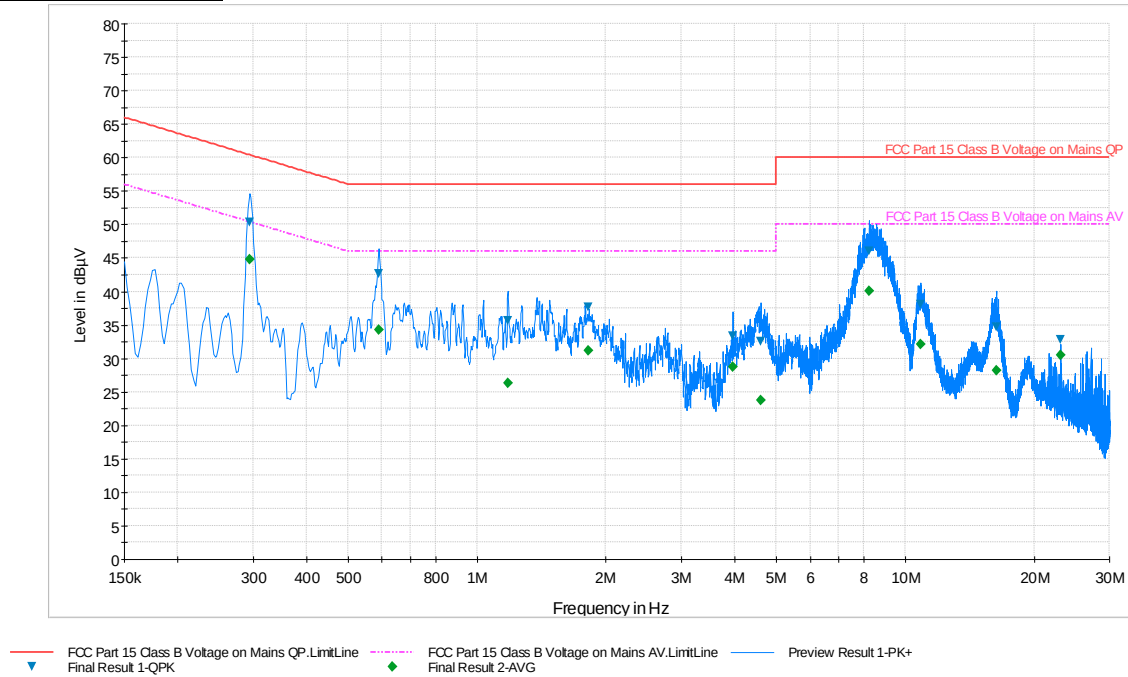
Plot 6-69. Line Conducted Plot with 802.11a UNII Band 1 (L1)
