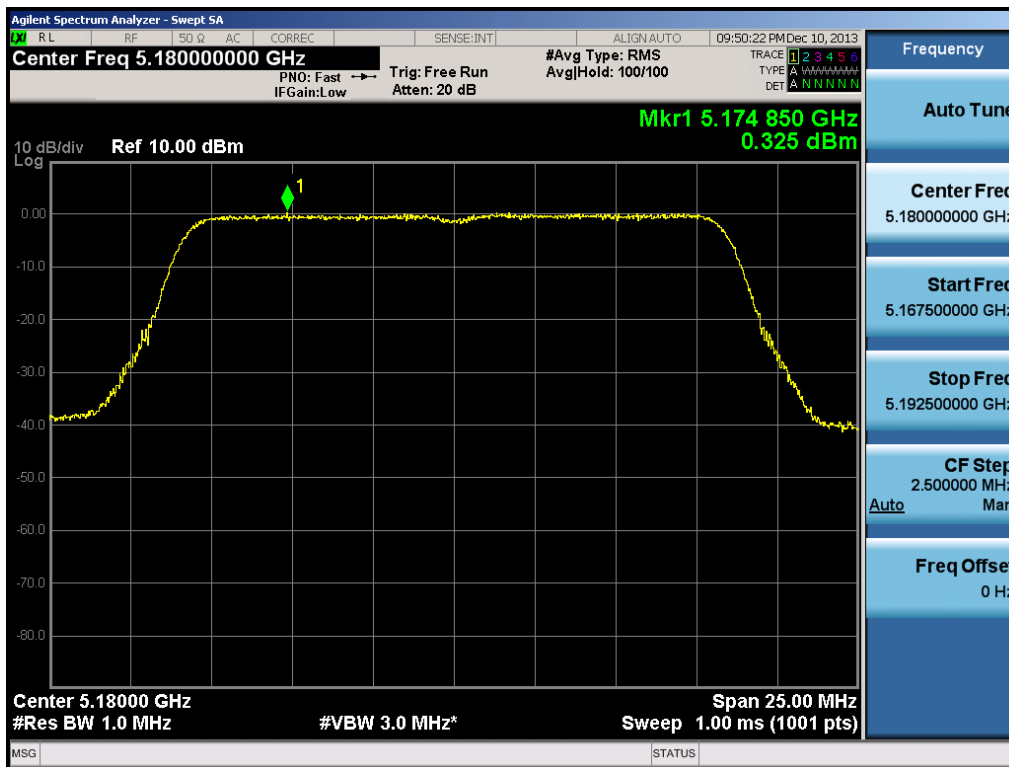
Plot 6-27. Peak Power Spectral Density Plot (802.11a (UNII Band 1) – Ch. 36)
