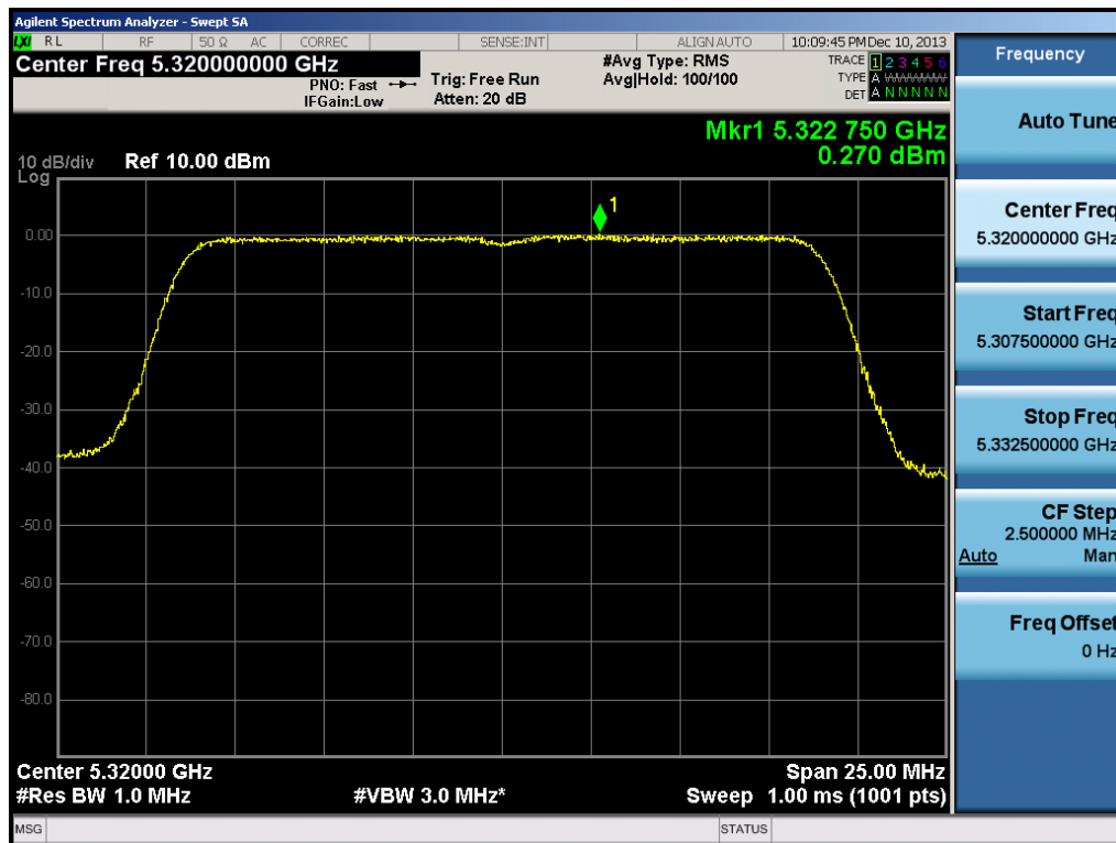
Plot 6-40. Peak Power Spectral Density Plot (20MHz BW 802.11n (UNII Band 2A) – Ch. 64)
