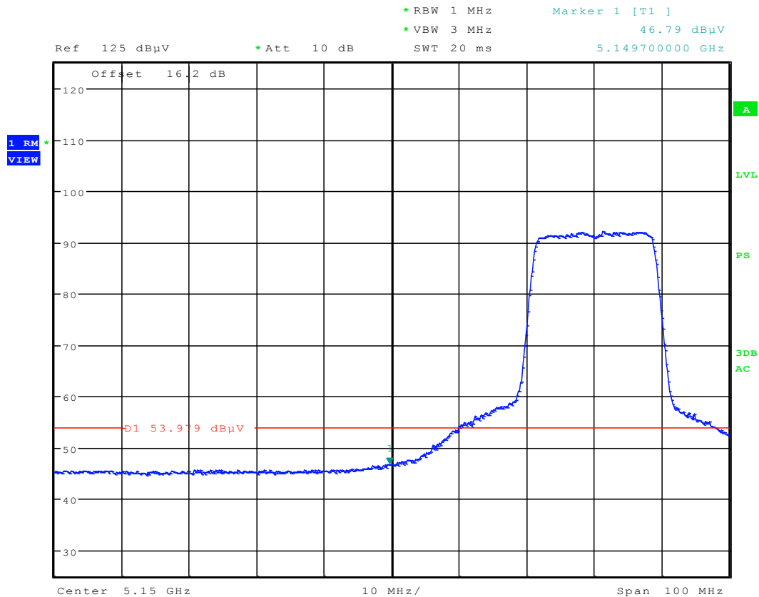
Plot 6-55. Radiated Restricted Lower Band Edge Plot (Average – UNII Band 1)
