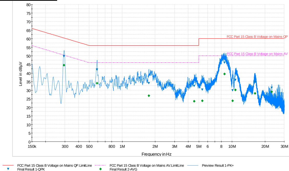
Plot 6-72. Line Conducted Plot with 802.11a UNII Band 2A (N)
