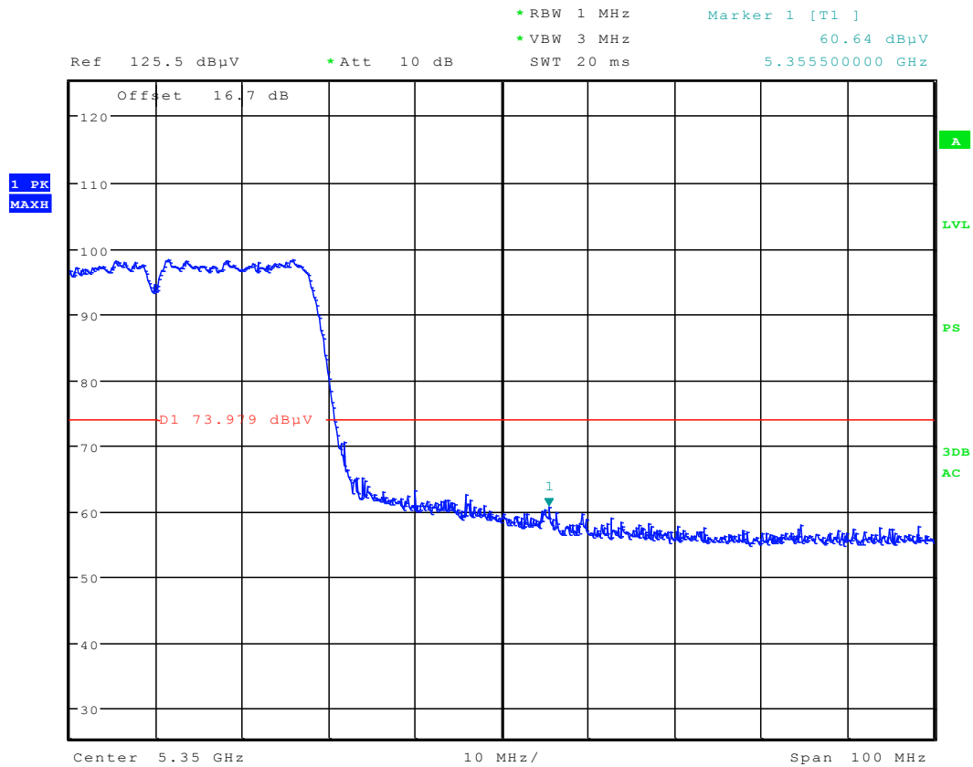
Plot 6-65. Radiated Restricted Upper Band Edge Plot (Peak – UNII Band 2A)
