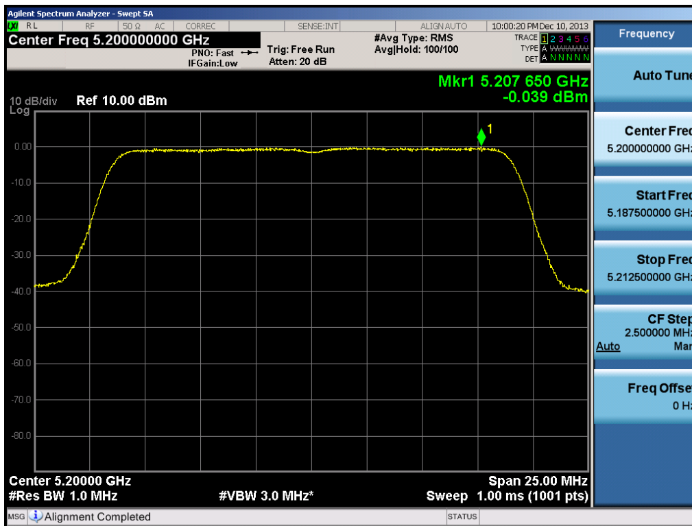
Plot 6-31. Peak Power Spectral Density Plot (20MHz BW 802.11n (UNII Band 1) – Ch. 40)
