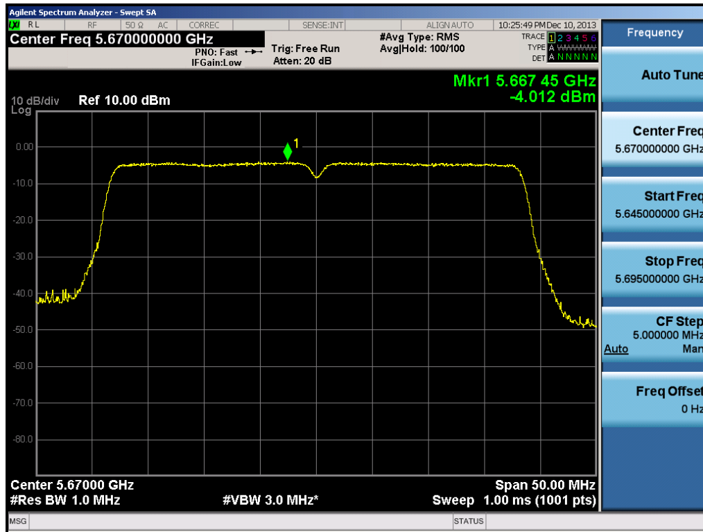
Plot 6-51. Peak Power Spectral Density Plot (40MHz BW 802.11n (UNII Band 2C) – Ch. 134)
