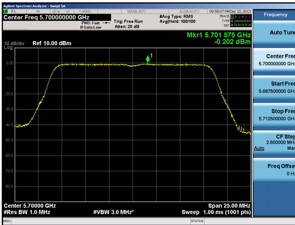
Plot 6-45. Peak Power Spectral Density Plot (802.11a (UNII Band 2C) – Ch. 140)
