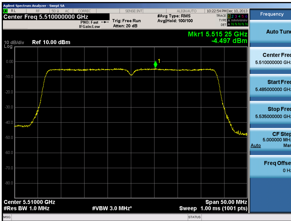
Plot 6-49. Peak Power Spectral Density Plot (40MHz BW 802.11n (UNII Band 2C) – Ch. 102)
