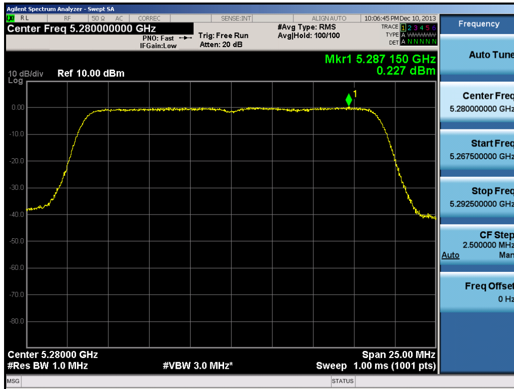
Plot 6-39. Peak Power Spectral Density Plot (20MHz BW 802.11n (UNII Band 2A) – Ch. 56)
