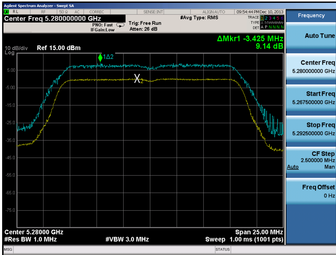
Plot 6-52. Peak Excursion Ratio Plot (802.11a)
