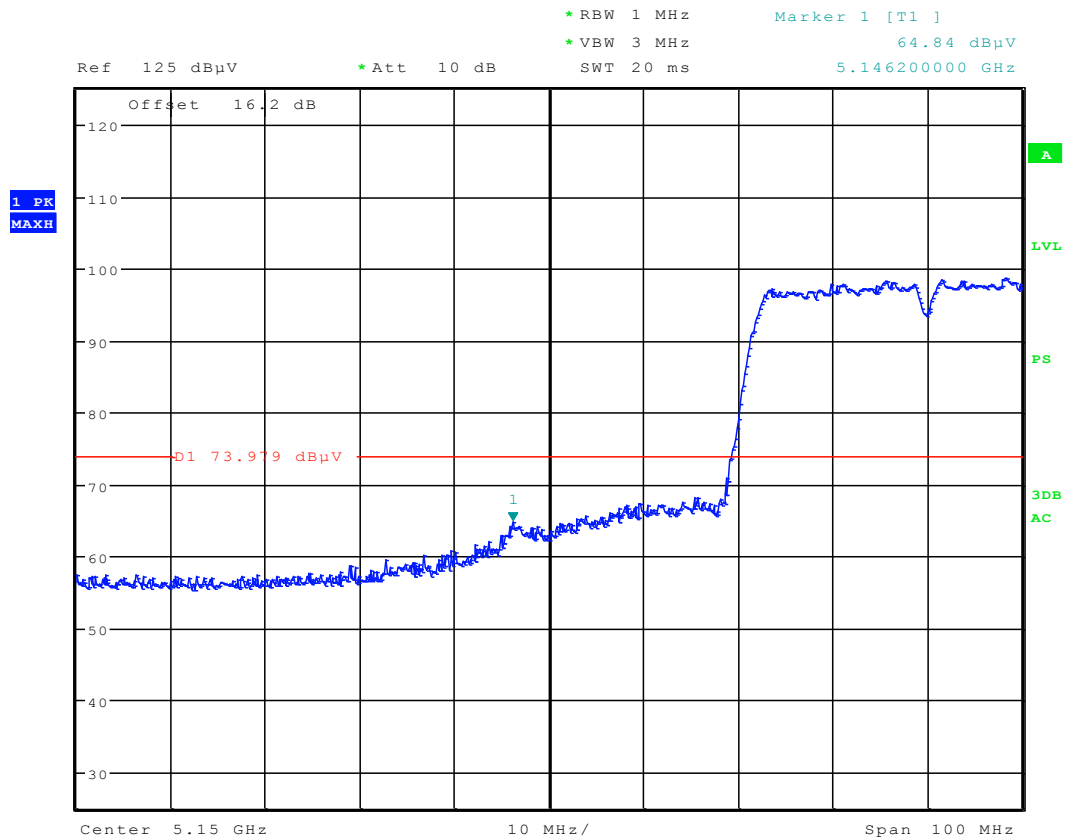
Plot 6-63. Radiated Restricted Lower Band Edge Plot (Peak – UNII Band 1)
