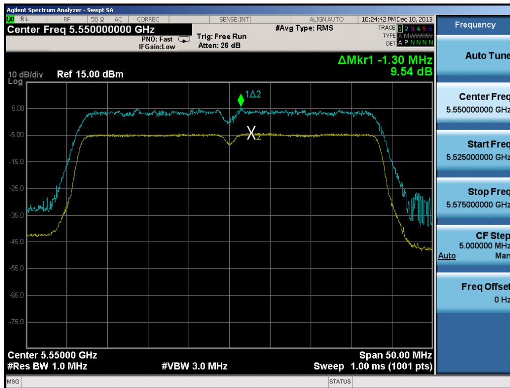
Plot 6-54. Peak Excursion Ratio Plot (40MHz BW 802.11n)
