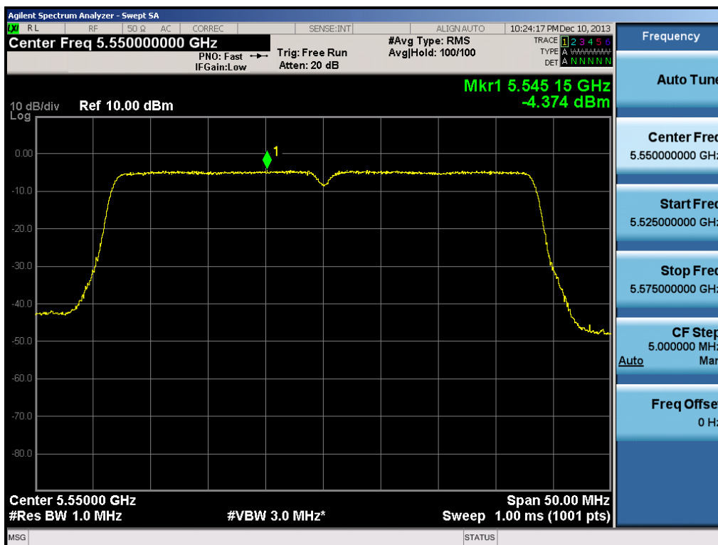
Plot 6-50. Peak Power Spectral Density Plot (40MHz BW 802.11n (UNII Band 2C) – Ch. 110)
