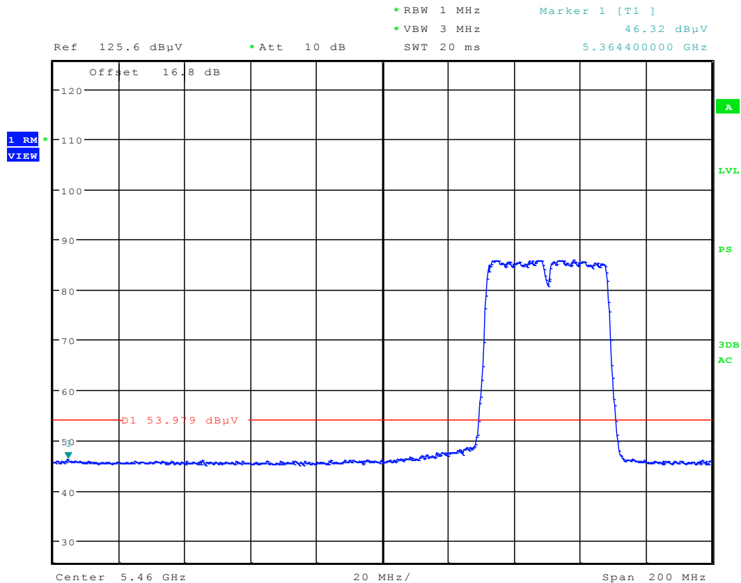
Plot 6-66. Radiated Restricted Lower Band Edge Plot (Average – UNII Band 2C)
