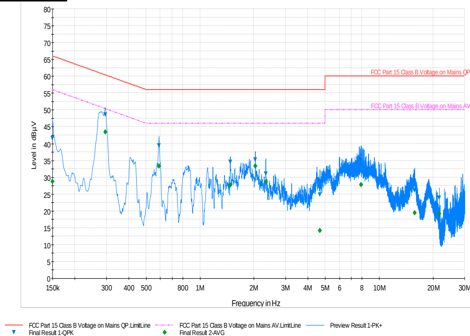
Plot 6-70. Line Conducted Plot with 802.11a UNII Band 1 (N)
