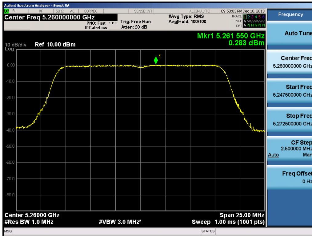
Plot 6-35. Peak Power Spectral Density Plot (802.11a (UNII Band 2A) – Ch. 52)
