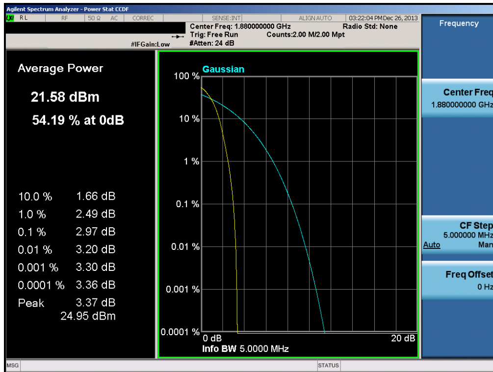
Plot 6-43. Peak-Average Ratio Plot (PCS WCDMA Mode – Ch. 9400)
