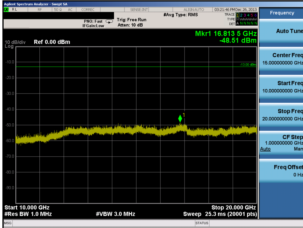
Plot 6-29. Conducted Spurious Plot (PCS WCDMA Mode – Ch. 9400)
