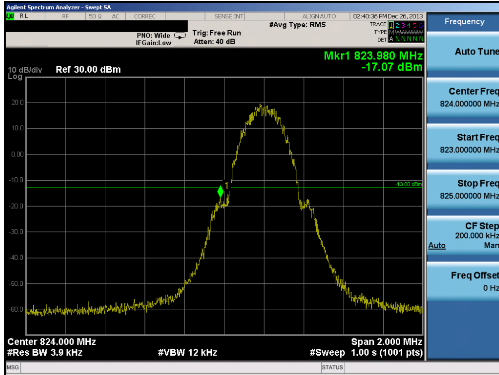
Plot 6-32. Band Edge Plot (Cellular GSM Mode – Ch. 128)
