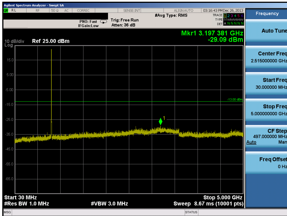
Plot 6-20. Conducted Spurious Plot (Cellular WCDMA Mode – Ch. 4132)
