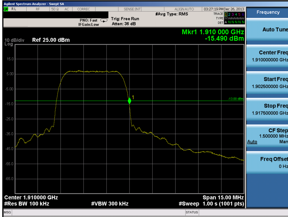
Plot 6-40. Band Edge Plot (PCS WCDMA Mode – Ch. 9538)
