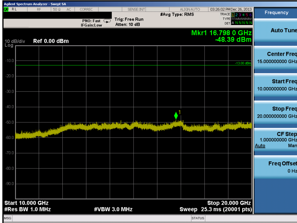
Plot 6-27. Conducted Spurious Plot (PCS WCDMA Mode – Ch. 9262)
