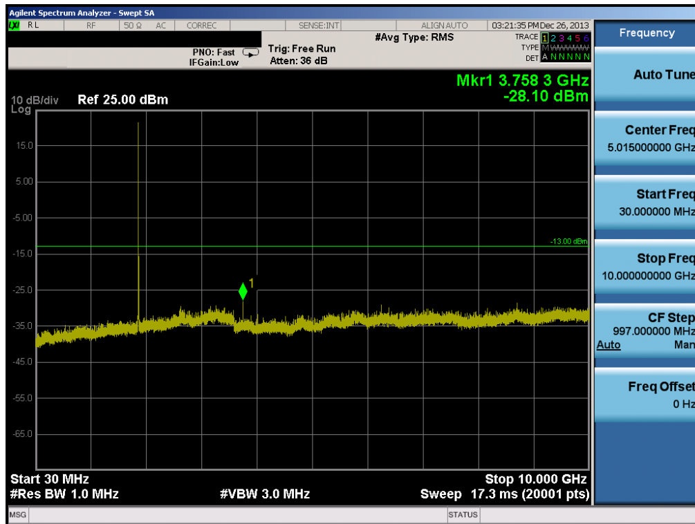
Plot 6-28. Conducted Spurious Plot (PCS WCDMA Mode – Ch. 9400)
