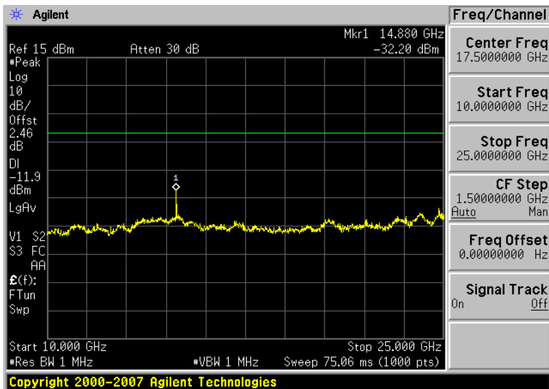
Plot 6-17. Conducted Spurious Plot (Bluetooth, 1Mbps – Ch. 0)
