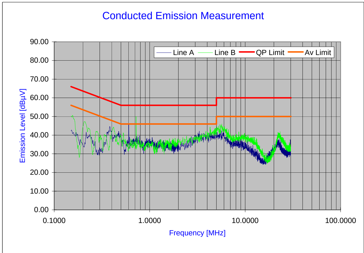
Plot 6-22. Line Conducted Plot with Bluetooth
