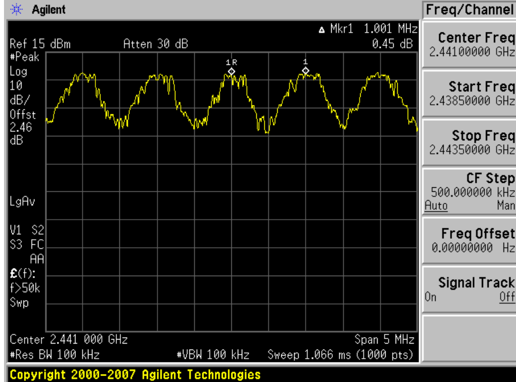
Plot 6-12. Channel Spacing Plot (Bluetooth)
