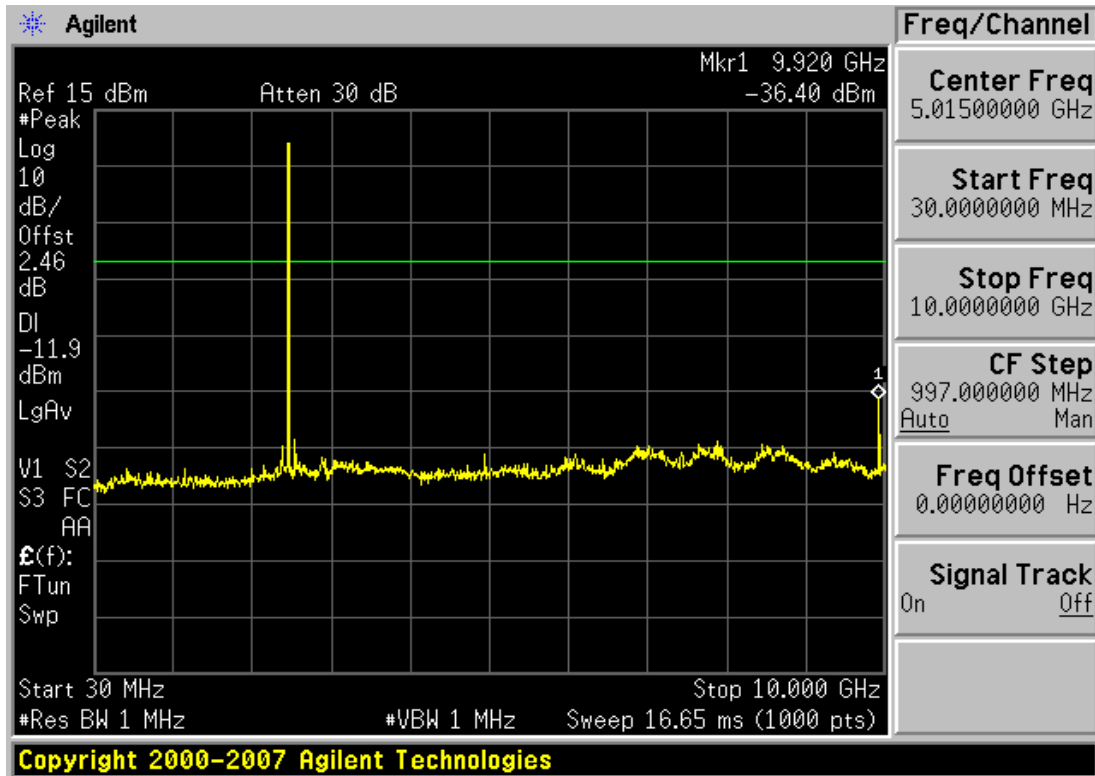
Plot 6-16. Conducted Spurious Plot (Bluetooth, 1Mbps – Ch. 0)
