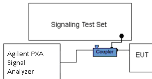
Figure 6-3. Test Instrument & Measurement Setup
