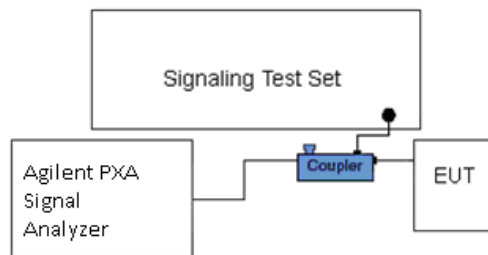
Figure 6-4. Test Instrument & Measurement Setup
