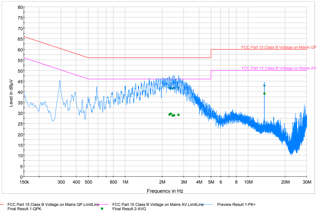
Plot 8-2. Line-Conducted Test Plot (N)
