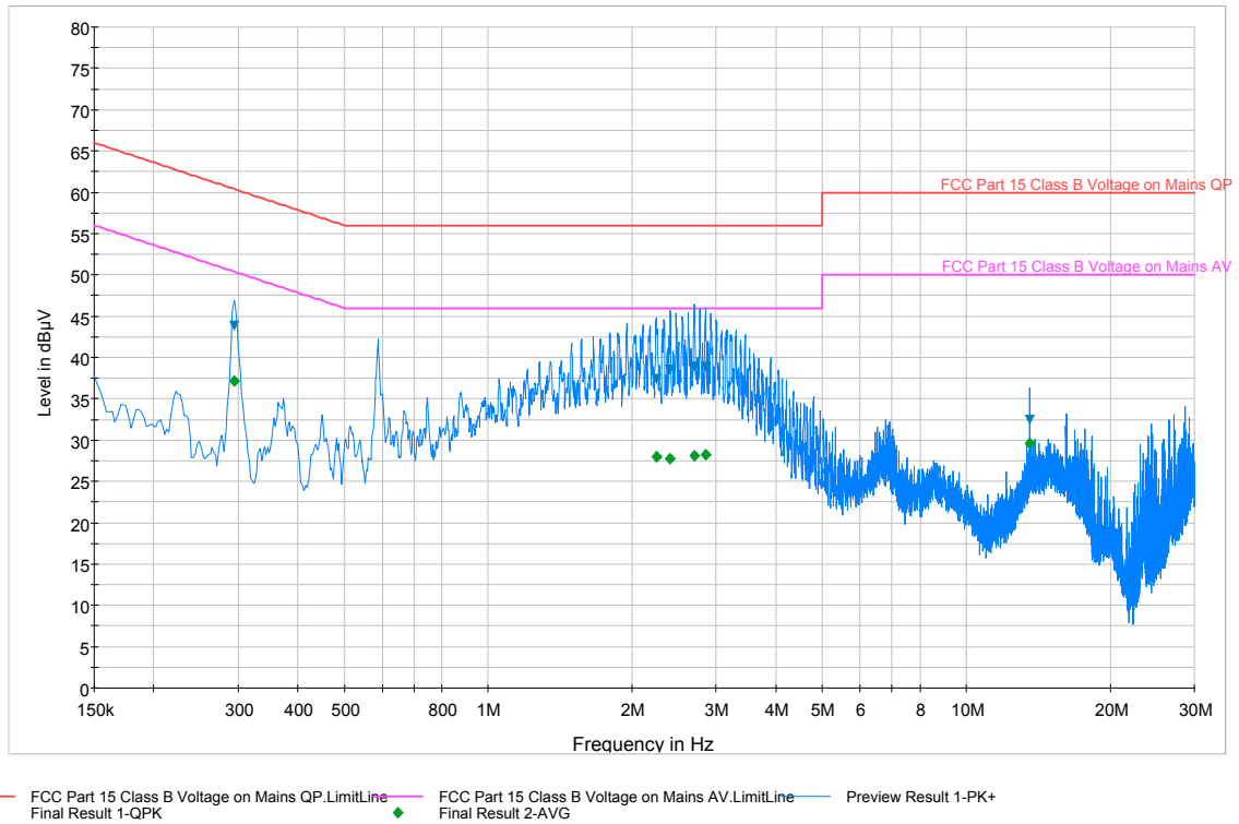
Plot 8-1. Line-Conducted Test Plot (L1)
