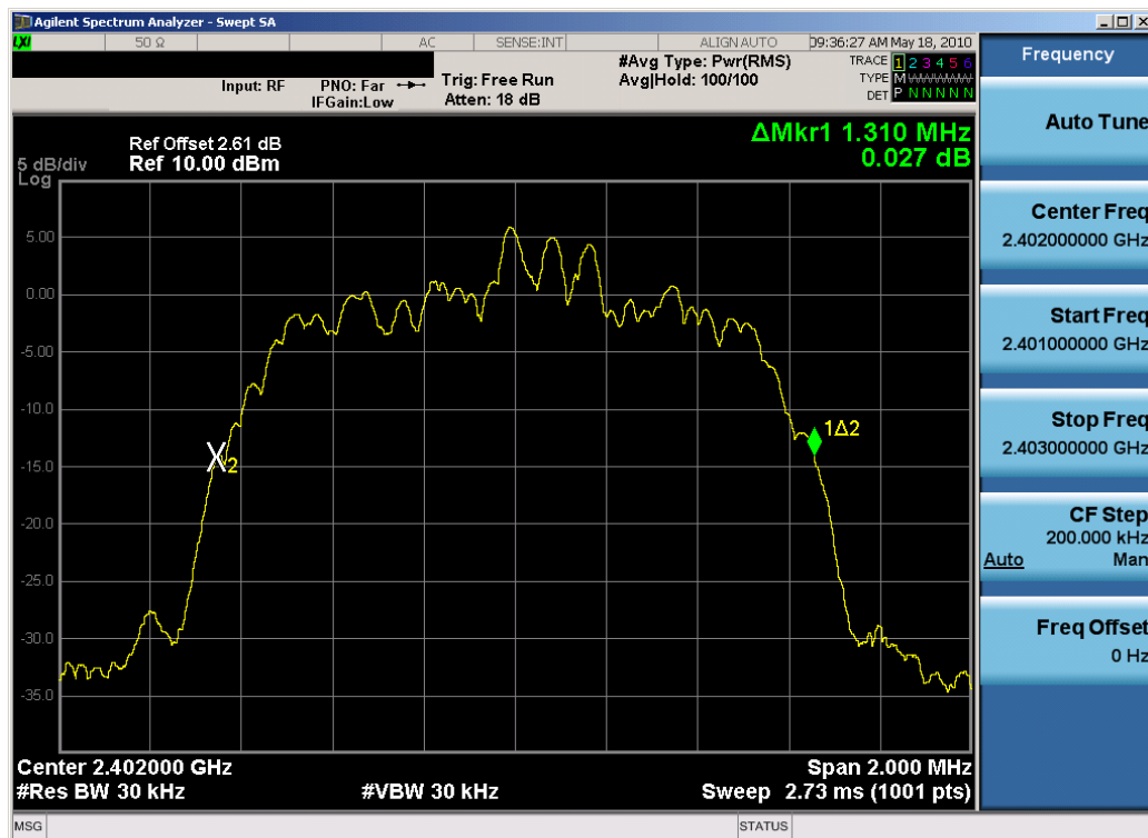
Plot 6-1. 20dB Bandwidth Plot (Ch. 0)
