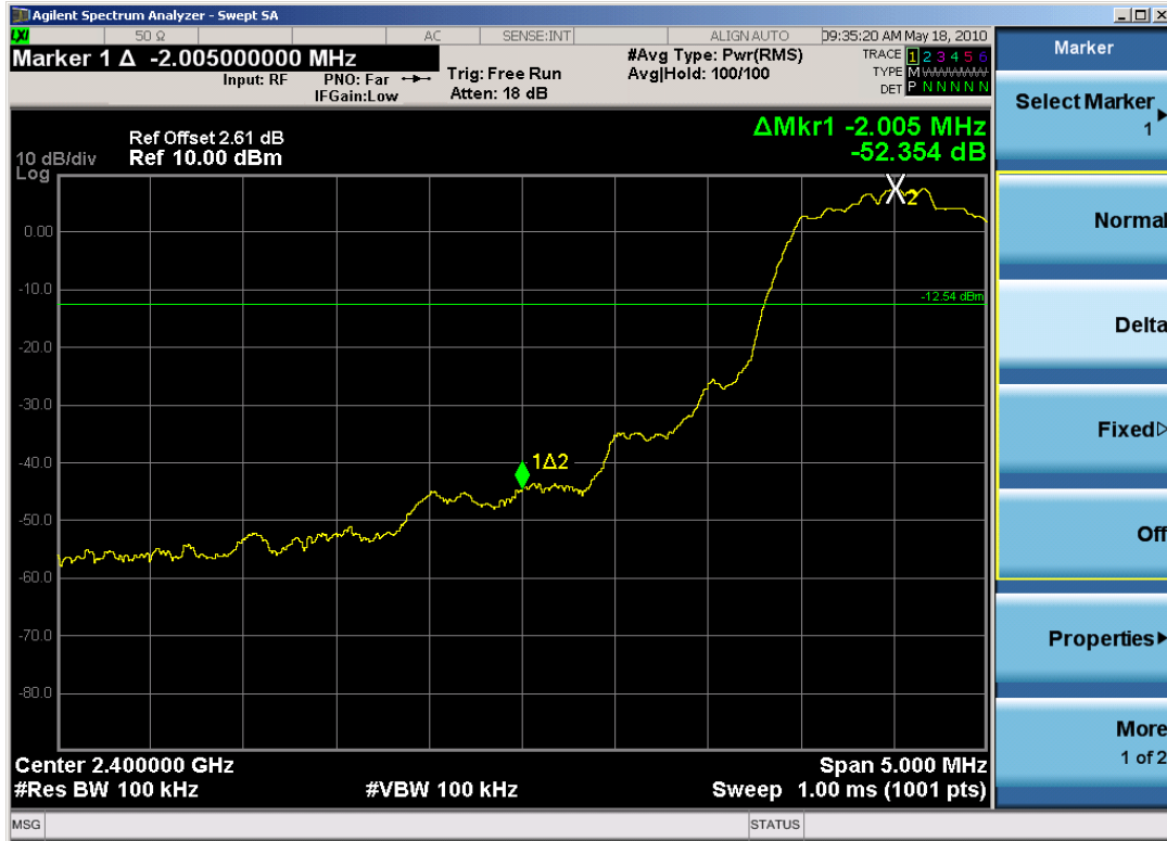
Plot 6-6. Band Edge Plot (Ch. 0)
