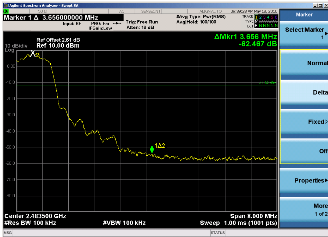
Plot 6-7. Band Edge Plot (Ch. 78)
