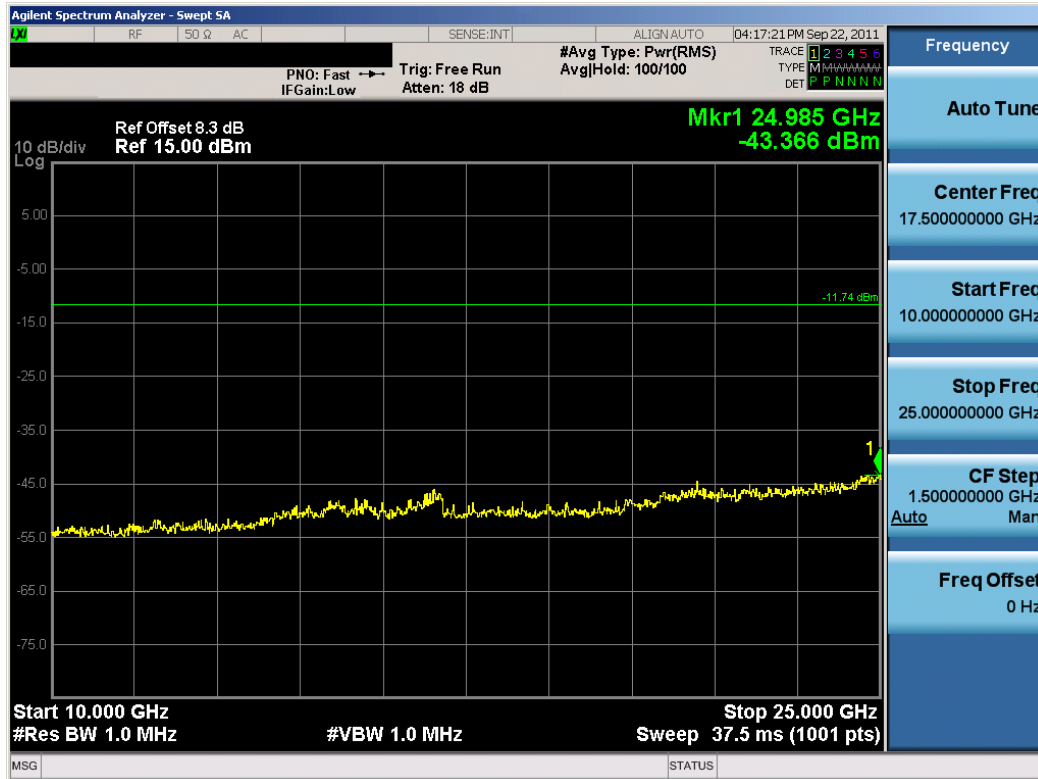
Plot 6-19. Conducted Spurious Plot (Bluetooth, 3Mbps – Ch. 39)
