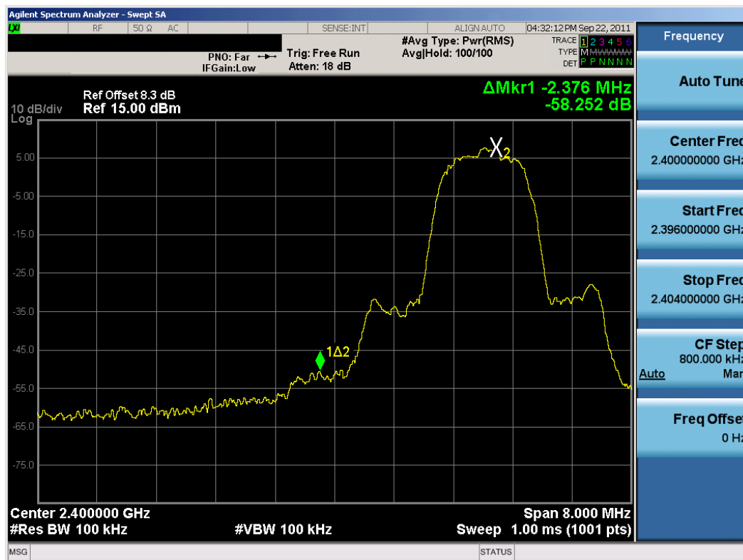
Plot 6-10. Band Edge Plot (Bluetooth, 3Mbps – Ch. 0)
