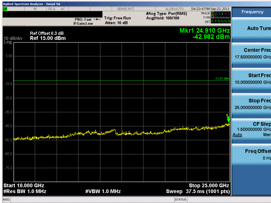
Plot 6-21. Conducted Spurious Plot (Bluetooth, 3Mbps – Ch. 78)
