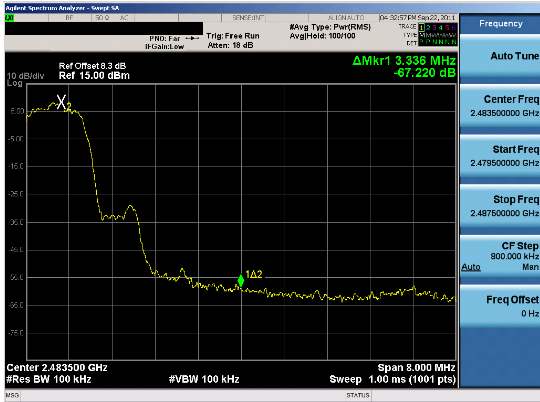
Plot 6-11. Band Edge Plot (Bluetooth, 3Mbps – Ch. 78)
