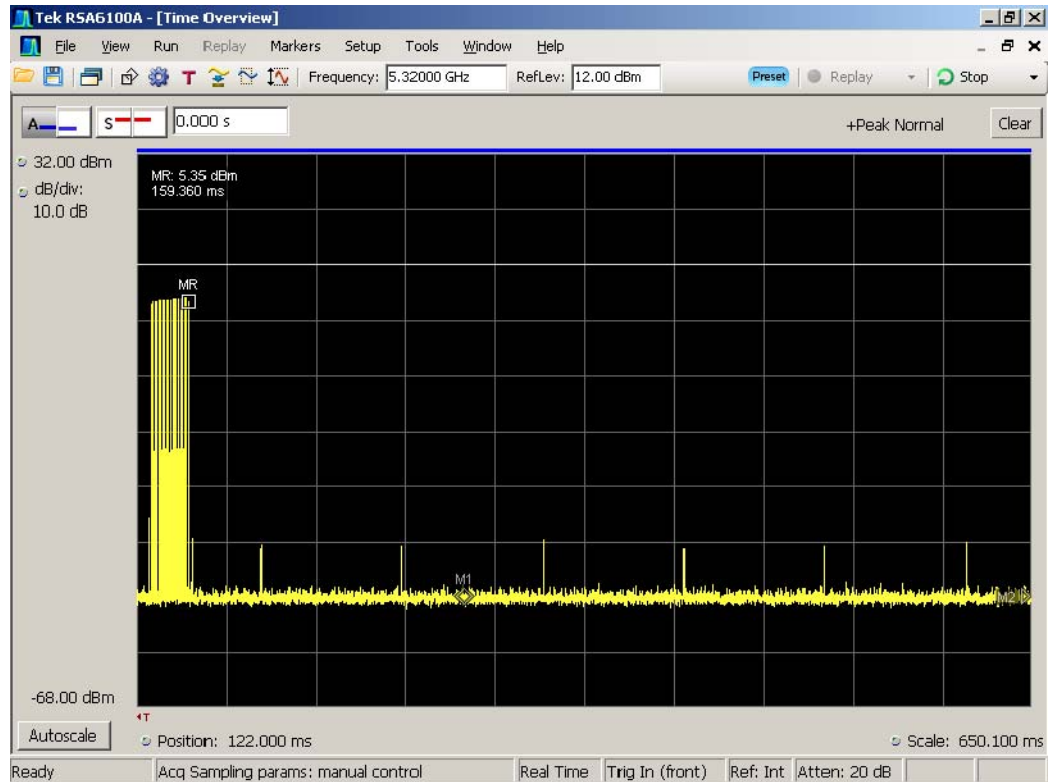
Figure 5-5. Channel Move Time (Zoomed In)
