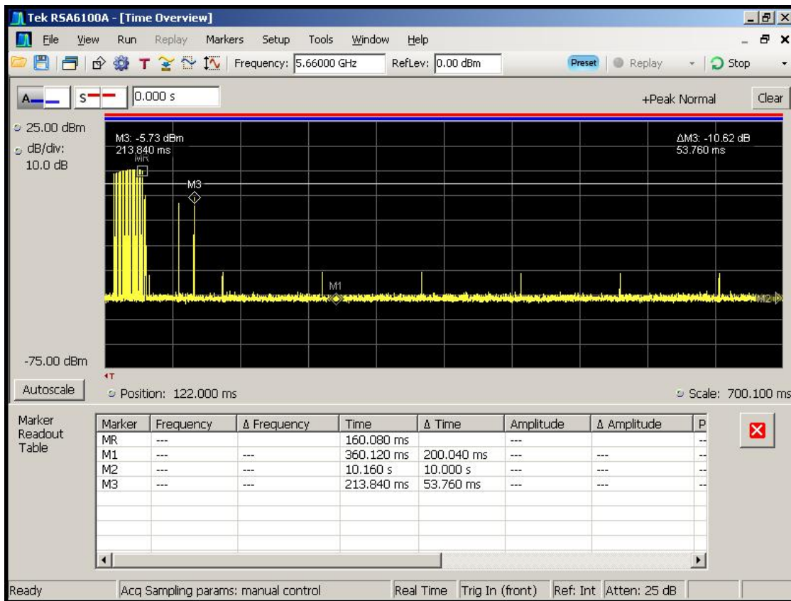
Figure 6-5. Channel Move Time (Zoomed In)
