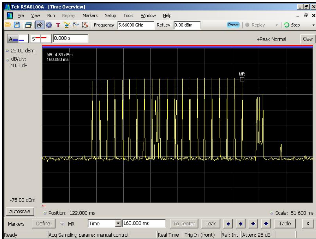
Figure 6-6-1. Type 1 Radar Pulse
