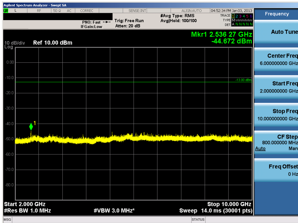
Plot 7-37. Conducted Spurious Plot (Cellular WCDMA Mode – Ch. 4233)
