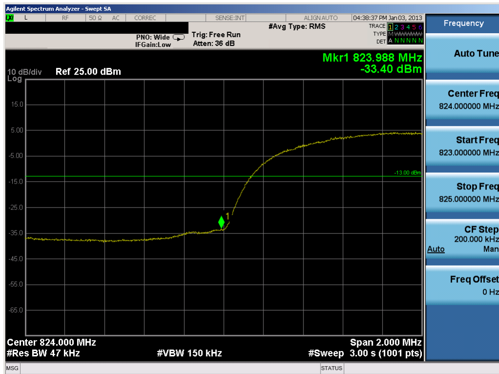
Plot 7-29. Band Edge Plot (Cellular WCDMA Mode – Ch. 4132)
