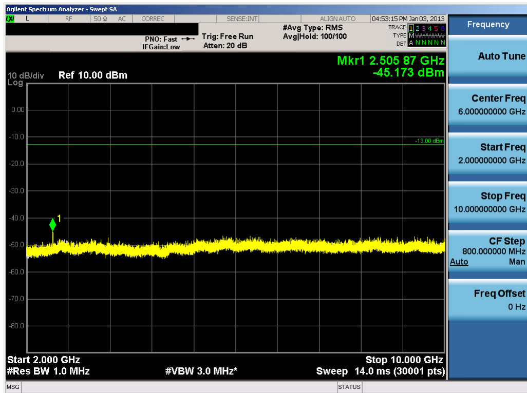
Plot 7-33. Conducted Spurious Plot (Cellular WCDMA Mode – Ch. 4183)
