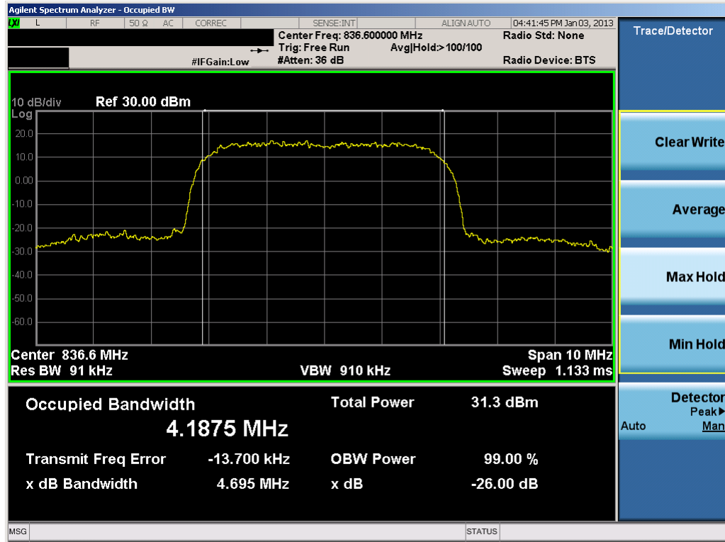
Plot 7-34. Occupied Bandwidth Plot (Cellular WCDMA Mode – Ch. 4183)
