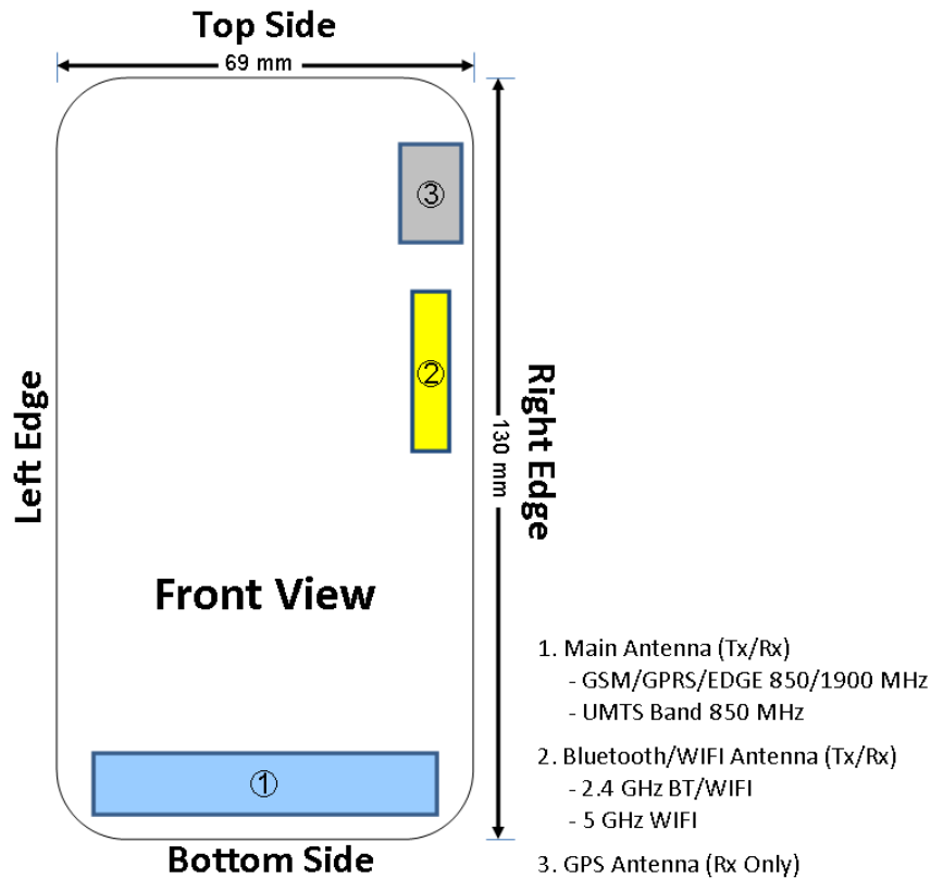
Figure 1-1 DUT Antenna Locations
