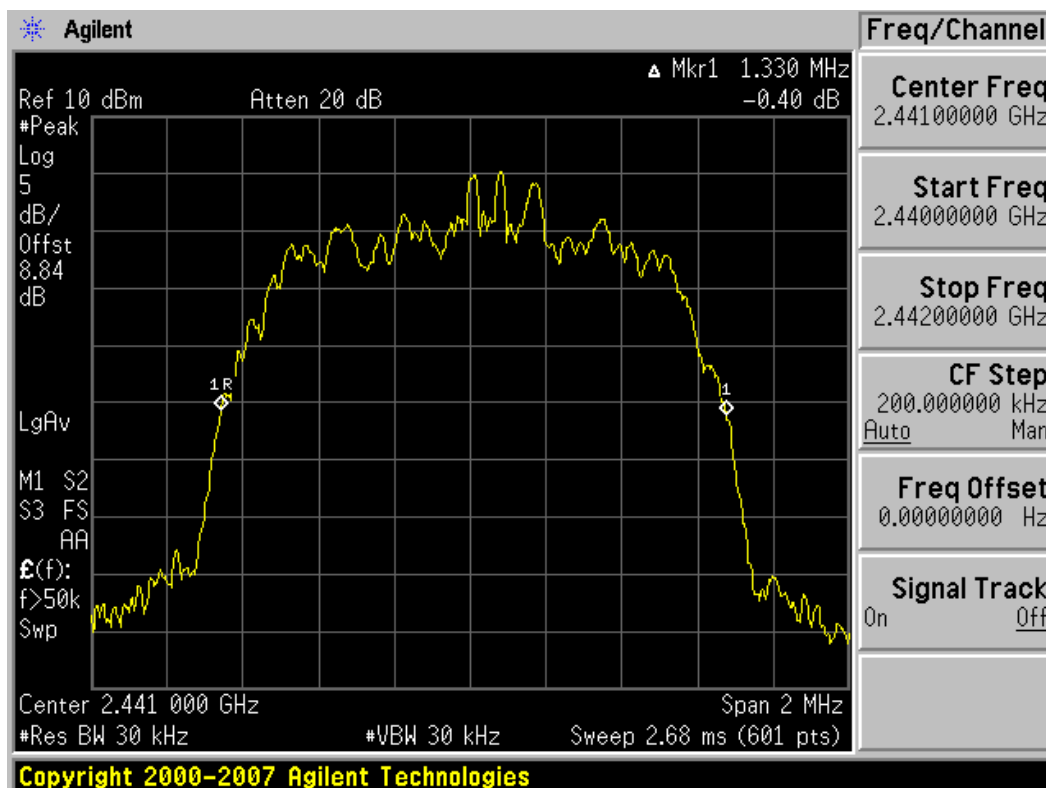
Plot 6-2. 20dB Bandwidth Plot (Bluetooth version 3.0 with enhanced data rates – Ch. 39)
