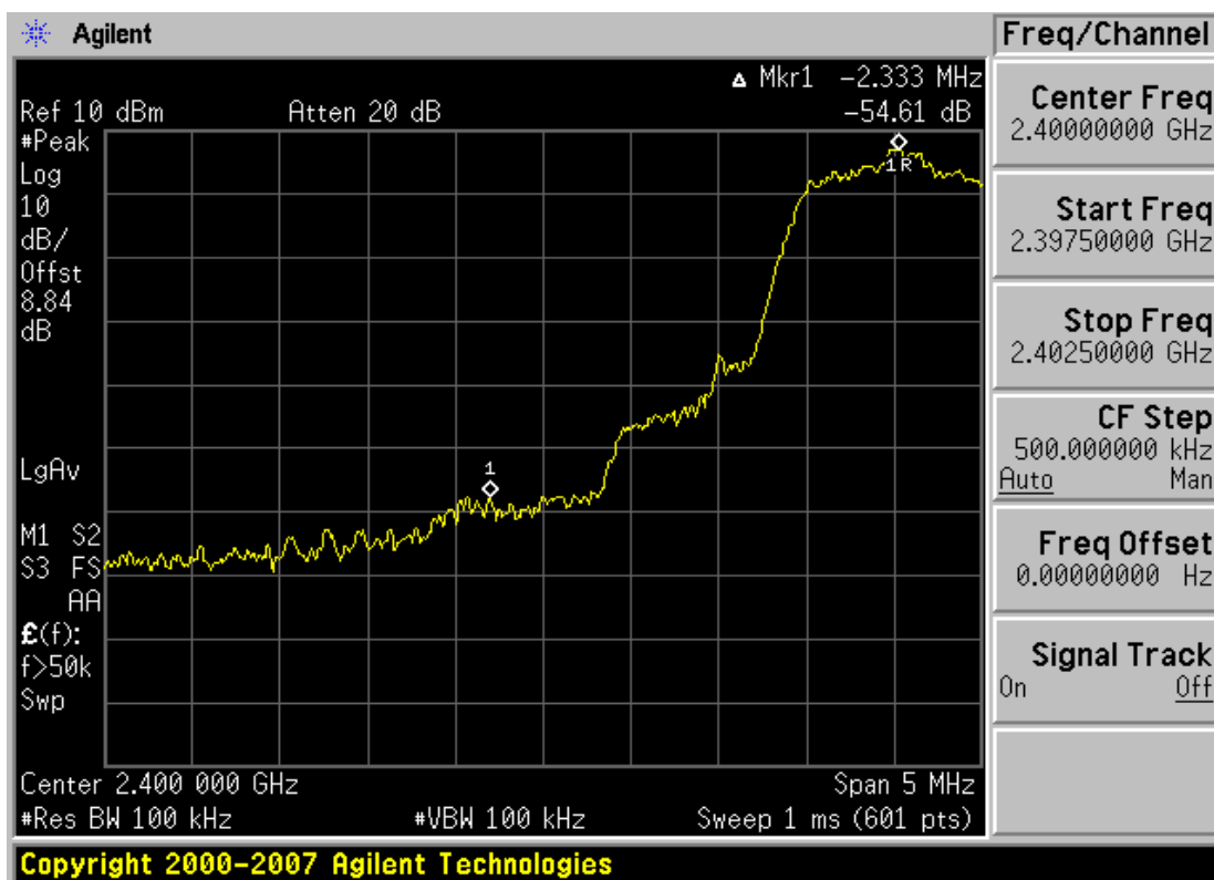
Plot 6-6. Band Edge Plot (Bluetooth version 3.0 with enhanced data rates – Ch. 0)
