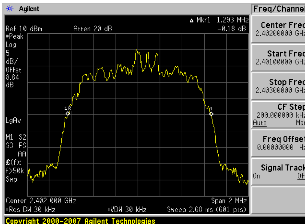
Plot 6-1. 20dB Bandwidth Plot (Bluetooth version 3.0 with enhanced data rates – Ch. 0)
