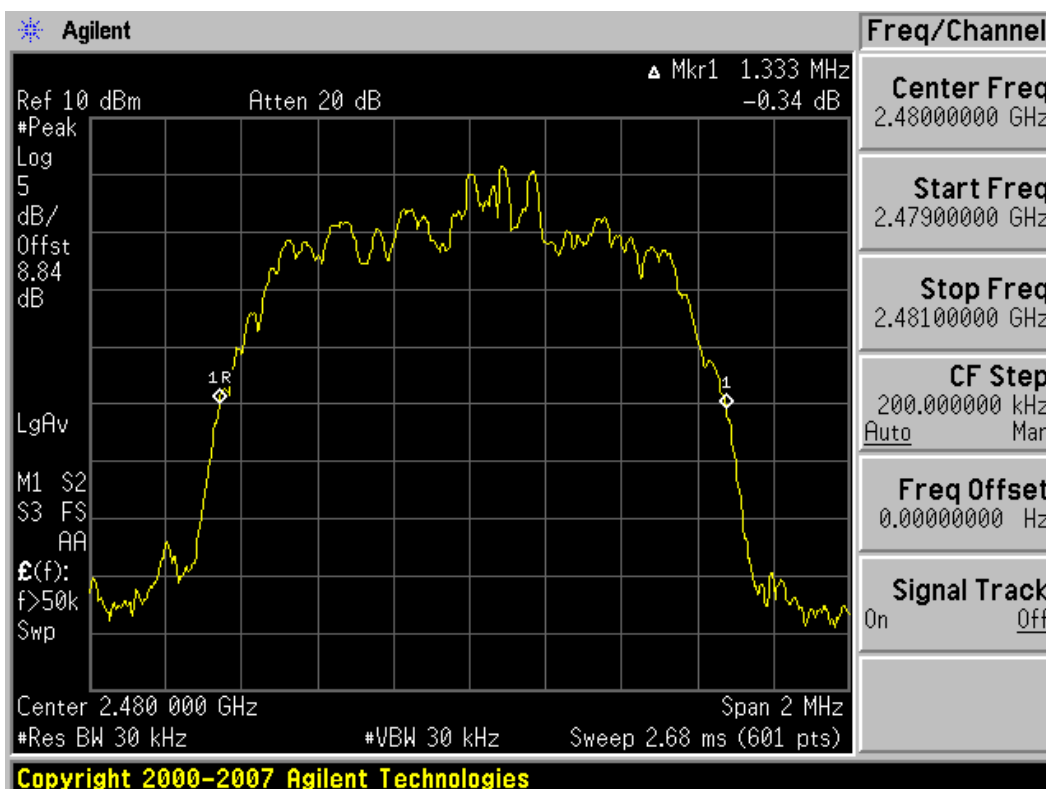
Plot 6-3. 20dB Bandwidth Plot (Bluetooth version 3.0 with enhanced data rates – Ch. 78)
