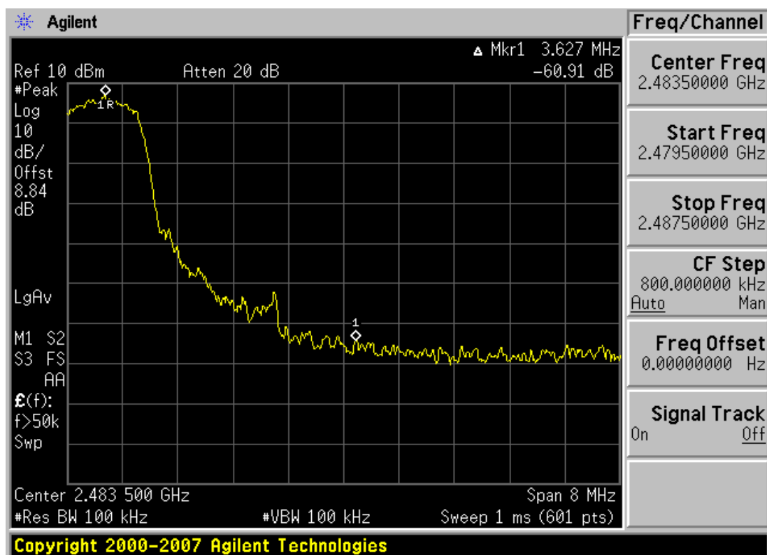
Plot 6-7. Band Edge Plot (Bluetooth version 3.0 with enhanced data rates – Ch. 78)
