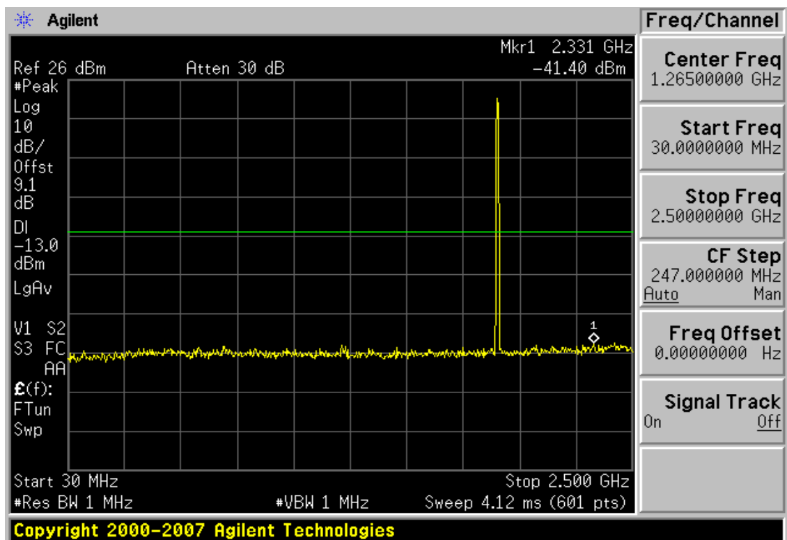
Plot 7-31. Conducted Spurious Plot (PCS WCDMA Mode – Ch. 9538)
