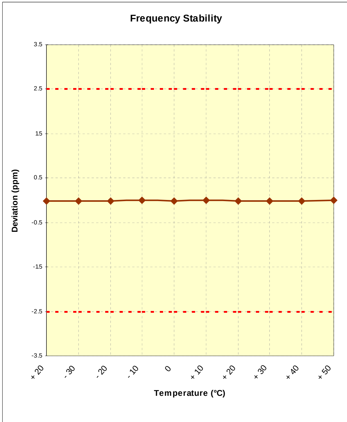
Figure 6-3. Frequency Stability Graph (PCS WCDMA Mode – Ch. 9400)
