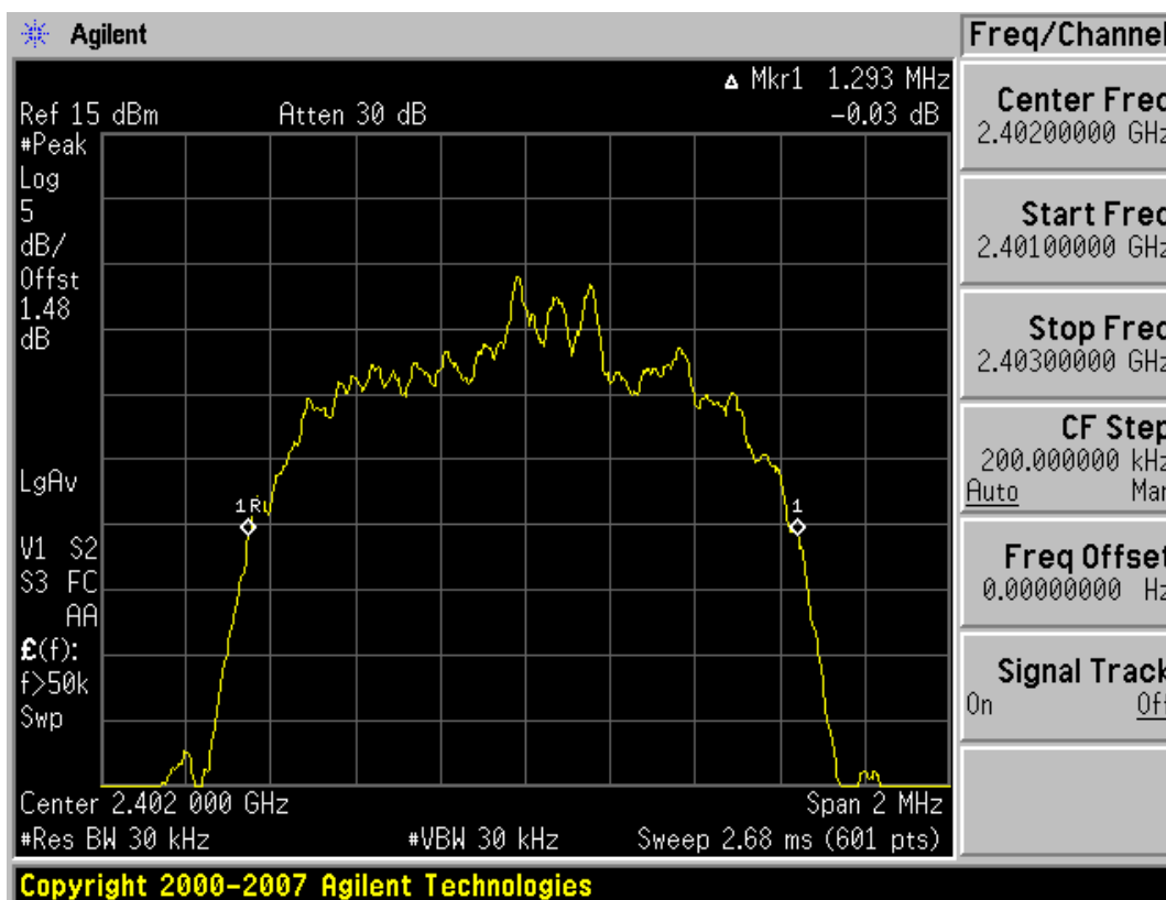
Plot 6-7. 20dB Bandwidth Plot (Bluetooth, 3Mbps – Ch. 0)
